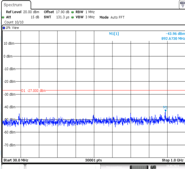
11AC20MIMO-Ant1-5720-30~1000-PASS
