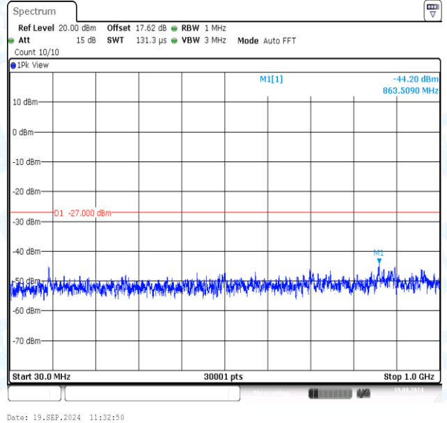
11AC80MIMO-Ant2-5530-30~1000-PASS
