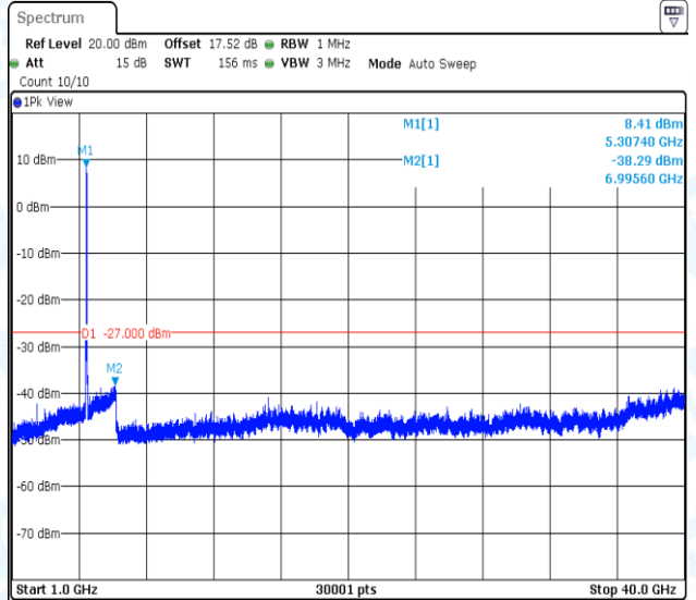
11AC40MIMO-Ant2-5310-1000~40000-PASS
