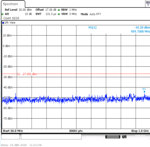
11AC80MIMO-Ant1-5530-30~1000-PASS
