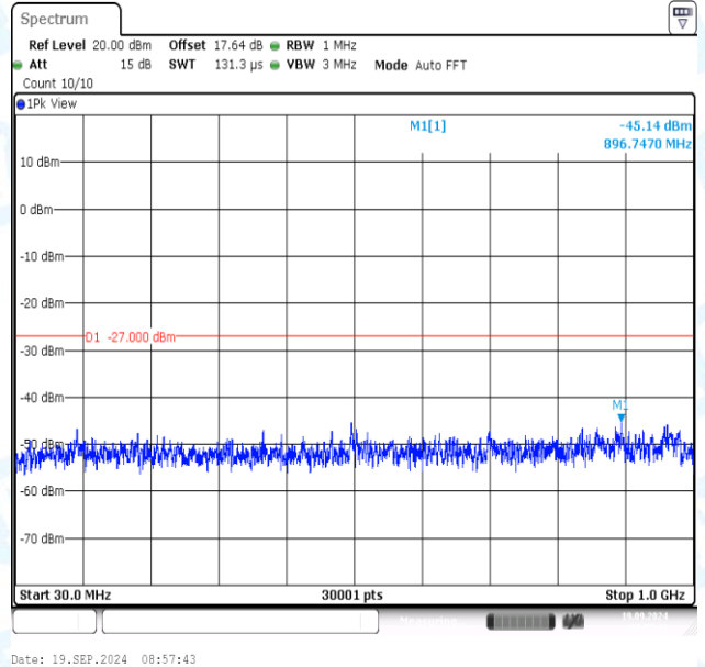
11AC20MIMO-Ant2-5500-30~1000-PASS
