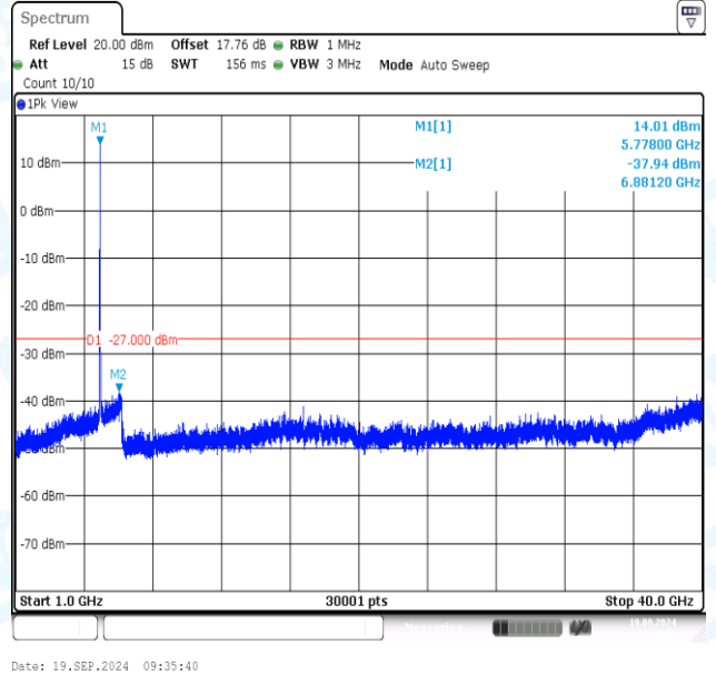
11AC20MIMO-Ant2-5785-1000~40000-PASS
