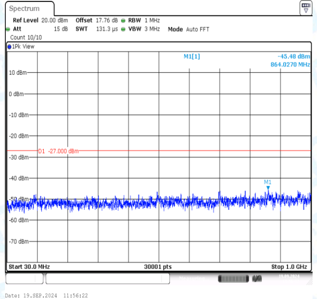
11AC80MIMO-Ant2-5775-30~1000-PASS
