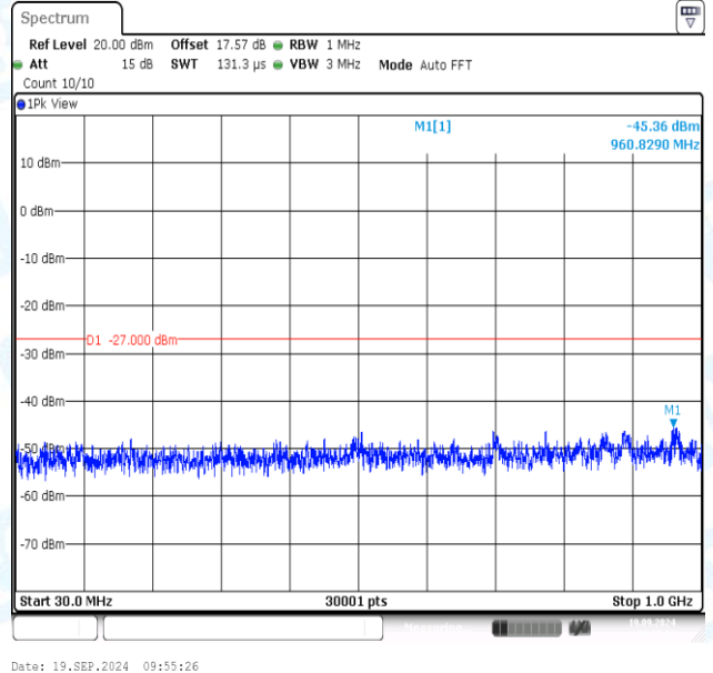
11AC40MIMO-Ant2-5230-30~1000-PASS
