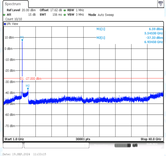
11AC80MIMO-Ant2-5530-1000~40000-PASS
