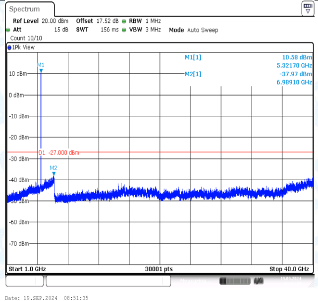
11AC20MIMO-Ant2-5320-1000~40000-PASS
