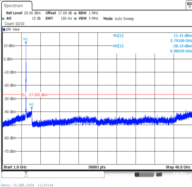
11AC40MIMO-Ant1-5795-1000~40000-PASS
