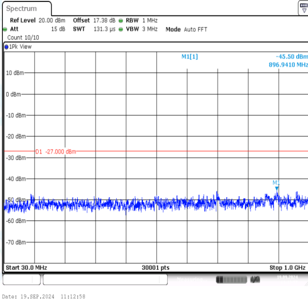
11AC80MIMO-Ant1-5210-30~1000-PASS
