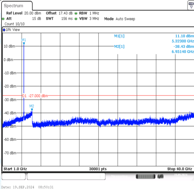
11AC20MIMO-Ant1-5320-1000~40000-PASS
