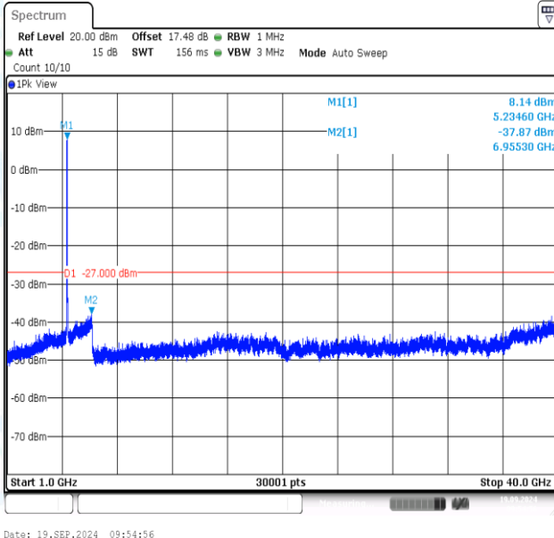
11AC40MIMO-Ant1-5230-1000~40000-PASS
