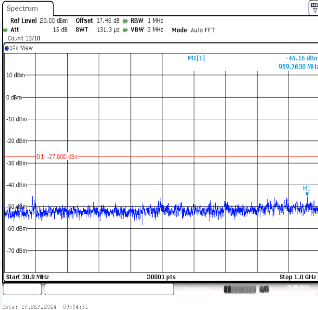
11AC40MIMO-Ant1-5230-30~1000-PASS
