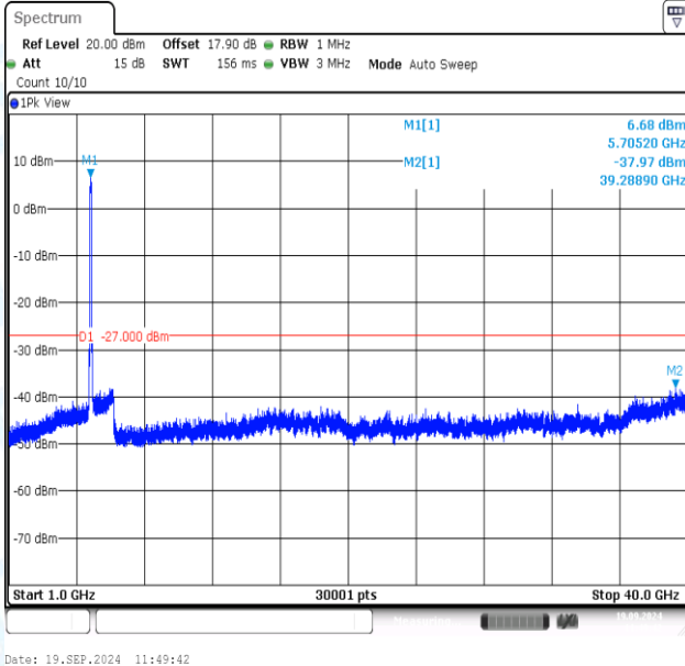
11AC80MIMO-Ant1-5690-1000~40000-PASS
