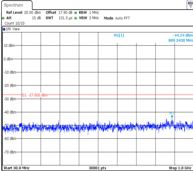
11AC40MIMO-Ant1-5710-30~1000-PASS
