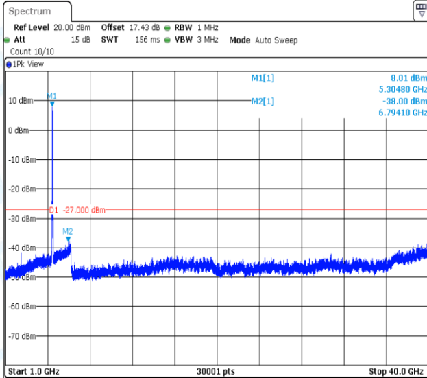
11AC40MIMO-Ant1-5310-1000~40000-PASS
