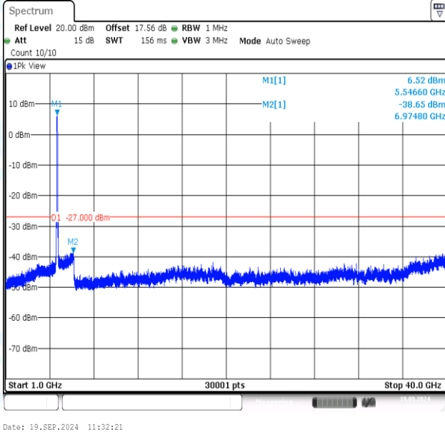
11AC80MIMO-Ant1-5530-1000~40000-PASS
