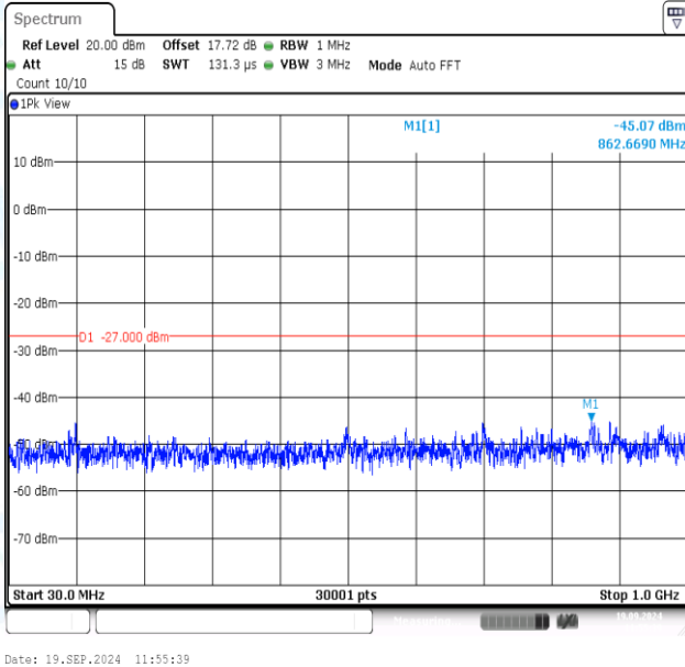
11AC80MIMO-Ant1-5775-30~1000-PASS
