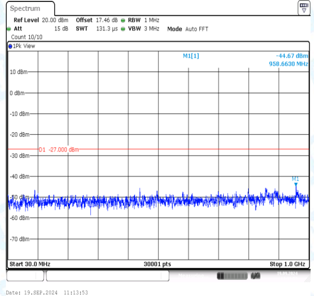
11AC80MIMO-Ant2-5210-30~1000-PASS
