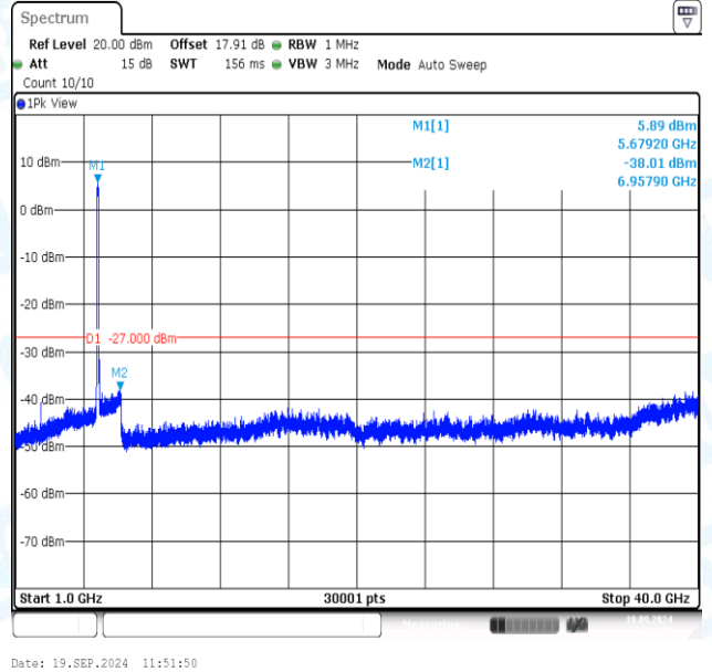
11AC80MIMO-Ant2-5690-1000~40000-PASS
