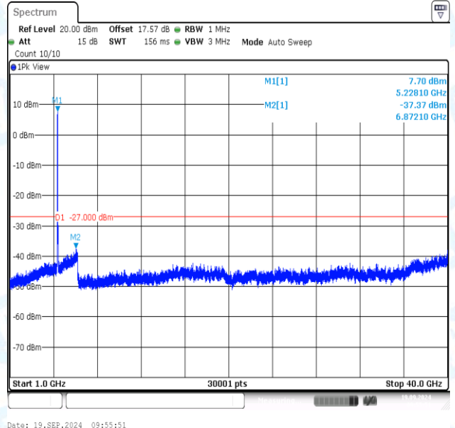
11AC40MIMO-Ant2-5230-1000~40000-PASS
