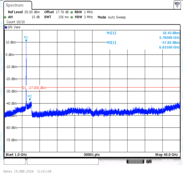
11AC40MIMO-Ant2-5795-1000~40000-PASS
