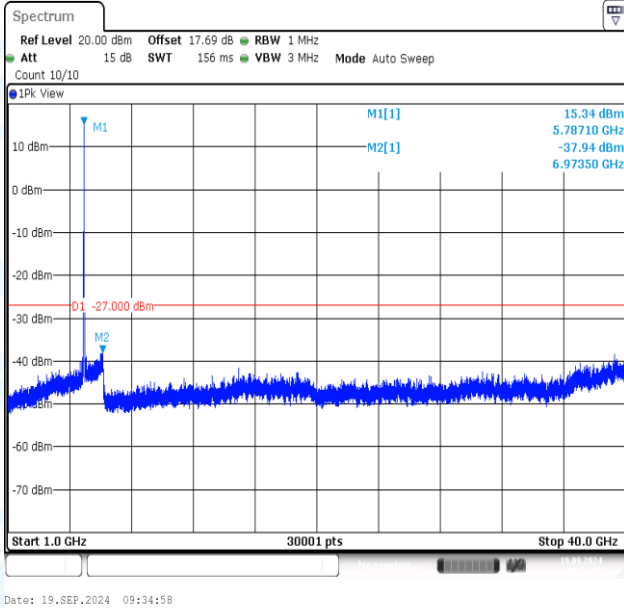
11AC20MIMO-Ant1-5785-1000~40000-PASS
