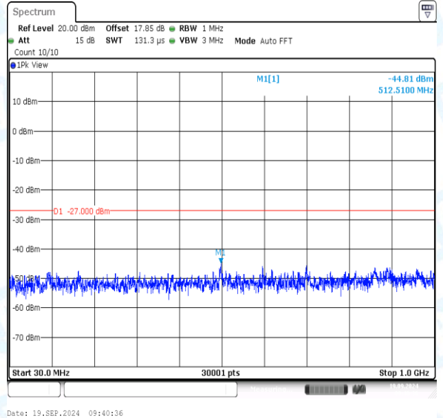
11AC20MIMO-Ant2-5825-30~1000-PASS
