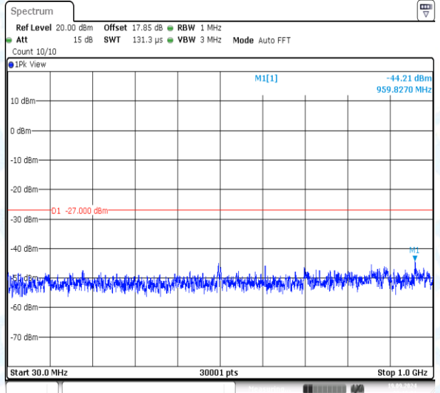
11AC20MIMO-Ant2-5720-30~1000-PASS
