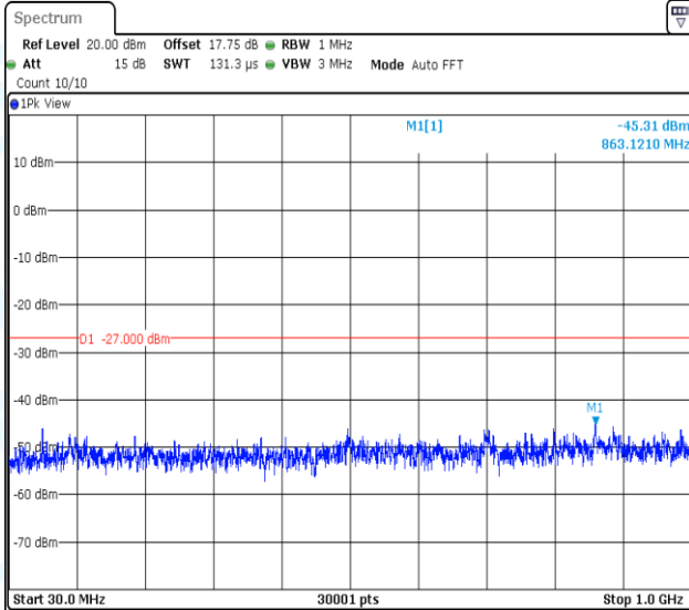
11N40MIMO-Ant1-5755-30~1000-PASS
