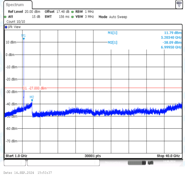
11N20MIMO-Ant2-5200-1000~40000-PASS
