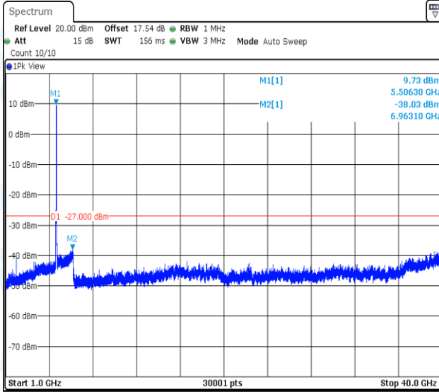
11N40MIMO-Ant1-5510-1000~40000-PASS
