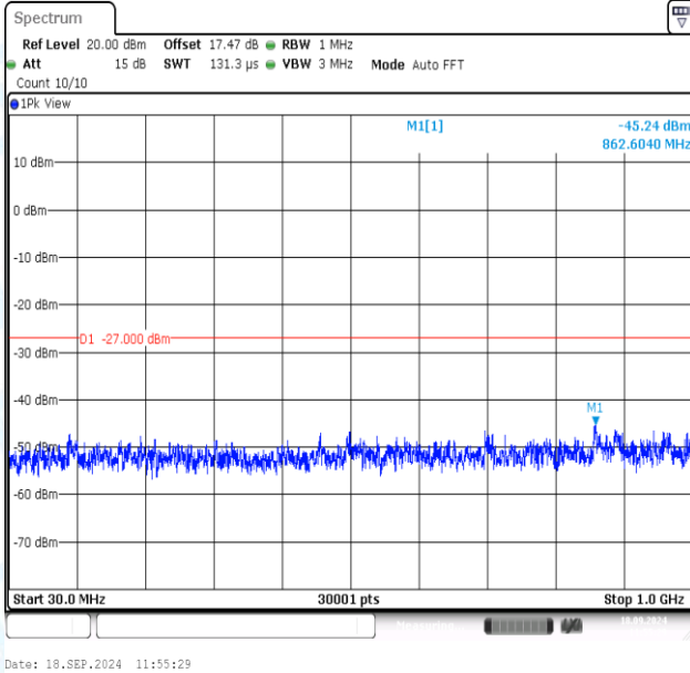
11AC20MIMO-Ant1-5260-30~1000-PASS
