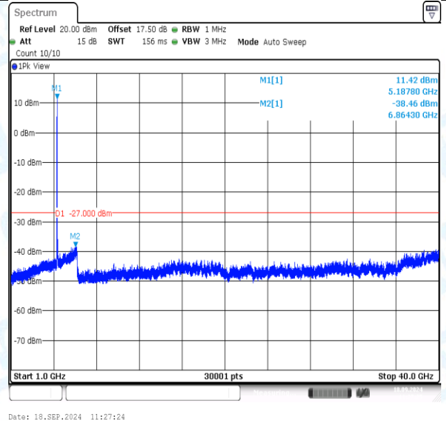
11AC20MIMO-Ant2-5180-1000~40000-PASS
