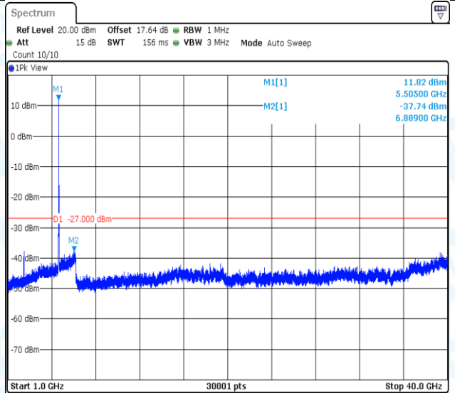
11N20MIMO-Ant2-5500-1000~40000-PASS
