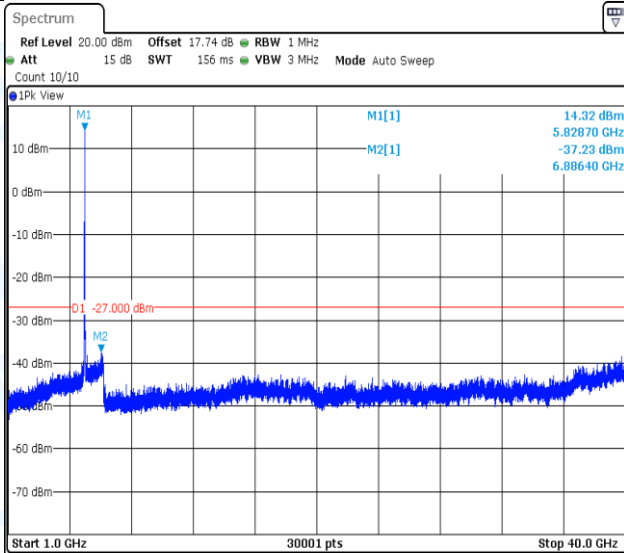
11N20MIMO-Ant1-5825-1000~40000-PASS
