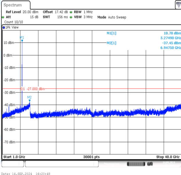
11N20MIMO-Ant1-5280-1000~40000-PASS
