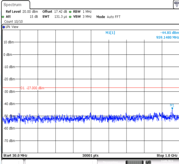
11N40MIMO-Ant1-5270-30~1000-PASS
