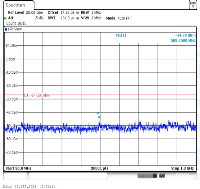
11AC20MIMO-Ant2-5260-30~1000-PASS
