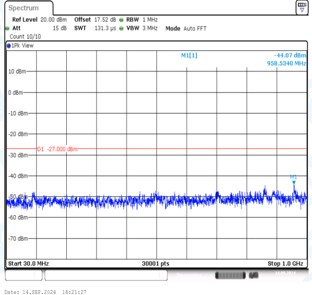
11N20MIMO-Ant2-5280-30~1000-PASS
