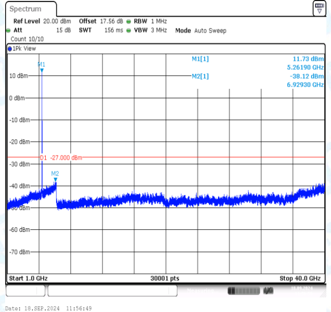
11AC20MIMO-Ant2-5260-1000~40000-PASS
