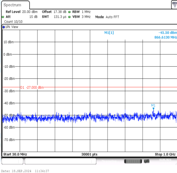
11AC20MIMO-Ant1-5200-30~1000-PASS
