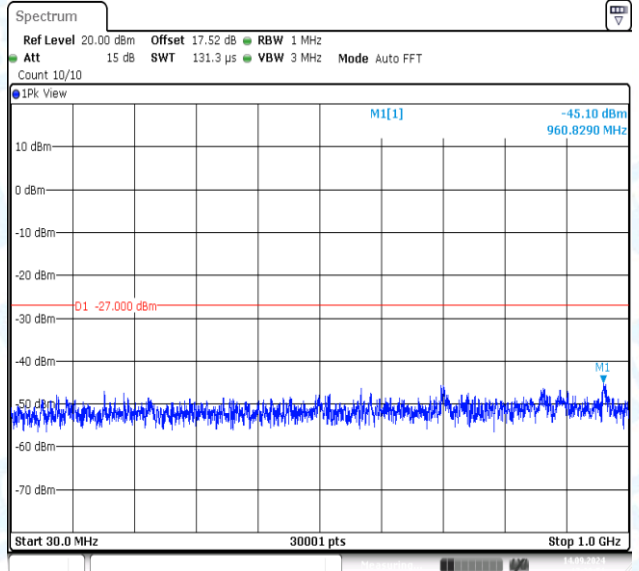
11N40MIMO-Ant2-5270-30~1000-PASS
