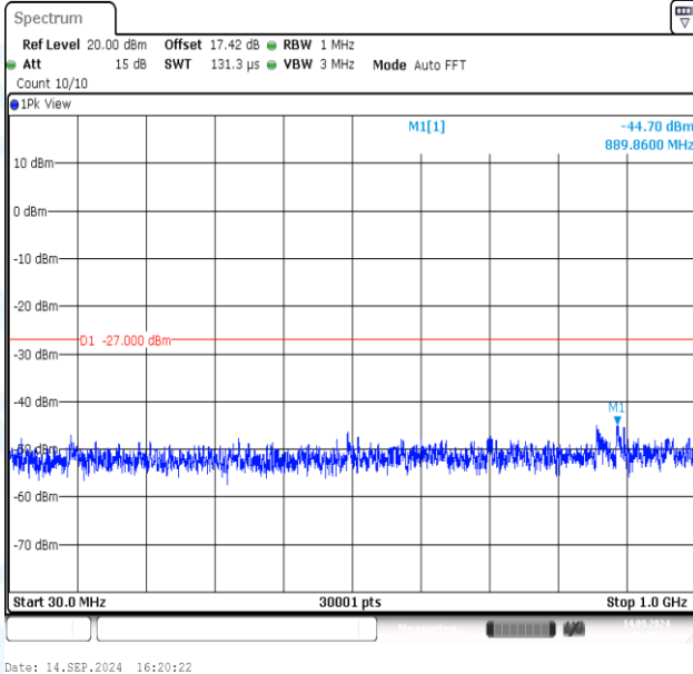
11N20MIMO-Ant1-5280-30~1000-PASS
