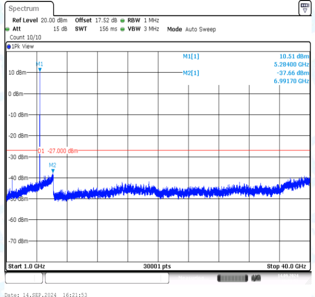
11N20MIMO-Ant2-5280-1000~40000-PASS
