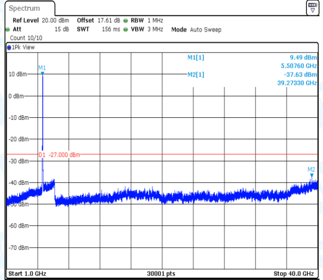
11N40MIMO-Ant2-5510-1000~40000-PASS
