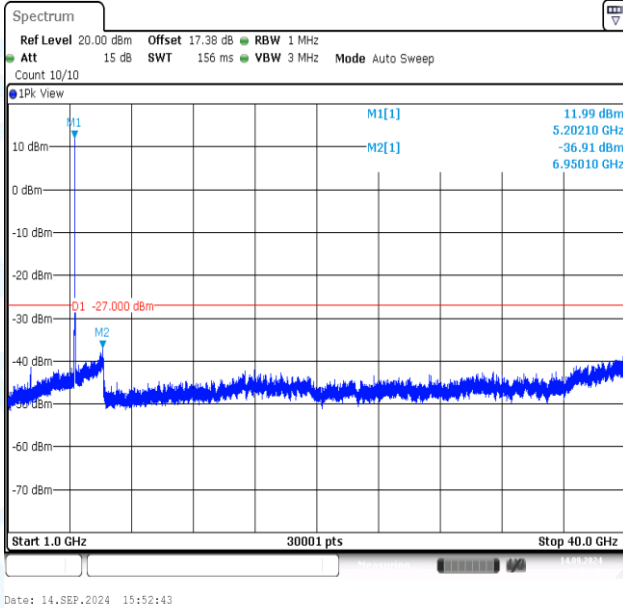
11N20MIMO-Ant1-5200-1000~40000-PASS
