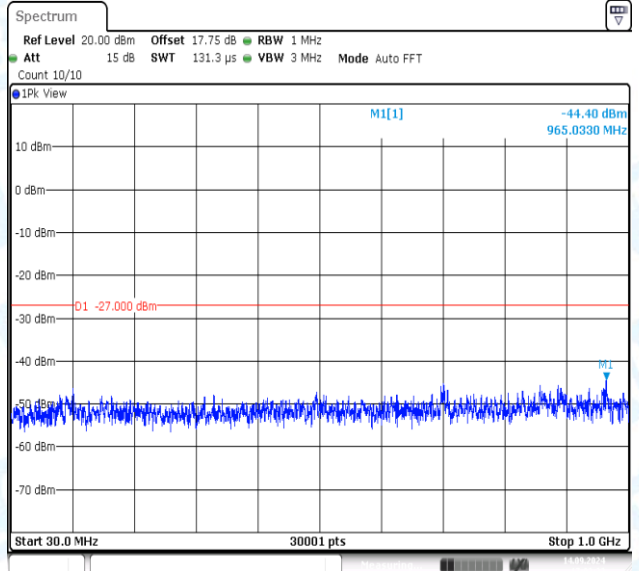
11N20MIMO-Ant2-5745-30~1000-PASS
