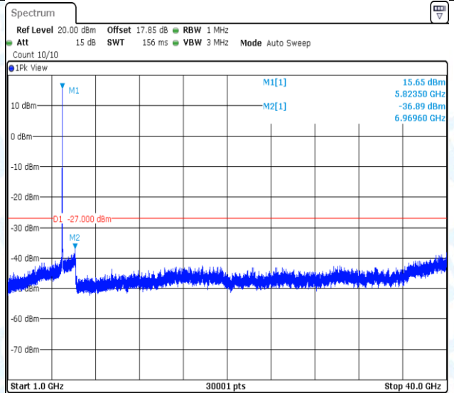
11N20MIMO-Ant2-5825-1000~40000-PASS
