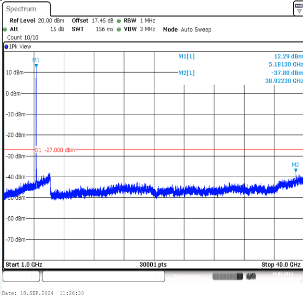
11AC20MIMO-Ant1-5180-1000~40000-PASS
