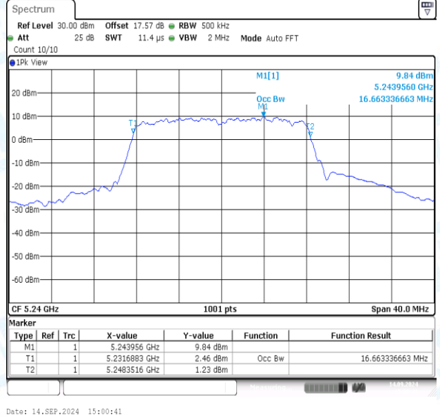
11A-Ant2-5240
