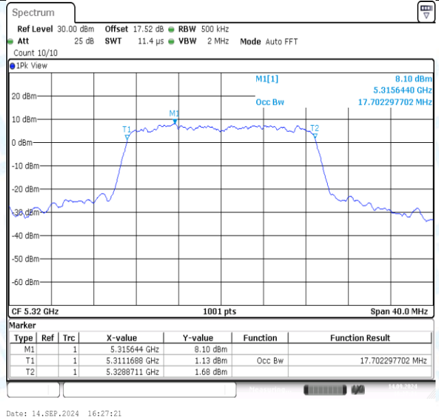
11N20MIMO-Ant2-5320
