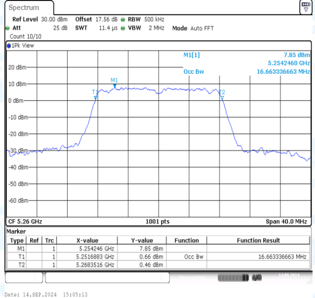
11A-Ant2-5260
