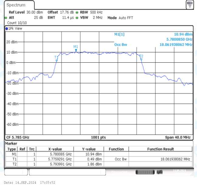
11N20MIMO-Ant2-5785
