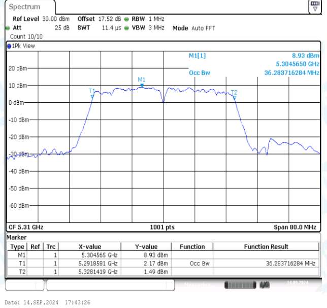
11N40MIMO-Ant2-5310
