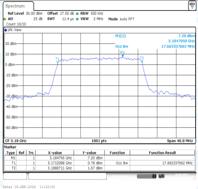
11AC20MIMO-Ant2-5180
