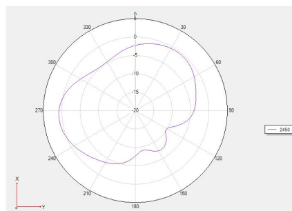
Theta =90 freq=2450MHz
