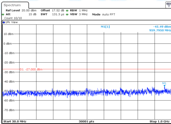
11AC40MIMO-Ant1-5270-30~1000-PASS
