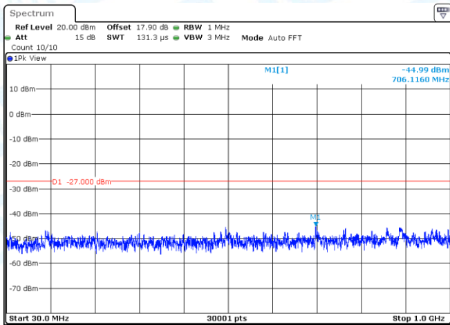
11AC80MIMO-Ant2-5610-30~1000-PASS
