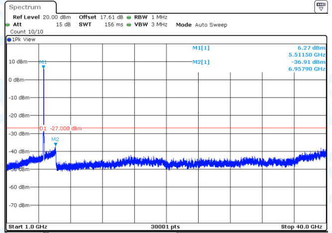
11AC40MIMO-Ant2-5510-1000~40000-PASS
