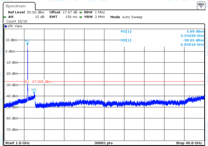
11AC40MIMO-Ant1-5550-1000~40000-PASS
