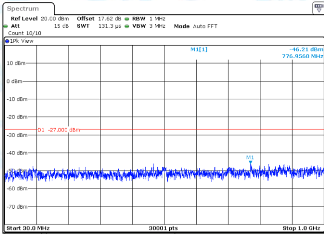
11AC40MIMO-Ant2-5510-30~1000-PASS
