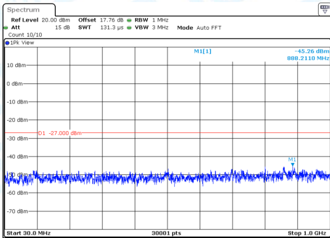
11AC40MIMO-Ant1-5795-30~1000-PASS
