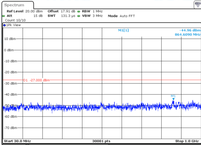
11AC80MIMO-Ant2-5690-30~1000-PASS
