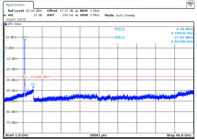
11AC40MIMO-Ant2-5230-1000~40000-PASS
