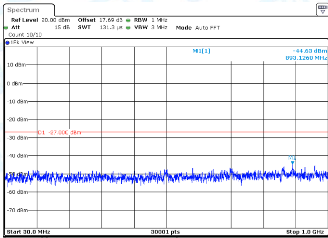
11AC40MIMO-Ant2-5755-30~1000-PASS
