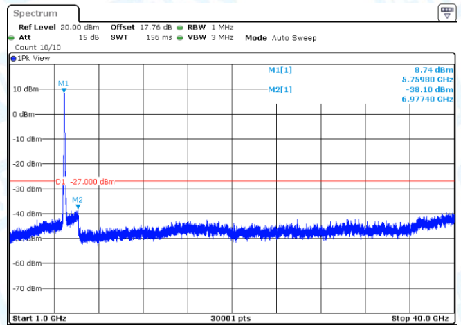
11AC80MIMO-Ant1-5775-1000~40000-PASS
