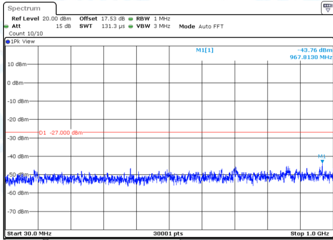
11AC80MIMO-Ant2-5290-30~1000-PASS
