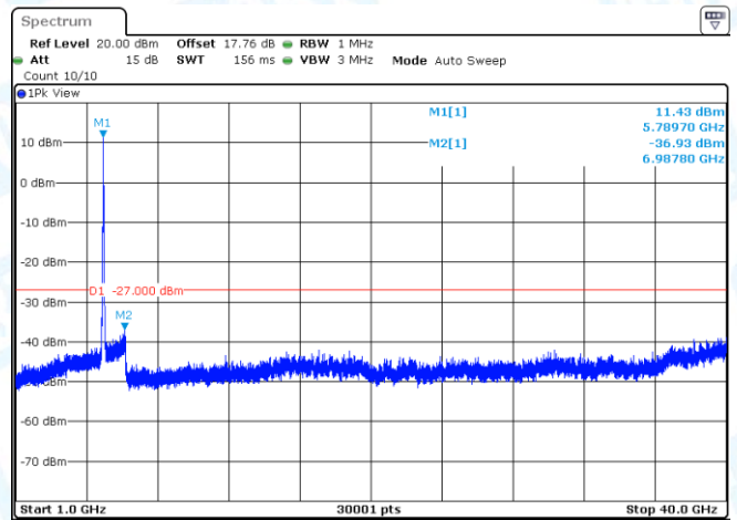
11AC40MIMO-Ant1-5795-1000~40000-PASS
