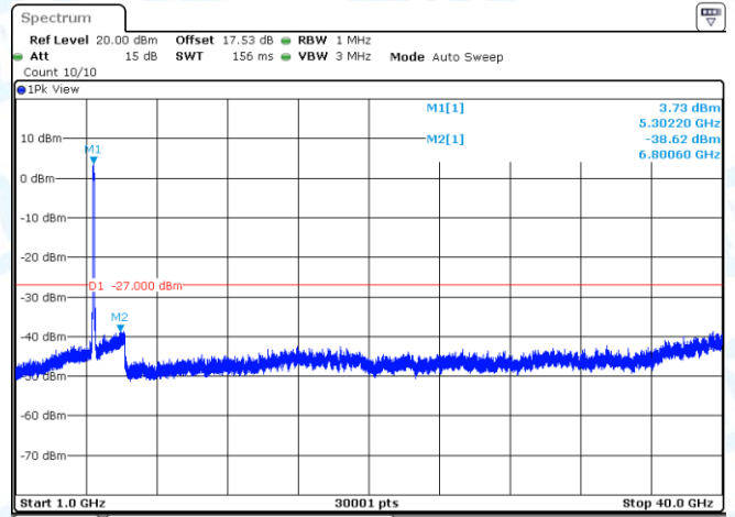
11AC80MIMO-Ant2-5290-1000~40000-PASS
