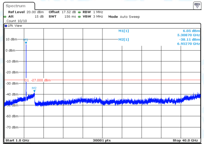
11AC40MIMO-Ant1-5310-1000~40000-PASS
