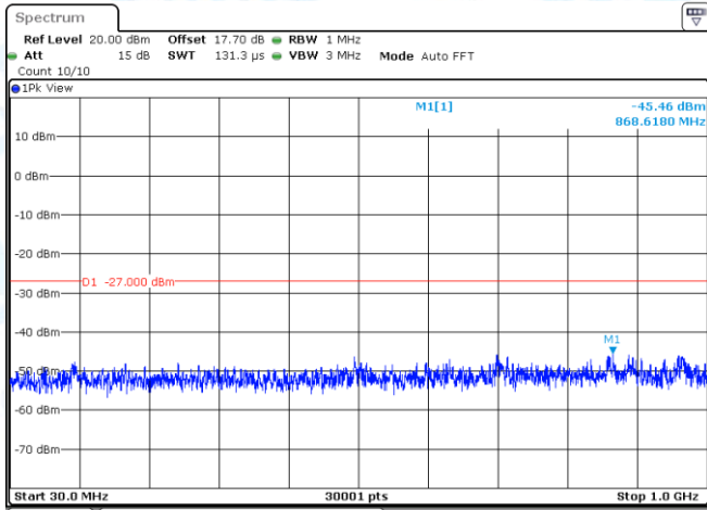
11AC80MIMO-Ant1-5610-30~1000-PASS
