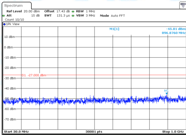
11AC80MIMO-Ant2-5210-30~1000-PASS
