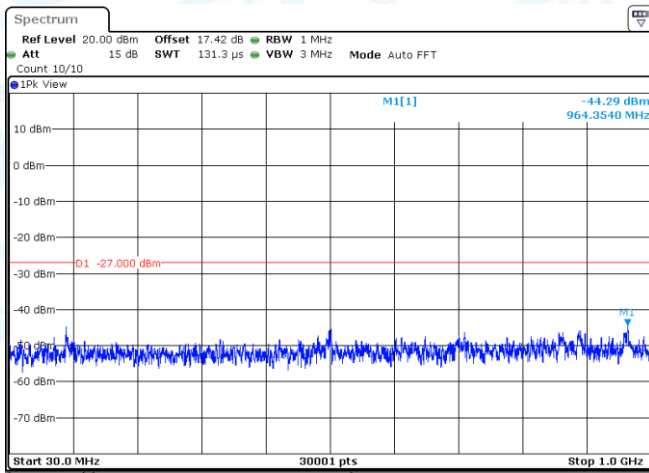
11AC40MIMO-Ant2-5230-30~1000-PASS
