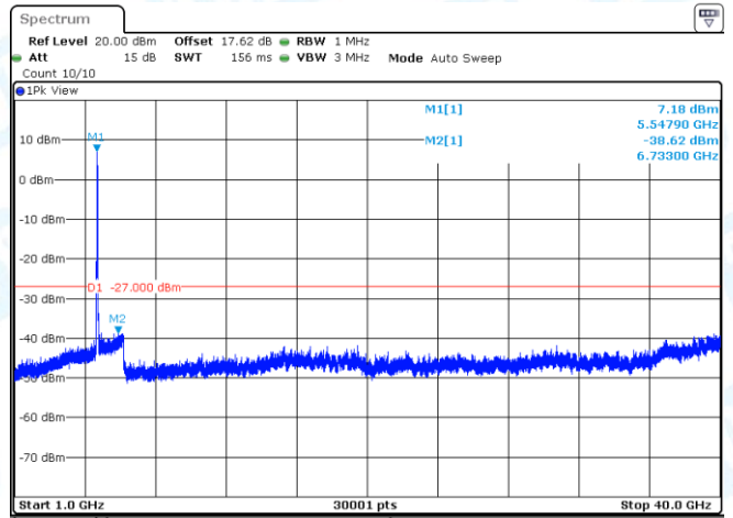
11AC40MIMO-Ant2-5510-1000~40000-PASS
