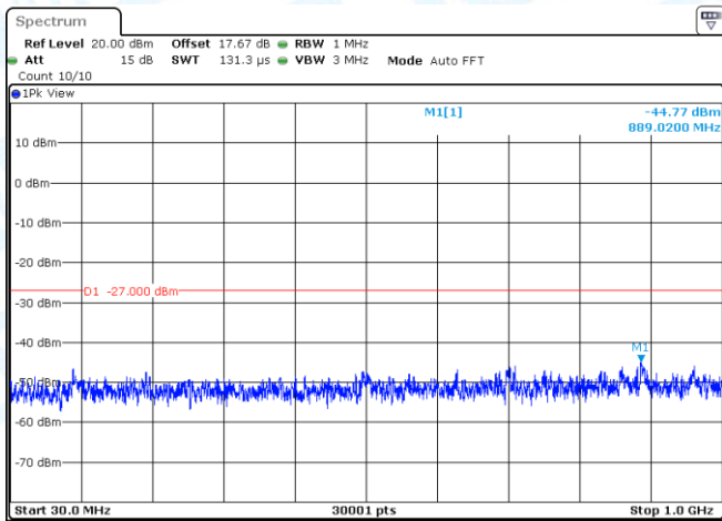
11AC40MIMO-Ant1-5550-30~1000-PASS
