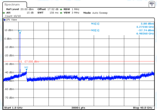
11AC40MIMO-Ant1-5270-1000~40000-PASS
