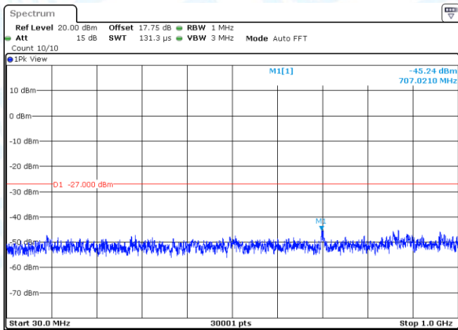
11AC40MIMO-Ant2-5710-30~1000-PASS
