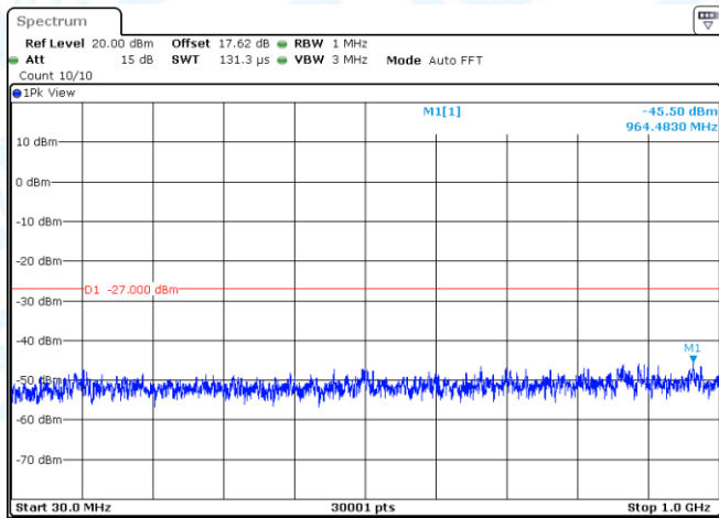
11AC80MIMO-Ant1-5530-30~1000-PASS
