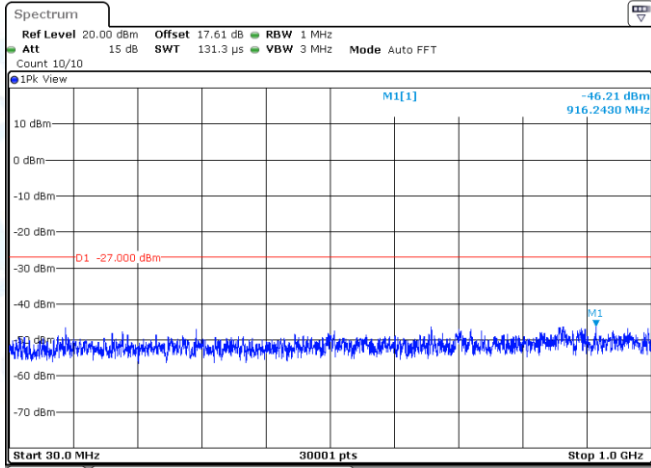
11AC40MIMO-Ant2-5510-30~1000-PASS
