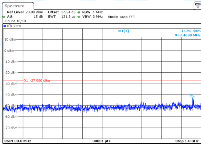
11AC40MIMO-Ant2-5310-30~1000-PASS
