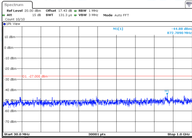
11AC40MIMO-Ant1-5310-30~1000-PASS
