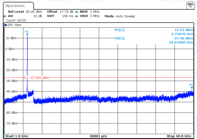
11AC40MIMO-Ant2-5710-1000~40000-PASS
