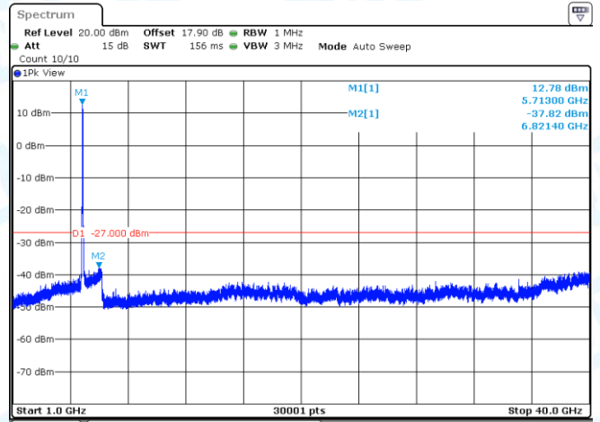
11AC40MIMO-Ant1-5710-1000~40000-PASS
