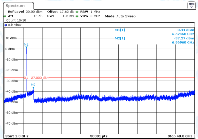
11AC80MIMO-Ant1-5530-1000~40000-PASS
