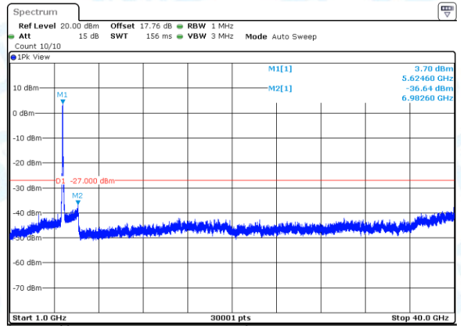
11AC80MIMO-Ant1-5610-1000~40000-PASS
