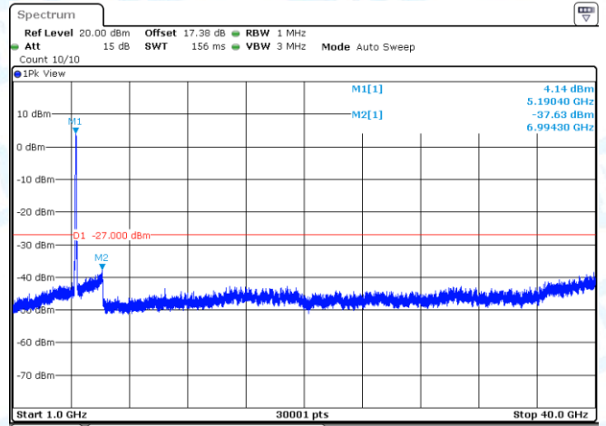
11AC80MIMO-Ant1-5210-1000~40000-PASS
