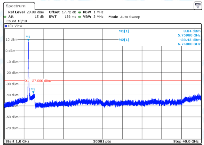
11AC80MIMO-Ant2-5690-1000~40000-PASS
