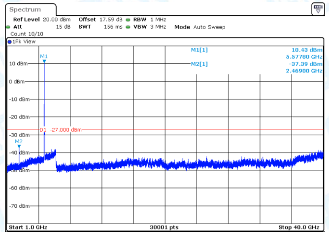
11N20MIMO-Ant2-5500-1000~40000-PASS
