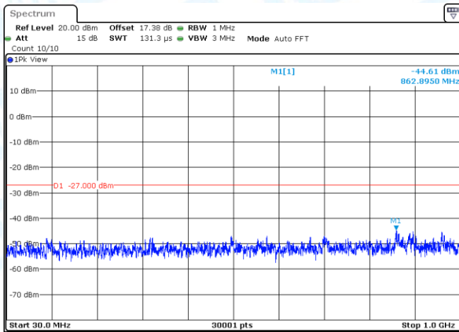
11AC20MIMO-Ant2-5180-30~1000-PASS
