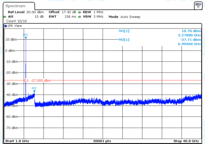
11AC20MIMO-Ant2-5260-1000~40000-PASS
