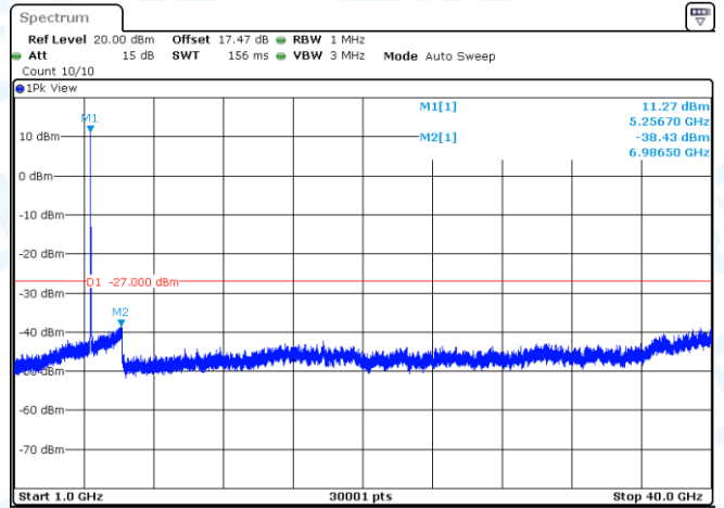
11AC20MIMO-Ant1-5260-1000~40000-PASS
