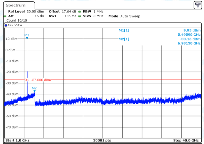
11AC20MIMO-Ant1-5500-1000~40000-PASS
