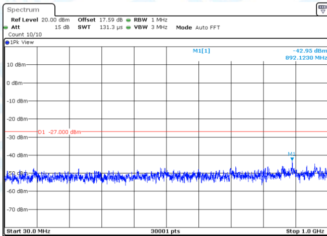
11N20MIMO-Ant2-5500-30~1000-PASS
