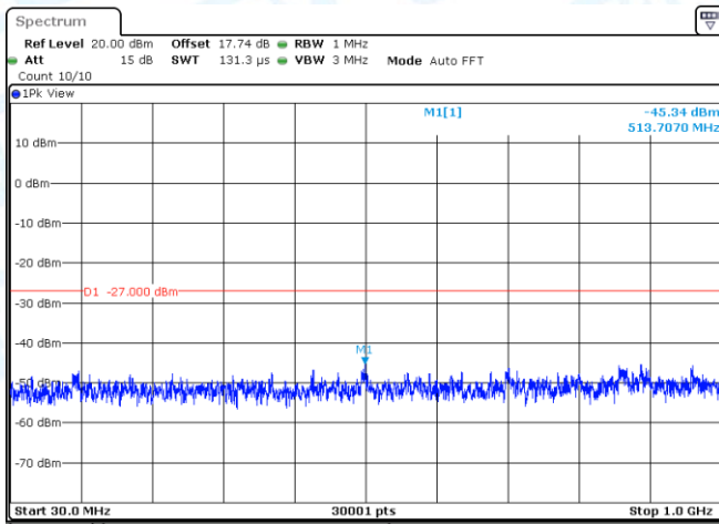
11AC20MIMO-Ant2-5785-30~1000-PASS
