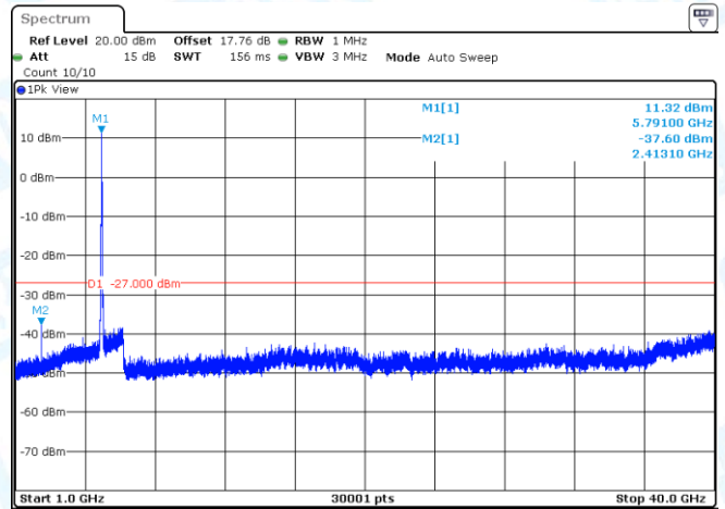
11N40MIMO-Ant1-5795-1000~40000-PASS
