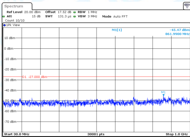
11N40MIMO-Ant1-5270-30~1000-PASS
