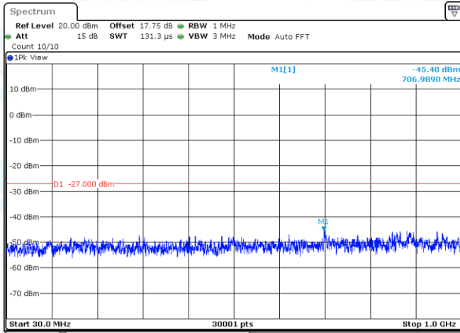
11AC20MIMO-Ant1-5745-30~1000-PASS
