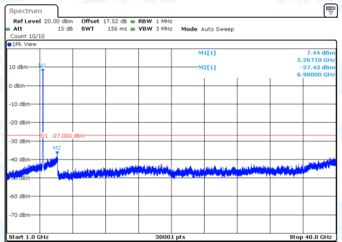
11N40MIMO-Ant1-5270-1000~40000-PASS
