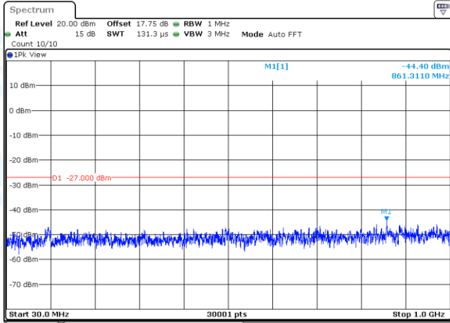
11N40MIMO-Ant2-5755-30~1000-PASS
