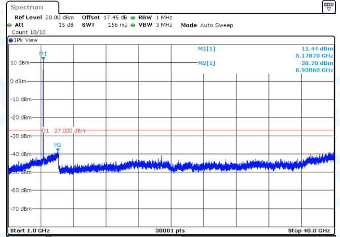
11AC20MIMO-Ant1-5180-1000~40000-PASS
