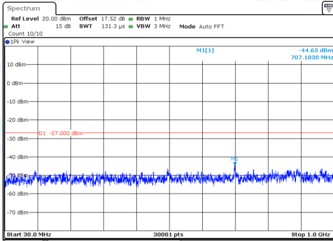
11AC20MIMO-Ant2-5280-30~1000-PASS
