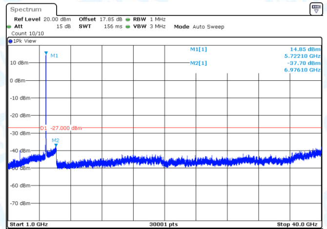
11N20MIMO-Ant1-5720-1000~40000-PASS
