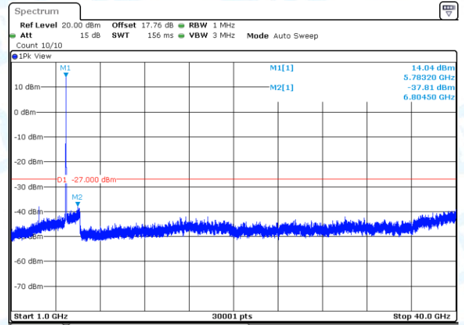
11AC20MIMO-Ant2-5785-1000~40000-PASS
