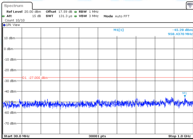
11AC20MIMO-Ant2-5500-30~1000-PASS
