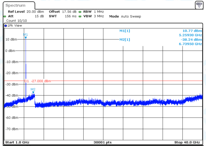
11AC20MIMO-Ant1-5260-1000~40000-PASS
