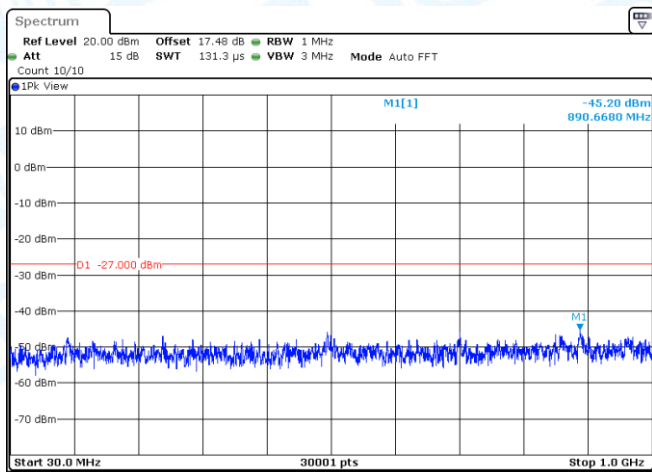
11N40MIMO-Ant2-5190-30~1000-PASS
