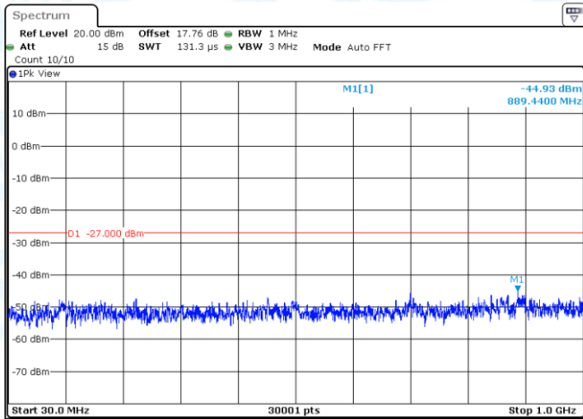
11N40MIMO-Ant1-5795-30~1000-PASS
