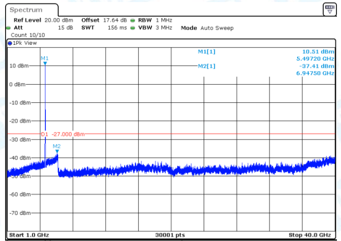
11N20MIMO-Ant1-5500-1000~40000-PASS
