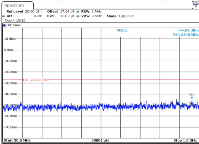
11AC20MIMO-Ant1-5500-30~1000-PASS
