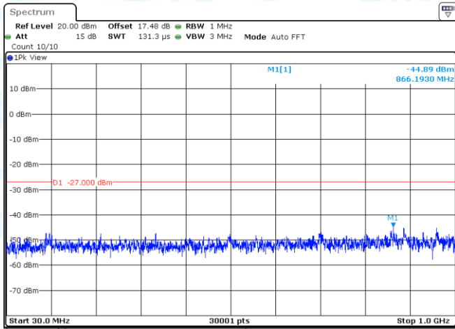
11AC40MIMO-Ant1-5190-30~1000-PASS
