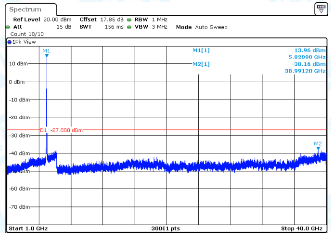
11N20MIMO-Ant1-5825-1000~40000-PASS
