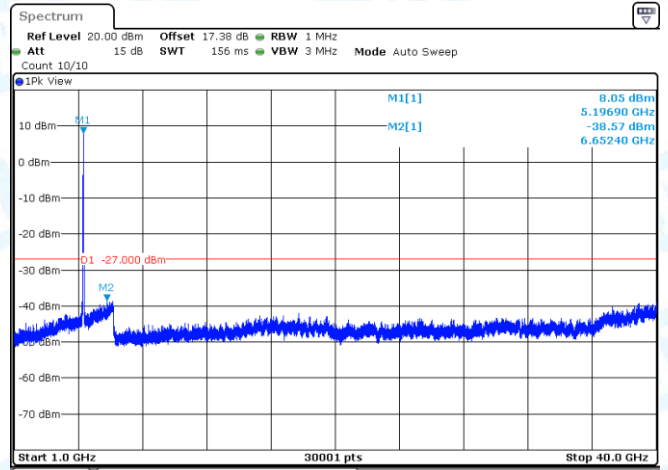
11N40MIMO-Ant1-5190-1000~40000-PASS
