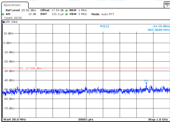
11N40MIMO-Ant2-5310-30~1000-PASS
