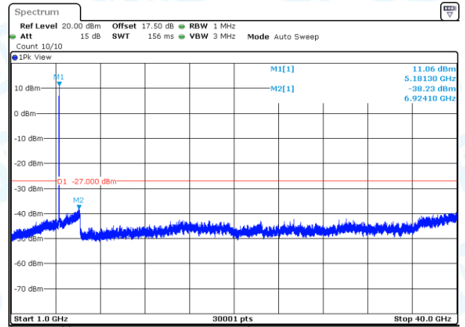
11AC20MIMO-Ant1-5180-1000~40000-PASS
