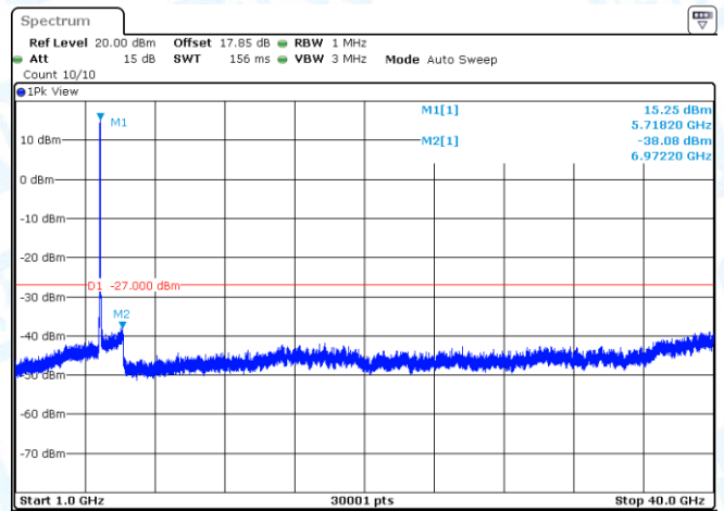
11AC20MIMO-Ant1-5720-1000~40000-PASS
