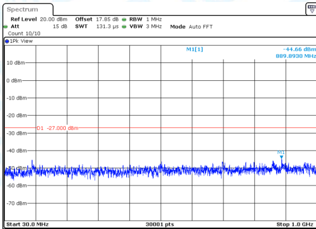
11N20MIMO-Ant1-5720-30~1000-PASS
