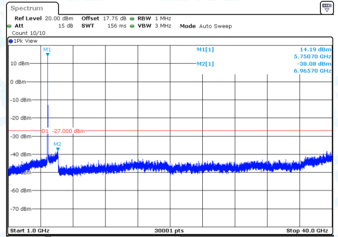
11AC20MIMO-Ant1-5745-1000~40000-PASS
