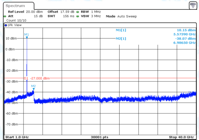
11AC20MIMO-Ant2-5500-1000~40000-PASS
