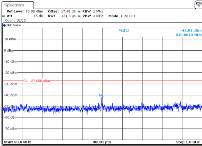
11AC20MIMO-Ant2-5200-30~1000-PASS
