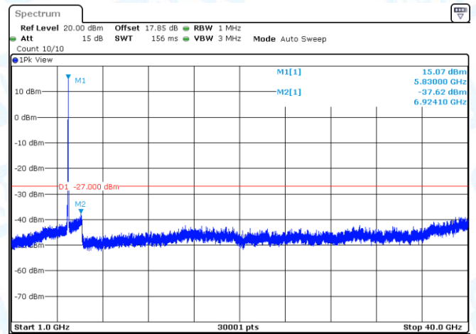
11AC20MIMO-Ant1-5825-1000~40000-PASS
