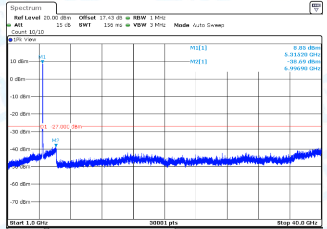
11N40MIMO-Ant1-5310-1000~40000-PASS
