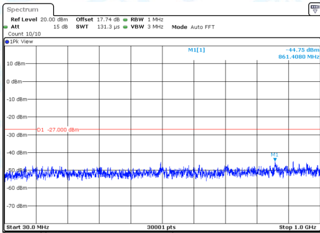
11N20MIMO-Ant2-5785-30~1000-PASS
