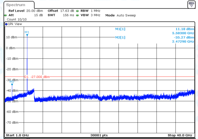
11N20MIMO-Ant2-5580-1000~40000-PASS
