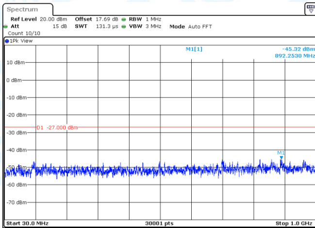
11AC20MIMO-Ant2-5745-30~1000-PASS
