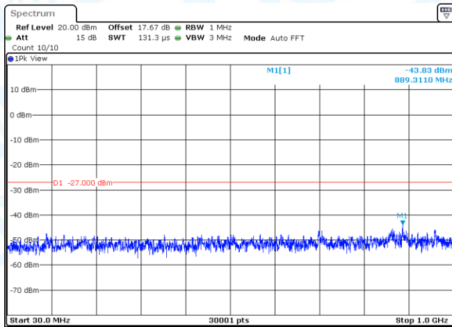
11N40MIMO-Ant1-5550-30~1000-PASS
