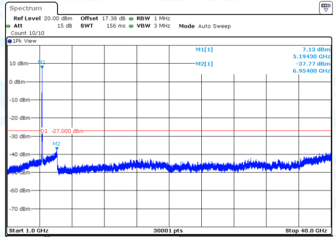
11AC40MIMO-Ant1-5190-1000~40000-PASS
