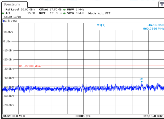
11AC20MIMO-Ant1-5180-30~1000-PASS
