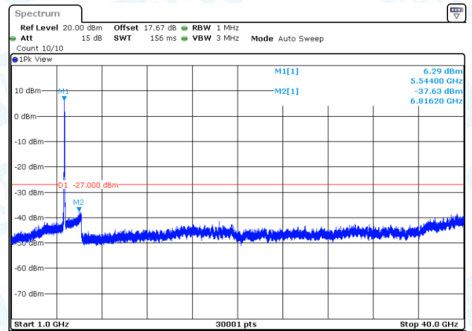
11N40MIMO-Ant1-5550-1000~40000-PASS
