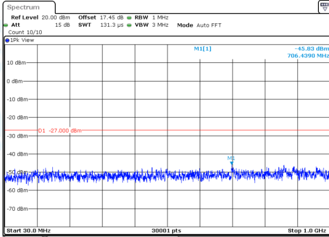
11AC20MIMO-Ant1-5180-30~1000-PASS
