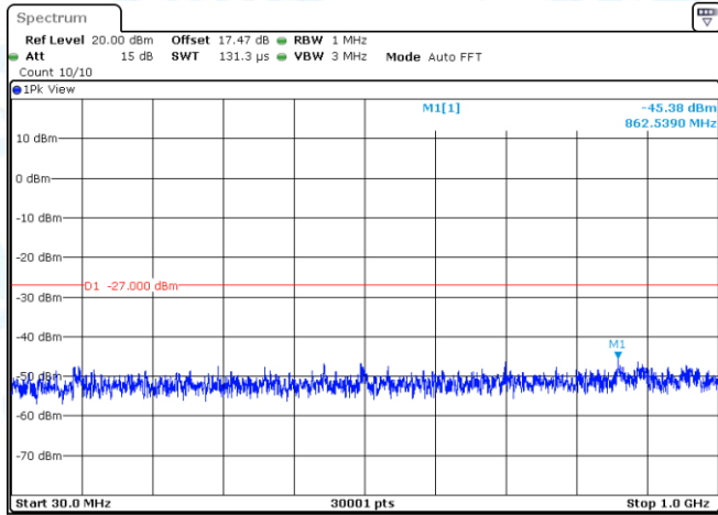
11AC20MIMO-Ant1-5260-30~1000-PASS
