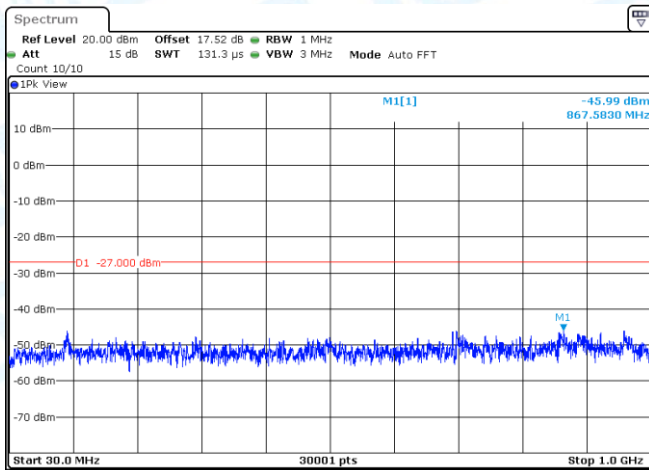
11AC20MIMO-Ant1-5320-30~1000-PASS
