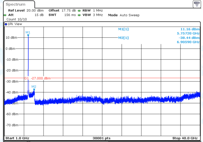
11N40MIMO-Ant2-5755-1000~40000-PASS
