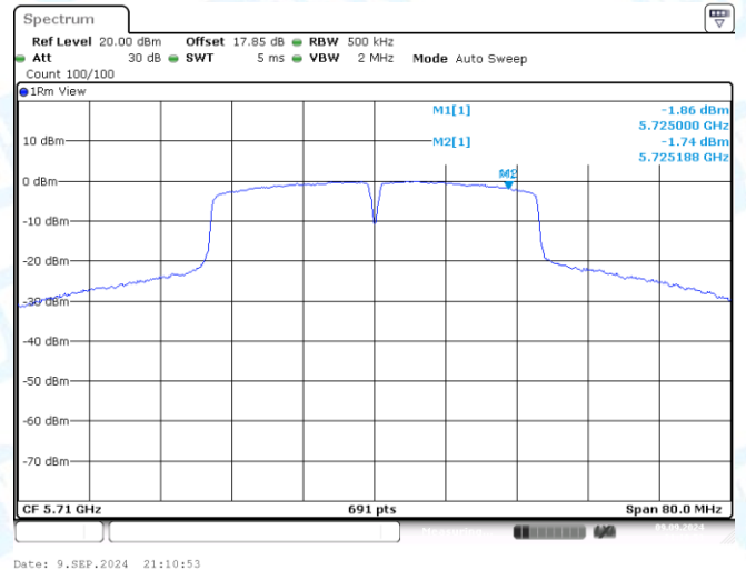
11AC40MIMO-Ant2-5710_UNII-3-PASS
