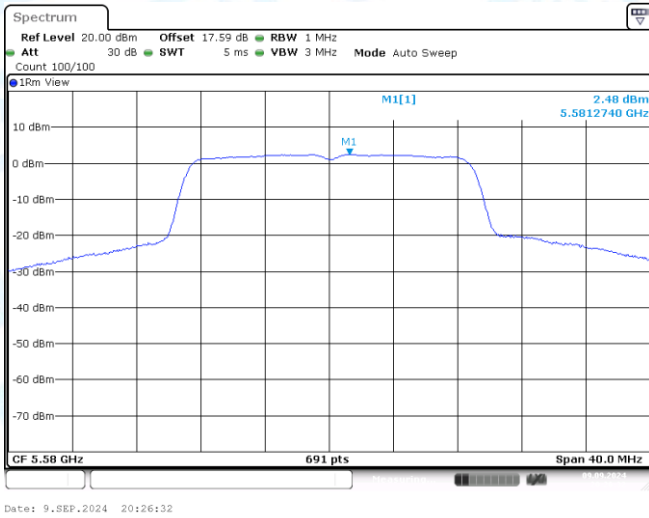
11AC20MIMO-Ant1-5580-PASS
