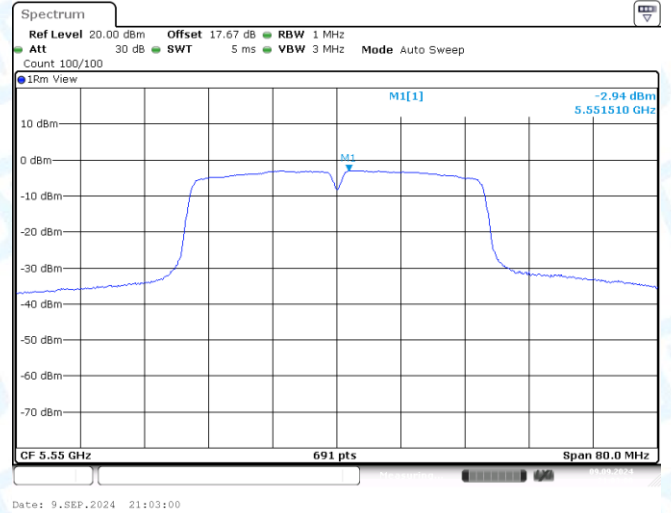
11AC40MIMO-Ant2-5550-PASS
