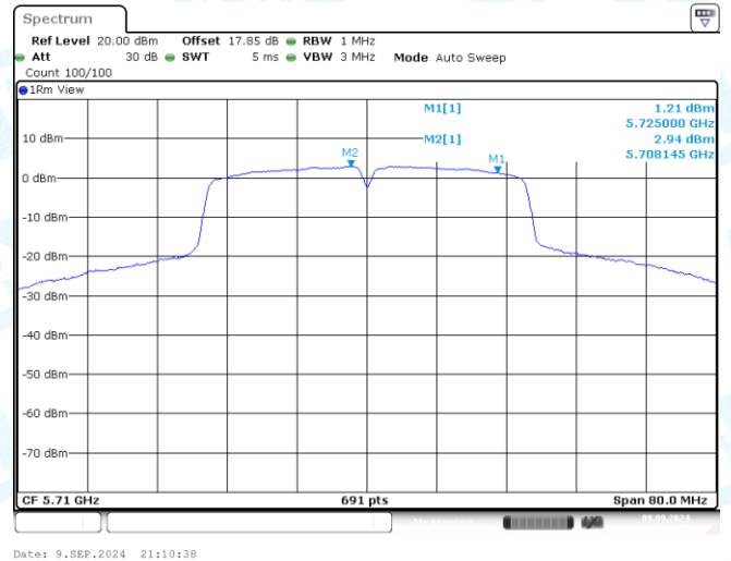
11AC40MIMO-Ant2-5710_UNII-2C-PASS
