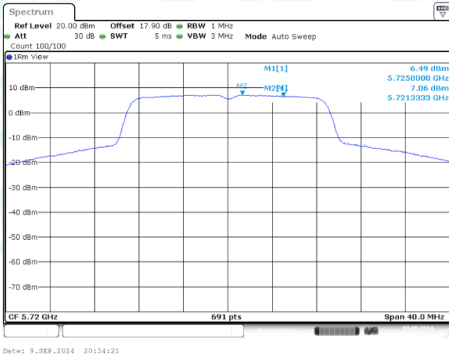
11AC20MIMO-Ant1-5720_UNII-2C-PASS
