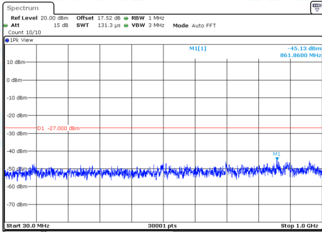
11N20MIMO-Ant2-5280-30~1000-PASS
