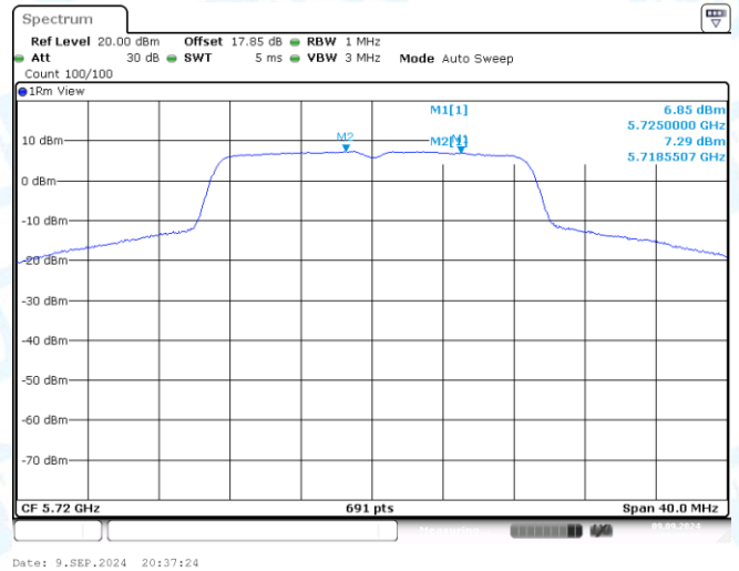
11AC20MIMO-Ant2-5720_UNII-2C-PASS
