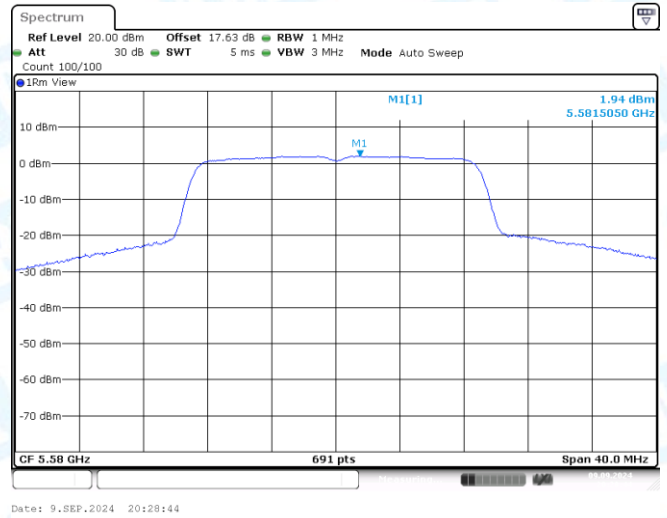
11AC20MIMO-Ant2-5580-PASS
