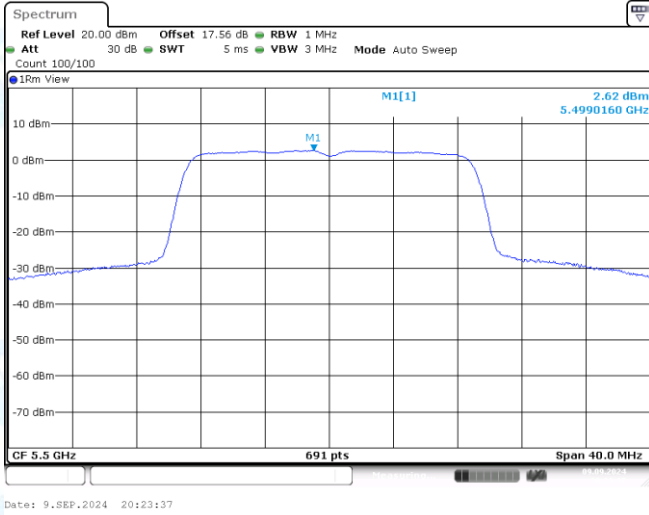
11AC20MIMO-Ant1-5500-PASS
