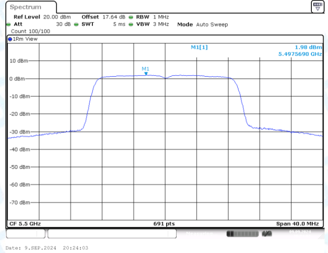
11AC20MIMO-Ant2-5500-PASS
