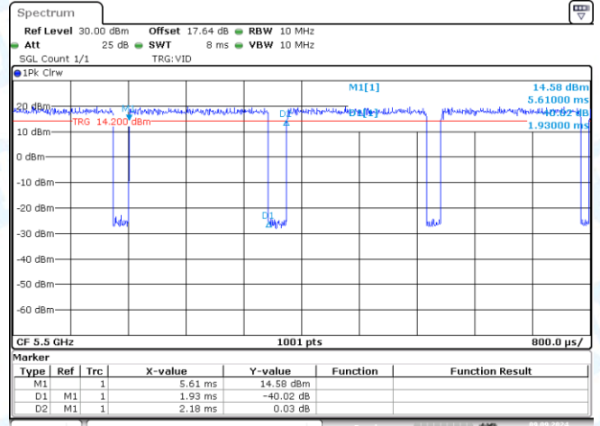
NTVN-11AC20MIMO-Ant2-5500
