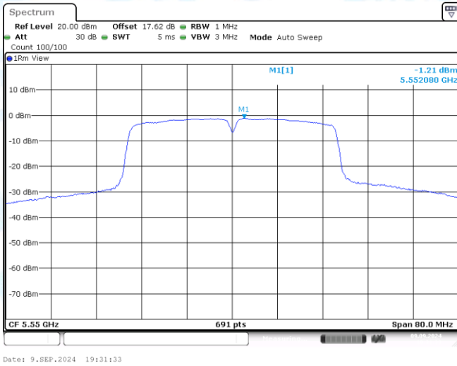
11N40MIMO-Ant1-5550-PASS
