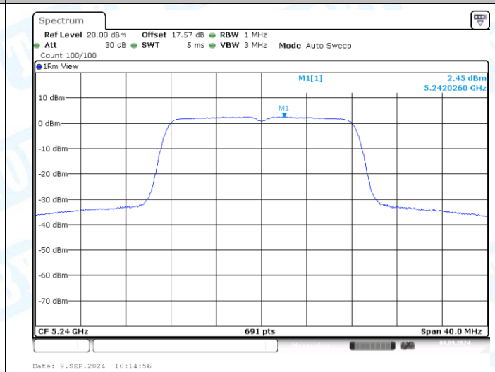
11A-Ant2-5240-PASS
