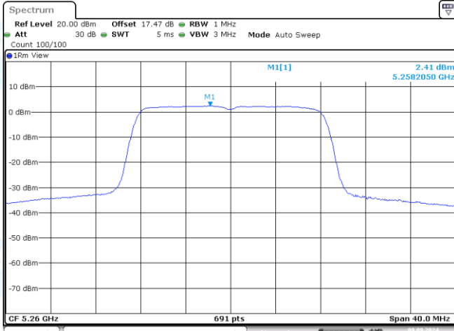
11A-Ant1-5260-PASS
