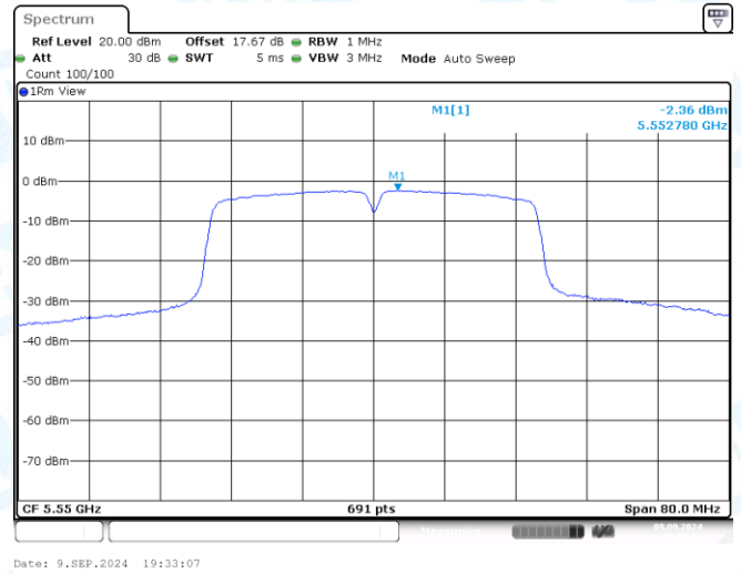
11N40MIMO-Ant2-5550-PASS
