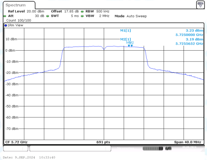
11A-Ant2-5720_UNII-3-PASS
