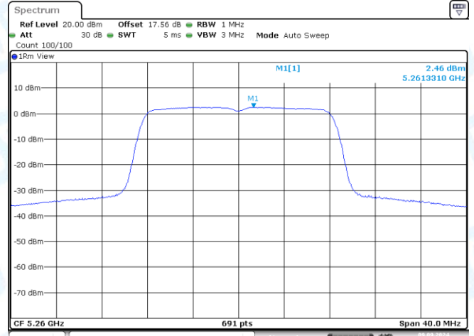
11A-Ant2-5260-PASS
