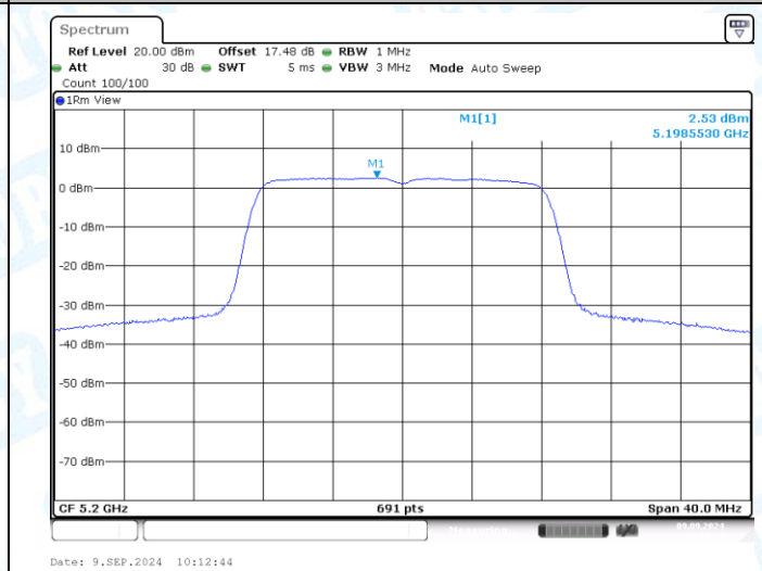
11A-Ant2-5200-PASS
