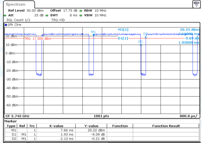
NTVN-11AC20MIMO-Ant2-5745
