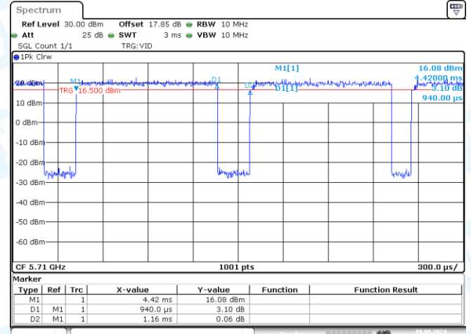
NTNV-11N40MIMO-Ant2-5710
