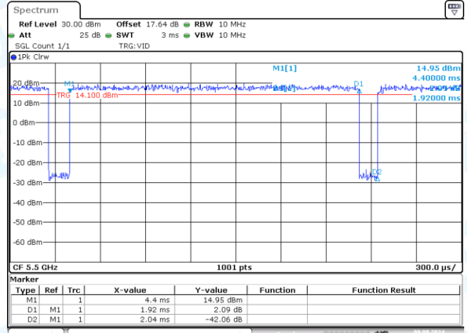
NTNV-11N20MIMO-Ant2-5500
