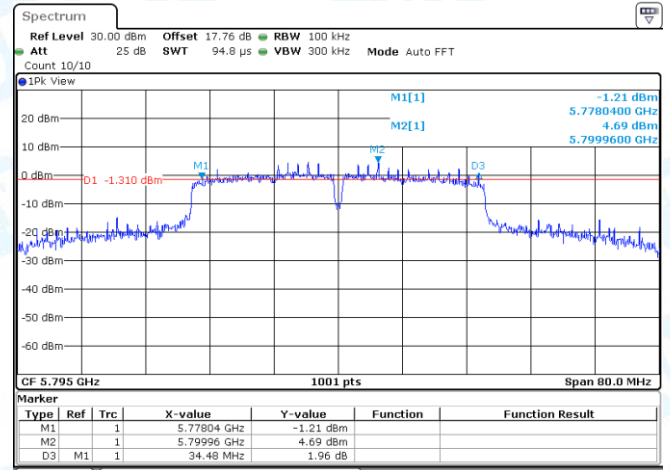
11AC40MIMO-Ant2-5795-PASS
