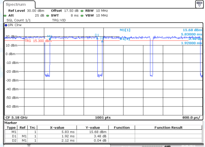
NTNV-11N20MIMO-Ant2-5180
