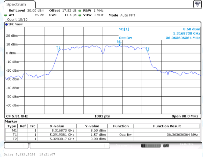
11N40MIMO-Ant2-5310
