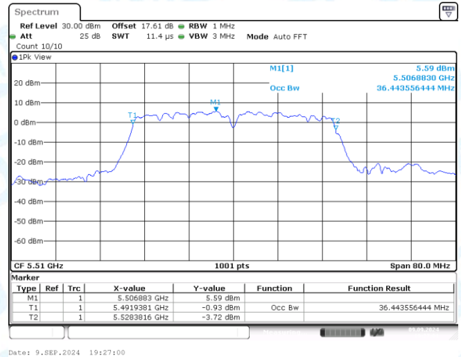
11N40MIMO-Ant2-5510
