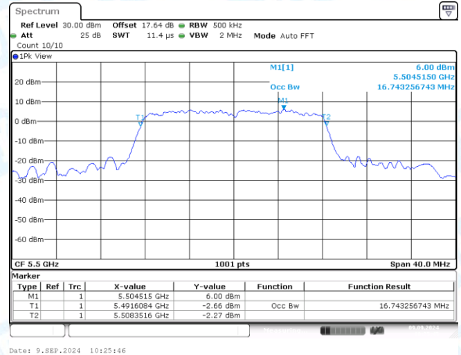
11A-Ant2-5500
