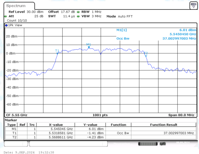
11N40MIMO-Ant2-5550
