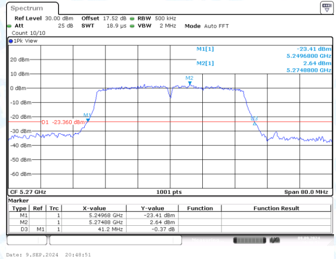
11AC40MIMO-Ant2-5270
