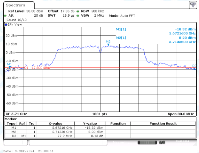
11AC40MIMO-Ant2-5710
