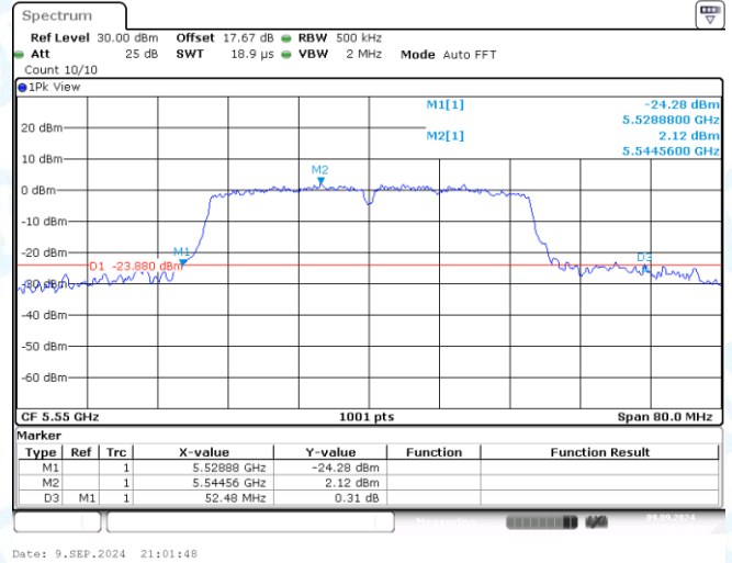
11AC40MIMO-Ant2-5550
