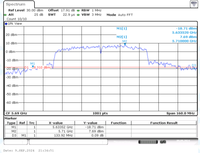
11AC80MIMO-Ant2-5690
