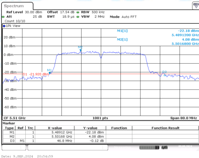
11AC40MIMO-Ant1-5510
