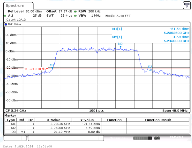
11N20MIMO-Ant2-5240
