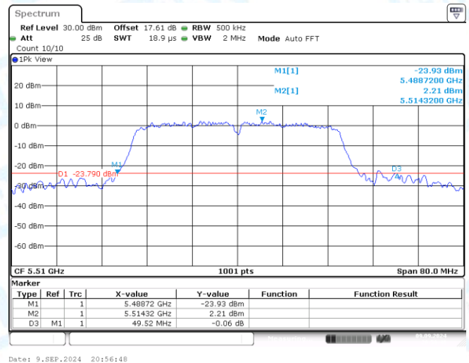
11AC40MIMO-Ant2-5510
