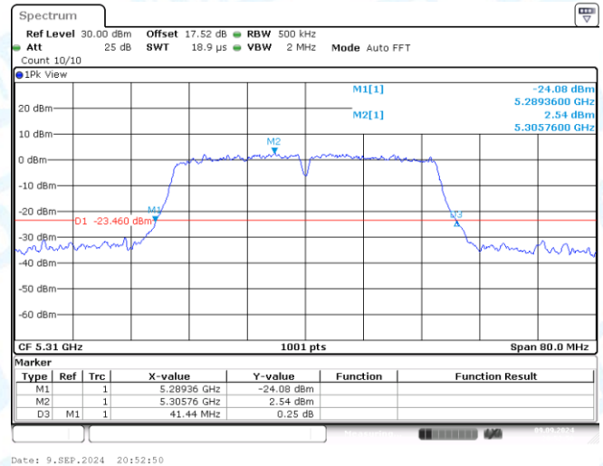
11AC40MIMO-Ant2-5310
