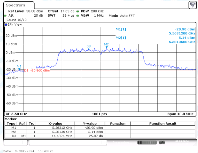
11N20MIMO-Ant2-5580
