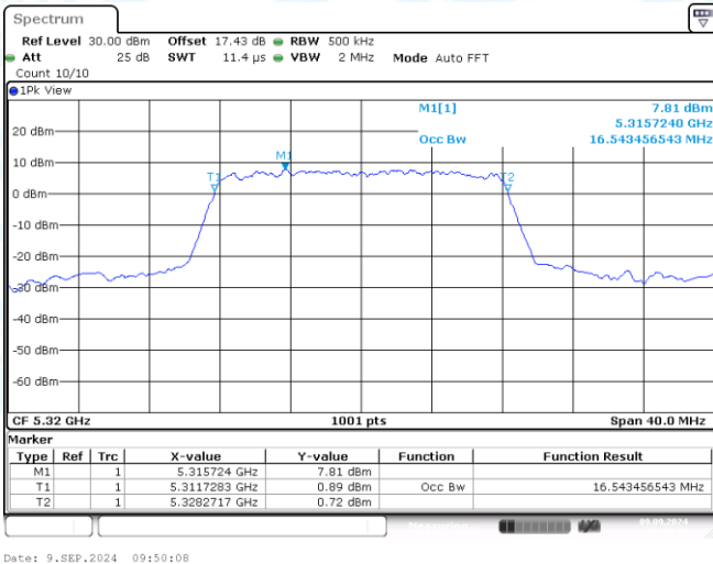
11A-Ant1-5320
