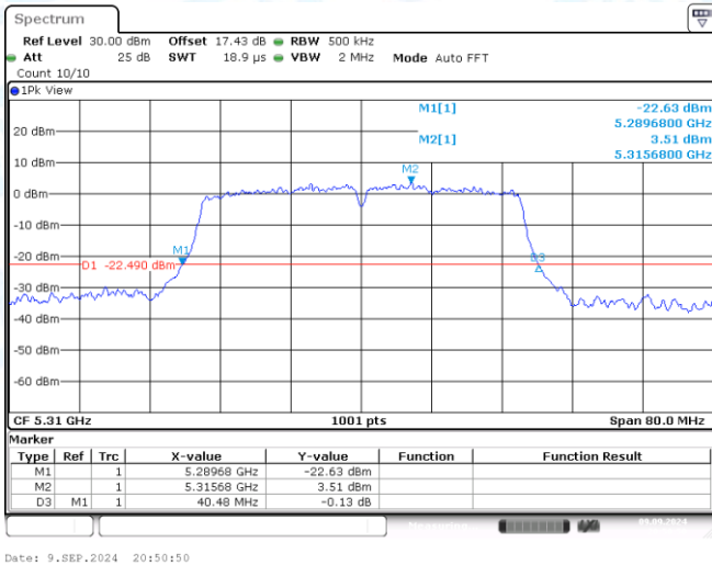
11AC40MIMO-Ant1-5310
