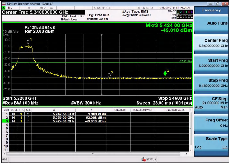
11N20SISO-Ant1-5240-PASS
