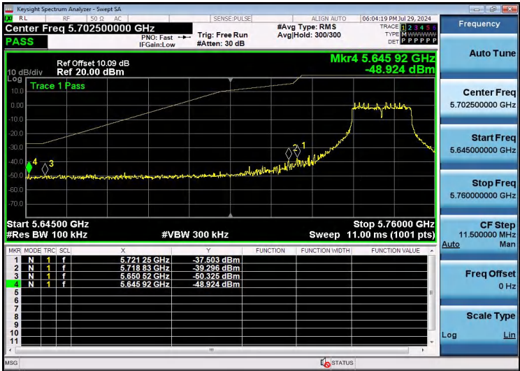
11A-Ant1-5745-PASS
