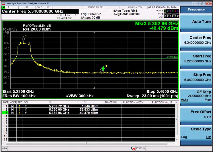
11AC20SISO-Ant1-5240-PASS
