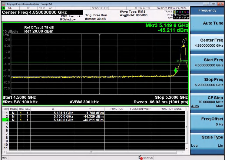
11N20SISO-Ant1-5180-PASS
