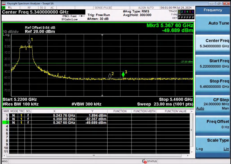
11A-Ant1-5240-PASS
