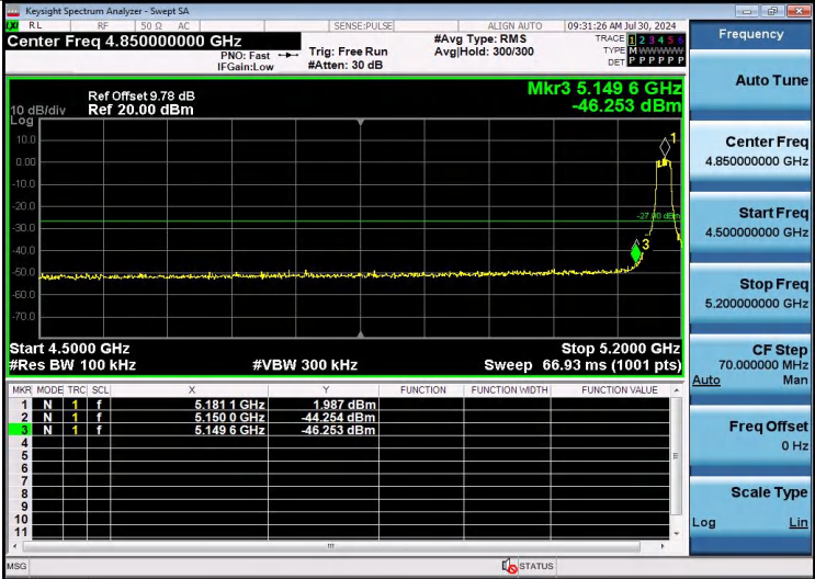
11A-Ant1-5180-PASS
