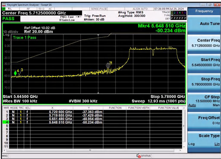
11AC40SISO-Ant1-5755-PASS
