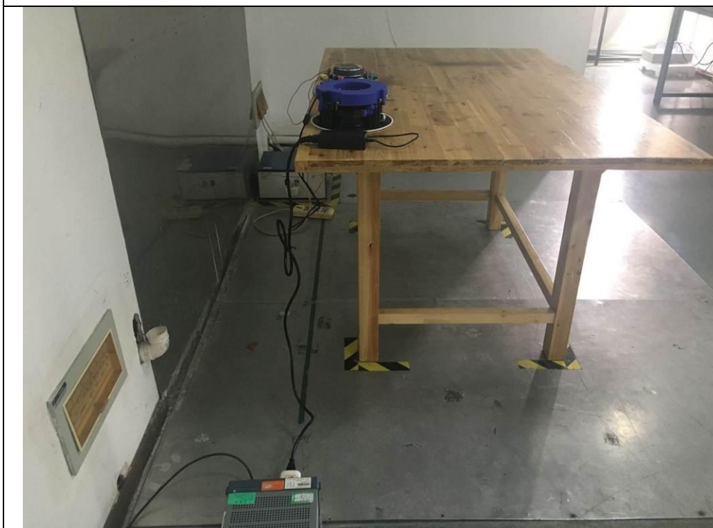
Conducted Emissions Setup Side View
