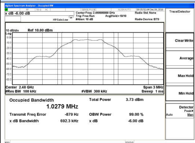
BT LE-left earbud -High channel
