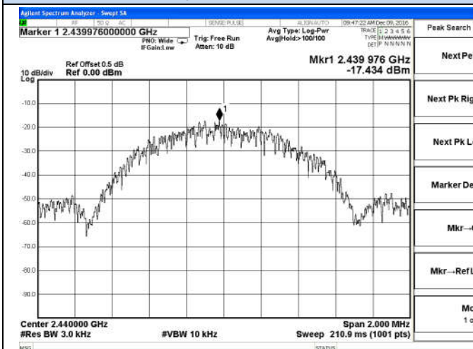
BT LE-right earbud-Middle channel
