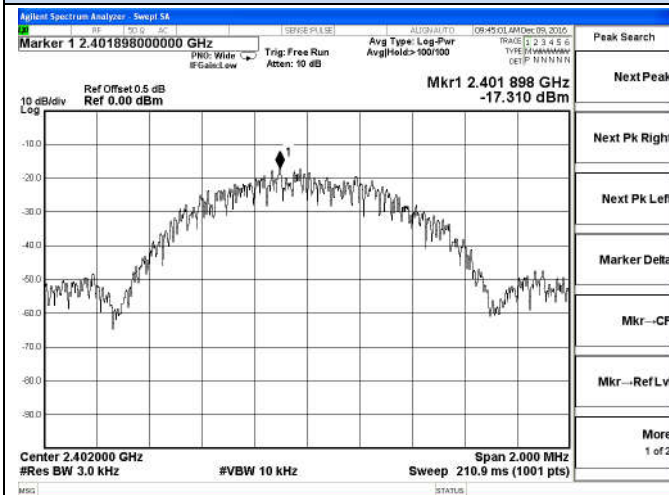
BT LE-right earbud-Low channel
