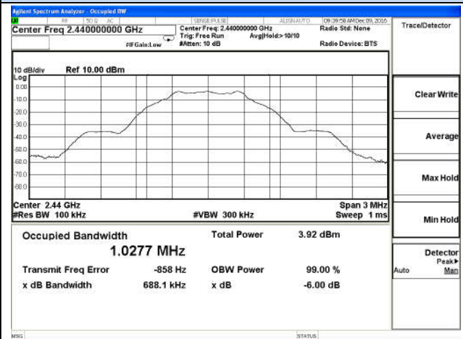
BT LE-left earbud -Middle channel
