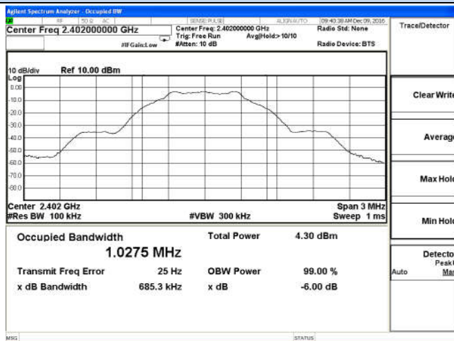
BT LE-right earbud-Low channel
