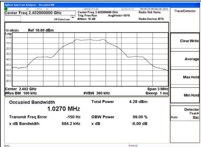
BT LE-left earbud-Low channel
