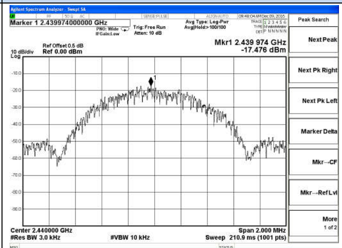
BT LE-left earbud -Middle channel
