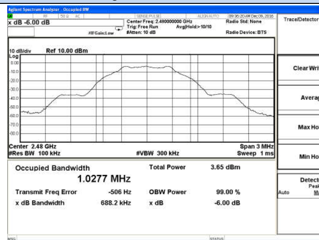
BT LE-right earbud-High channel
