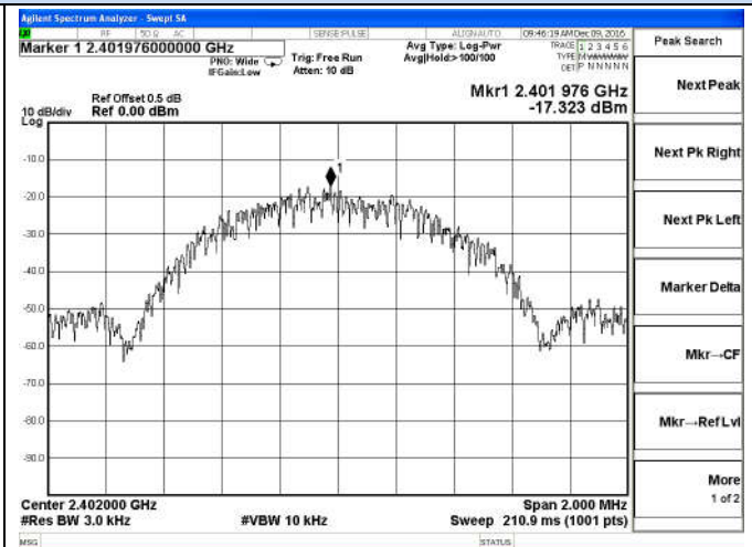
BT LE-left earbud-Low channel
