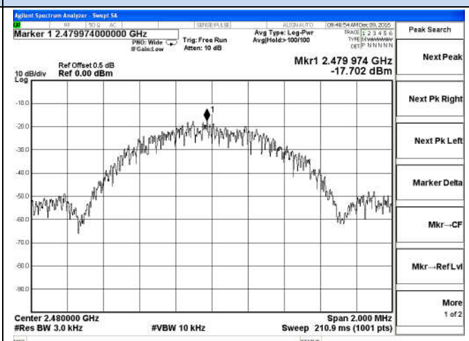
BT LE-left earbud -High channel
