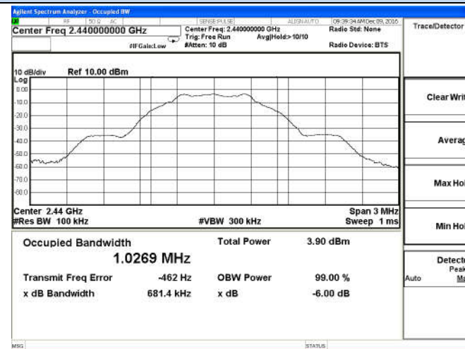
BT LE-right earbud-Middle channel
