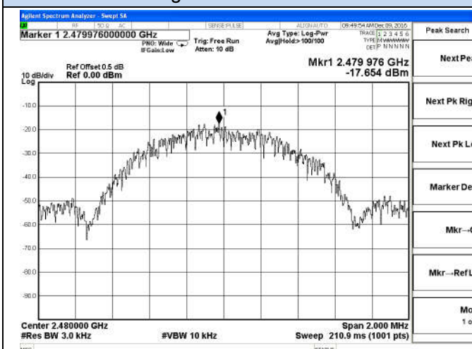
BT LE-right earbud-High channel
