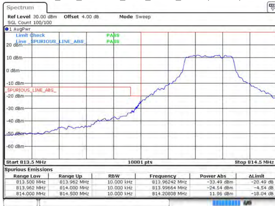
LTE_B26_CH26697_1.4M_QPSK_1RB0 (Part 90)
