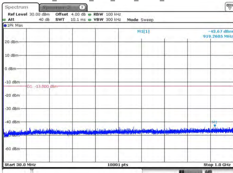
B25_CH26047_1.4M_1RB2_QPSK_Below 1G
