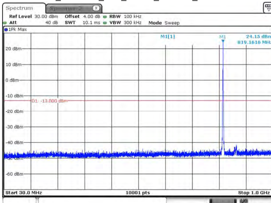
B26_CH26740_10M_1RB24_16-QAM_Below 1G
