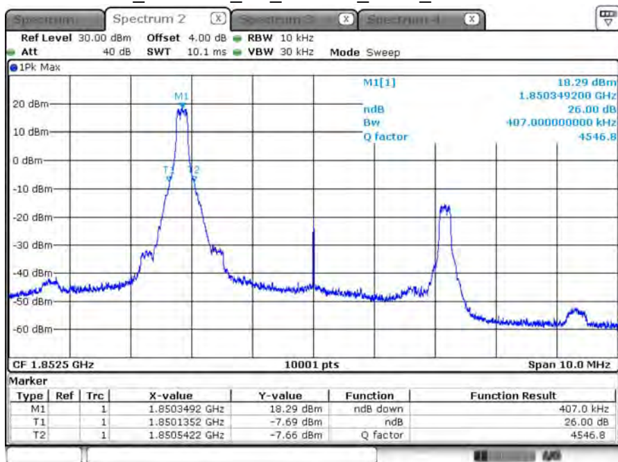
B2_CH18625_5M_16-QAM_1RB0_26dB BW
