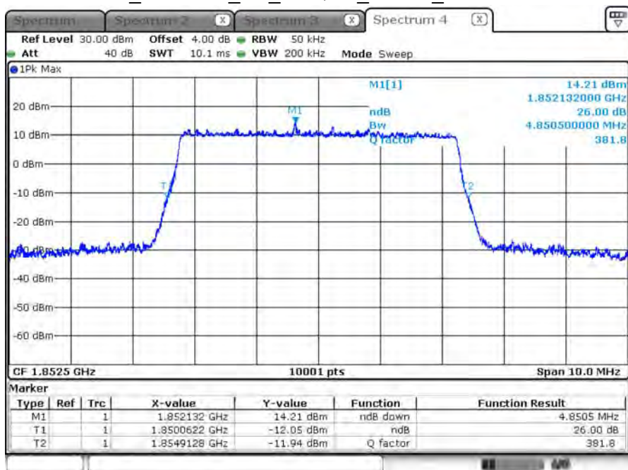
B2_CH18625_5M_16-QAM_25RB0_26dB BW
