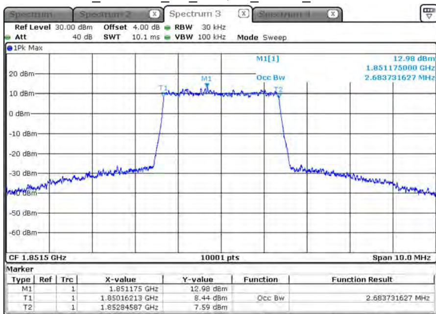
B2_CH18615_3M_16-QAM_15RB0_99% BW
