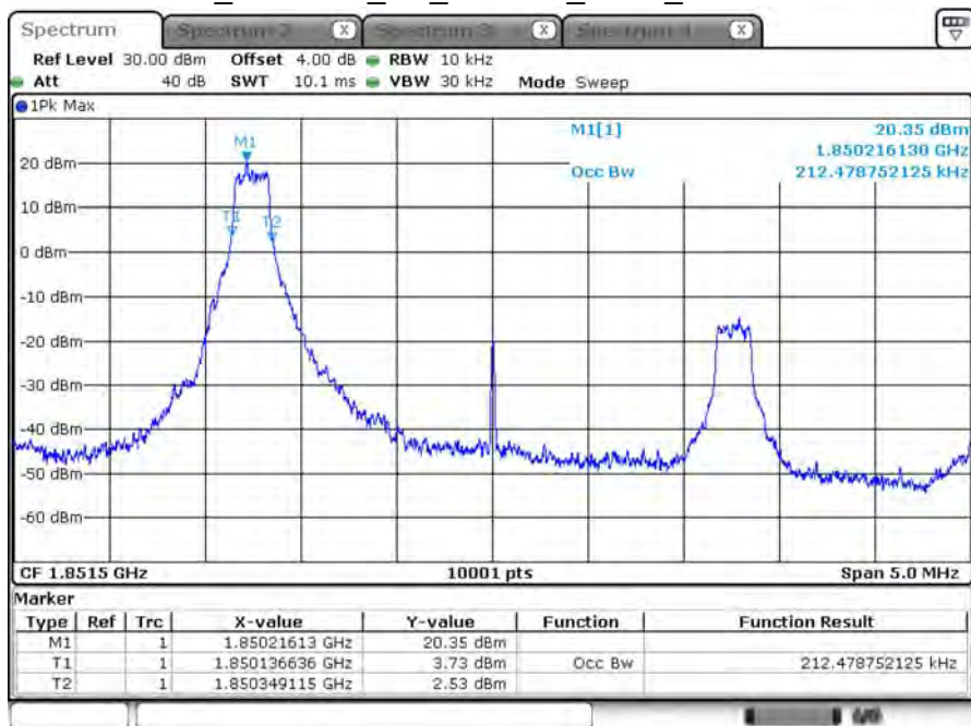
B2_CH18615_3M_16-QAM_1RB0_99% BW
