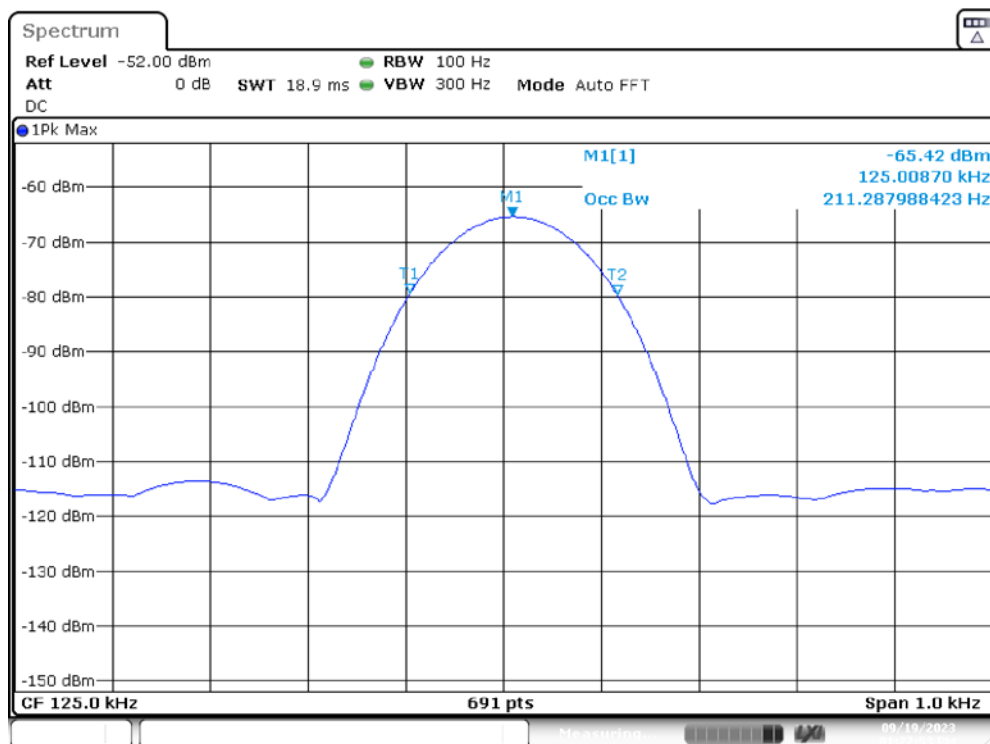
99% OBW Plot
