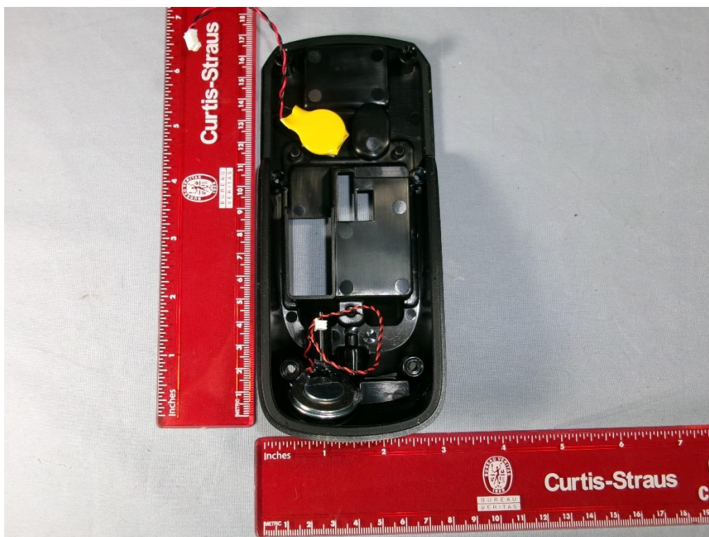
iDFace ASK Controller Inside Bottom Cover
