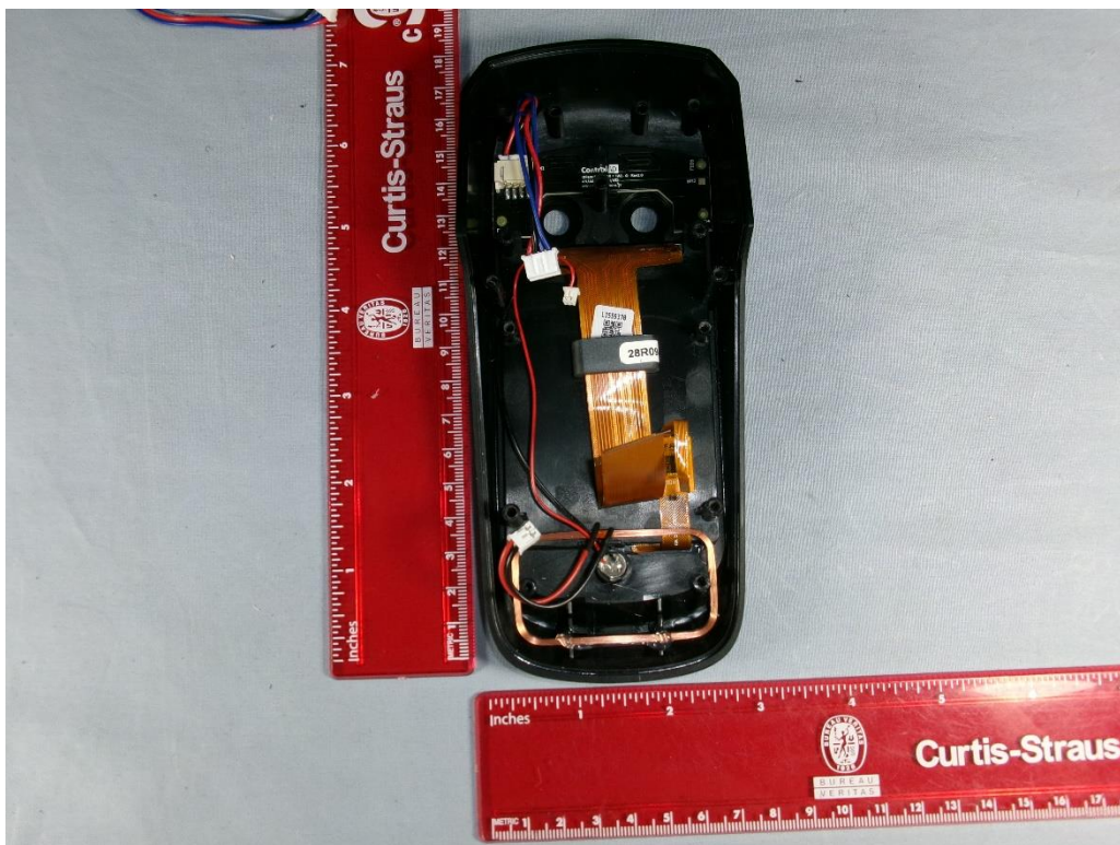
iDface ASK Controller Inside Top Cover
