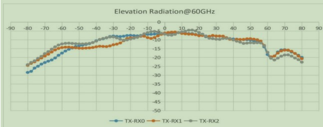
Figure 5-3 Antenna Elevation(YOZ) Radiation Pattern 1,2
