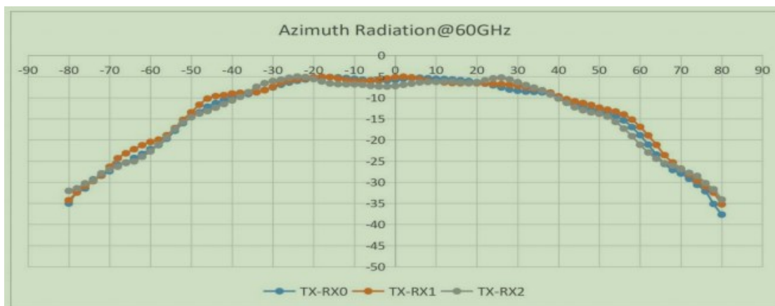
Figure 5-2 Antenna Azimuth(XOZ) Radiation Pattern 1,2
