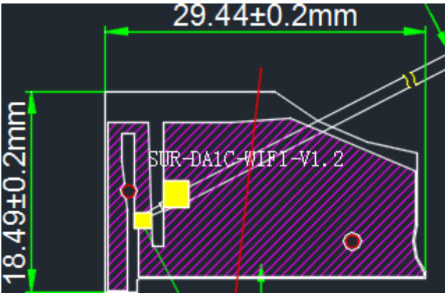
WiFi antenna
