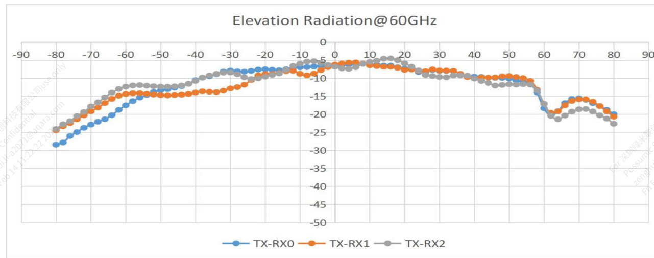
Figure 5-3 Antenna Elevation(YOZ) Radiation Pattern 1,2
