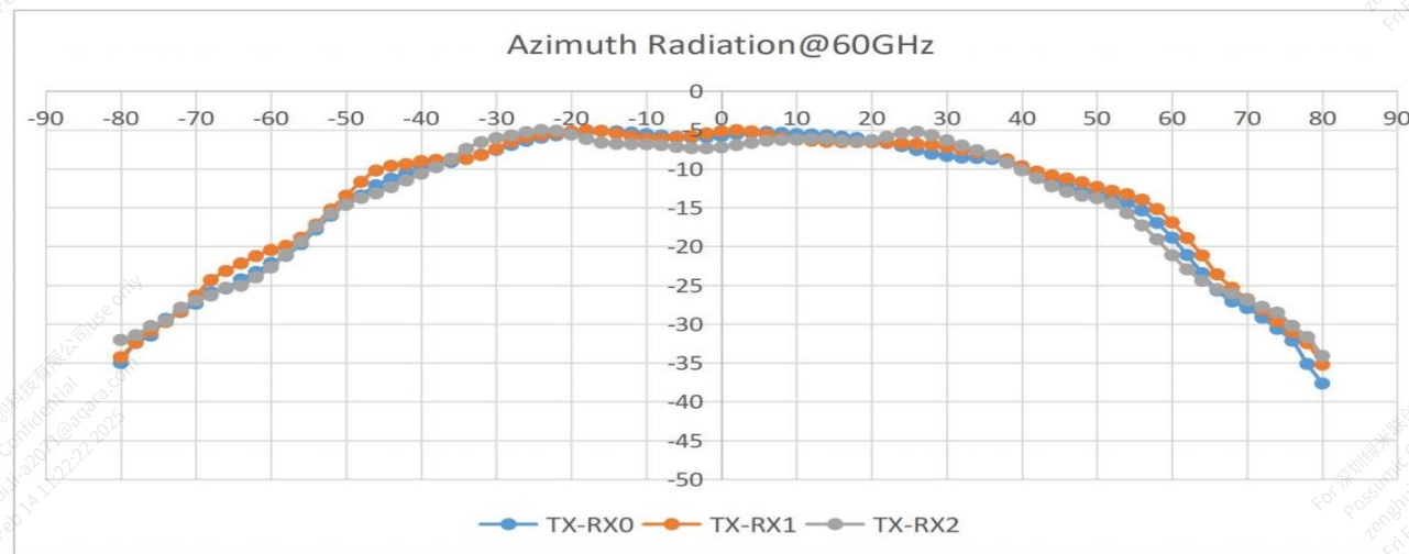
Figure 5-2 Antenna Azimuth(XOZ) Radiation Pattern 1,2
