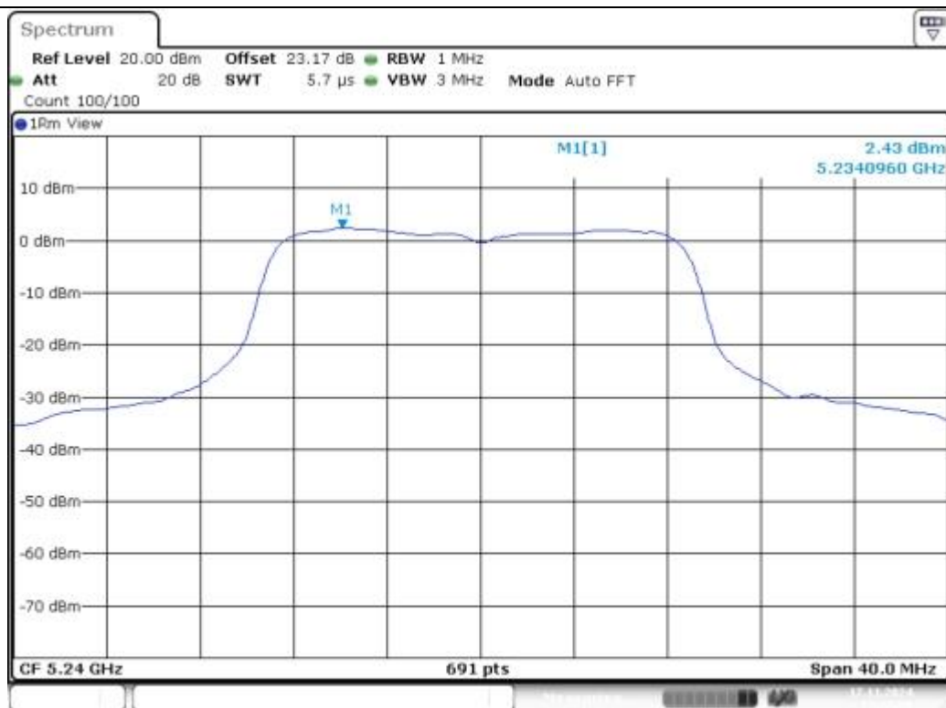
11N20SISO-Ant1-5240-PASS
