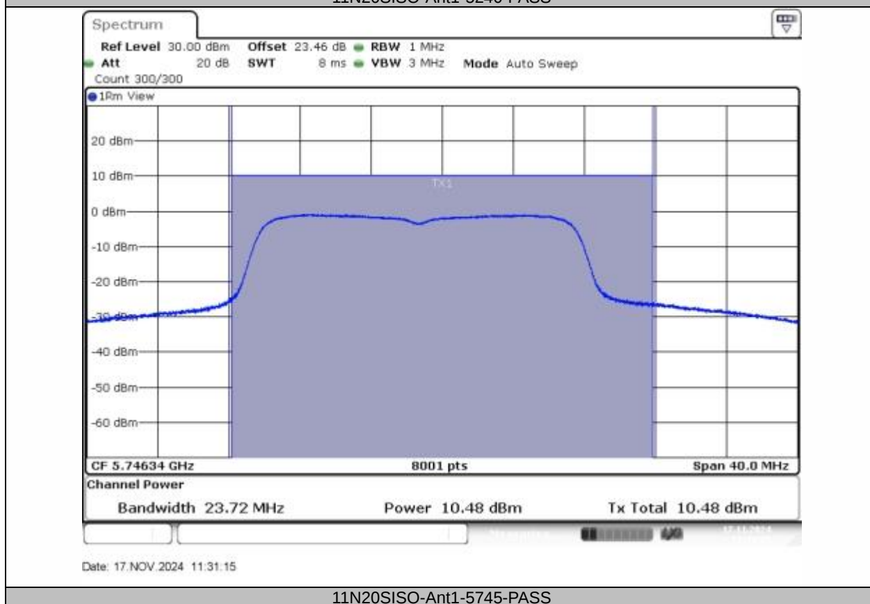
11N20SISO-Ant1-5745-PASS
