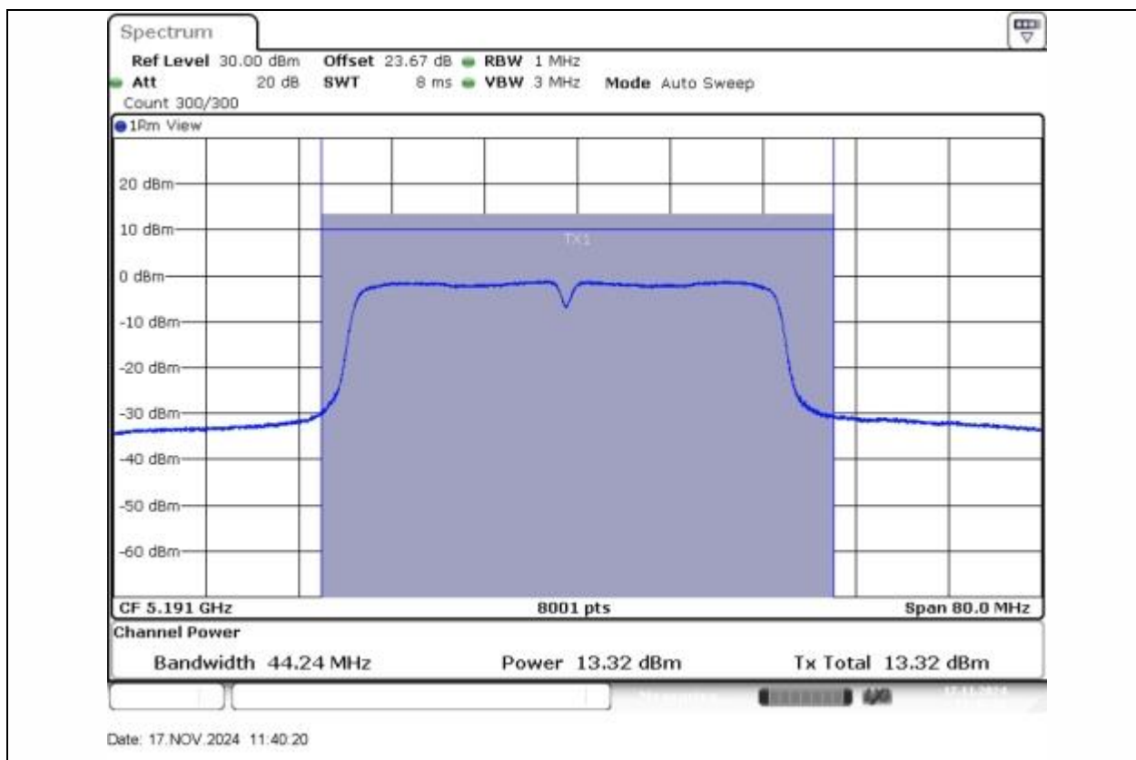
11N40SISO-Ant1-5190-PASS
