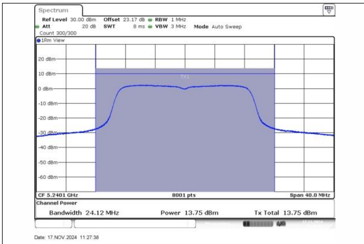
11N20SISO-Ant1-5240-PASS
