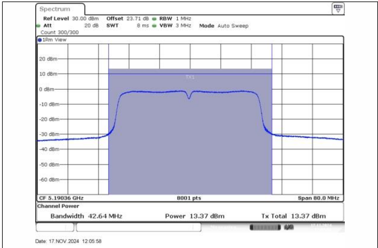
11AC40SISO-Ant1-5190-PASS
