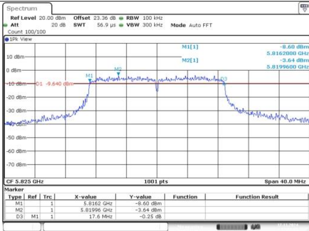
11AC20SISO-Ant1-5825-PASS
