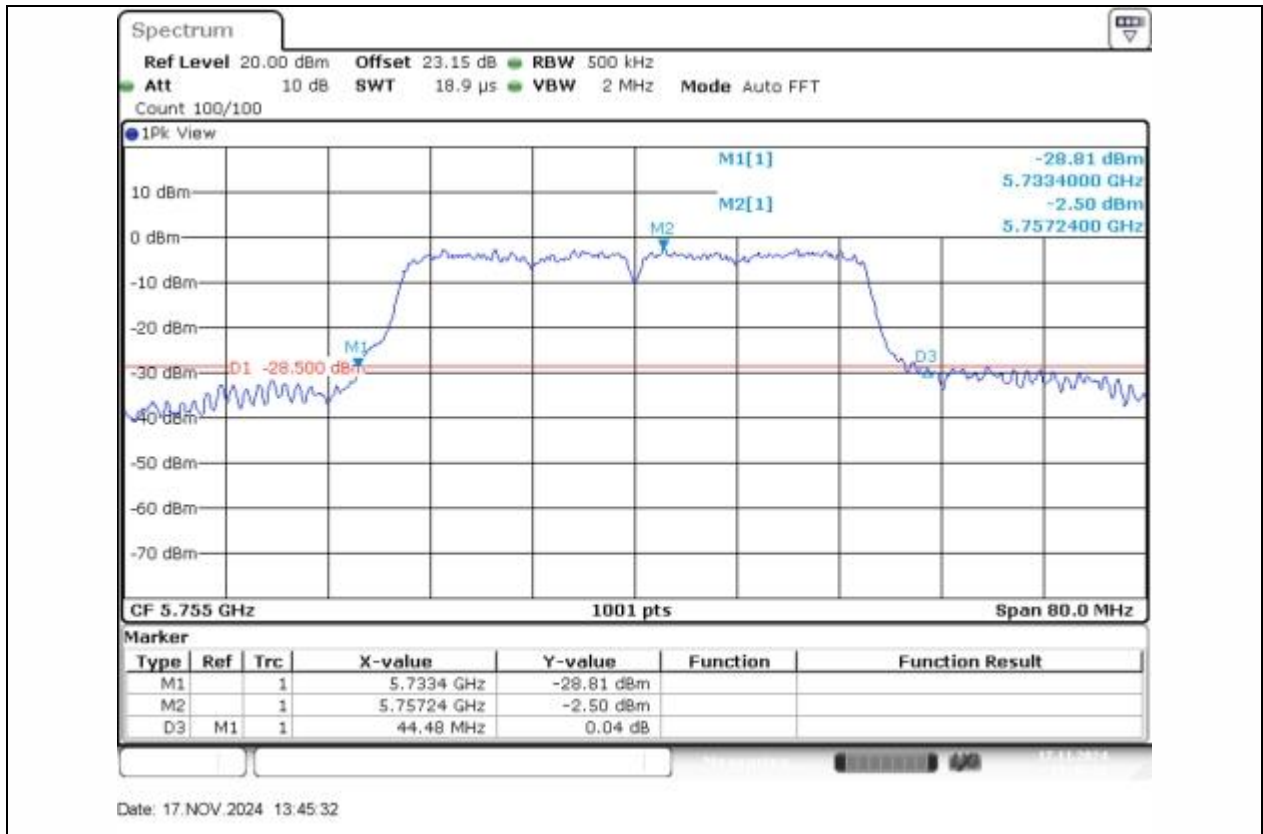
11AC40SISO-Ant1-5755
