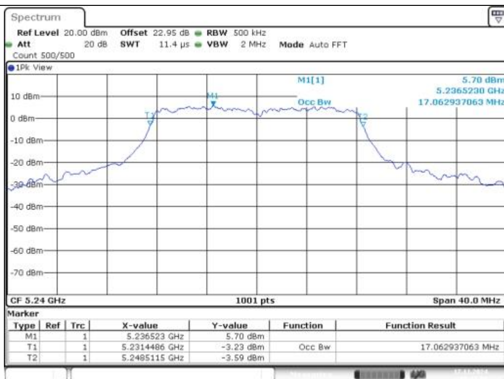
11A-Ant1-5240
