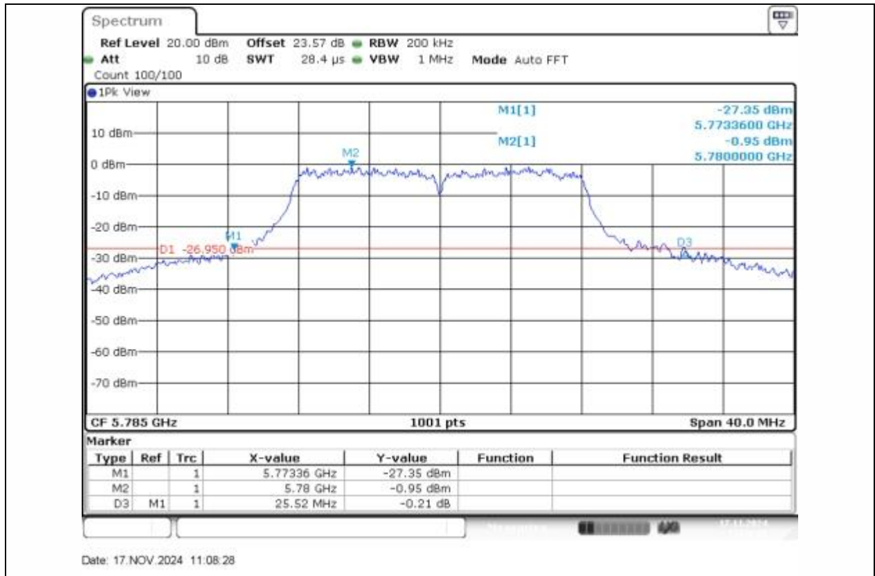
11A-Ant1-5785
