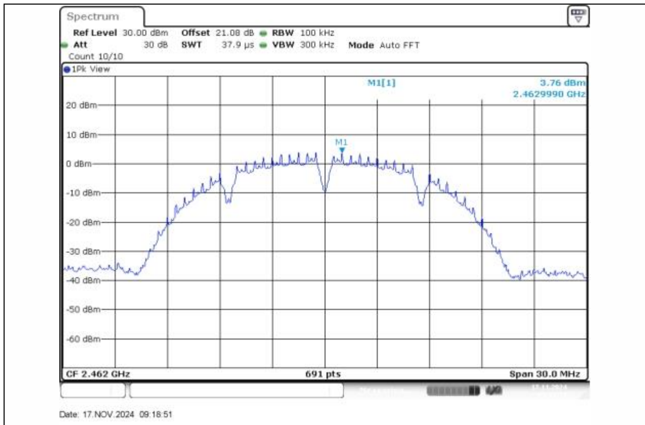
11B-Ant1-2462-0~Reference-PASS
