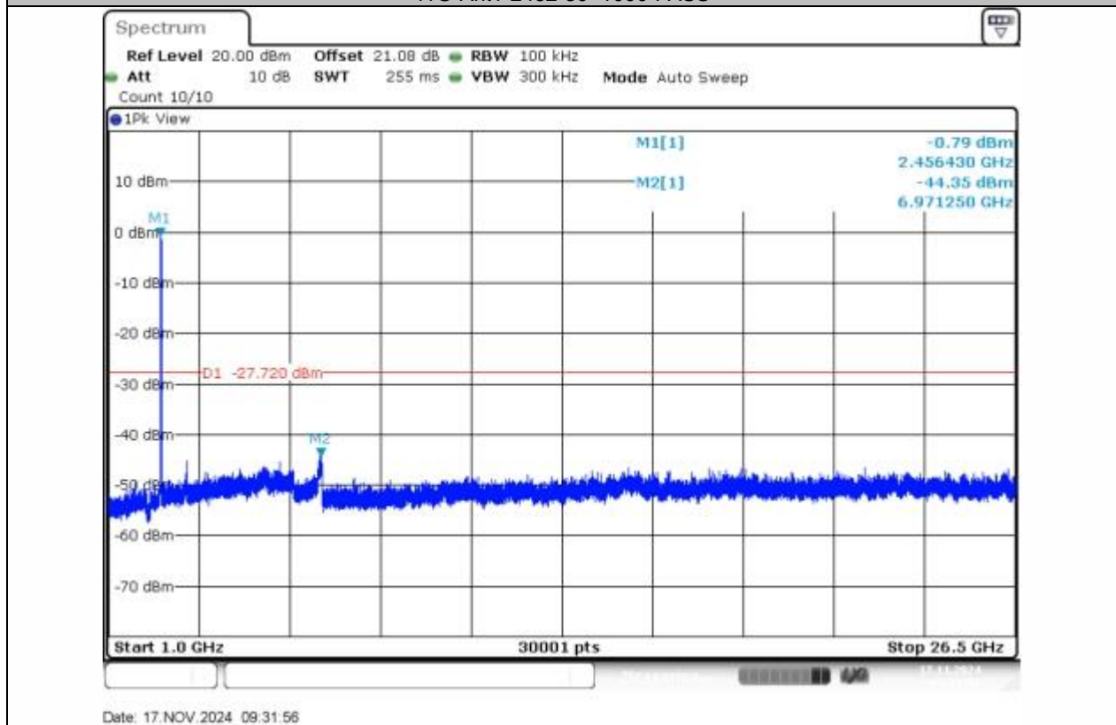
11G-Ant1-2462-1000~26500-PASS
