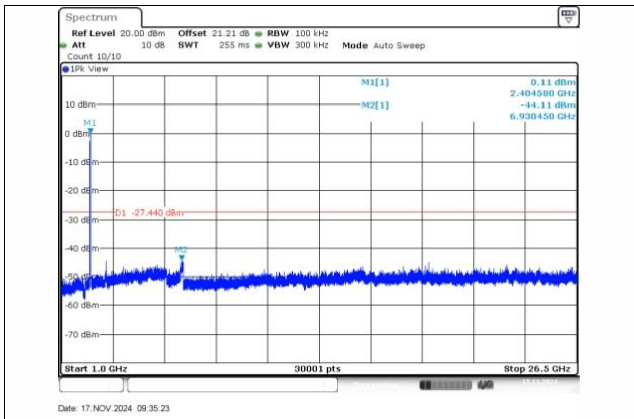
11N20SISO-Ant1-2412-1000~26500-PASS
