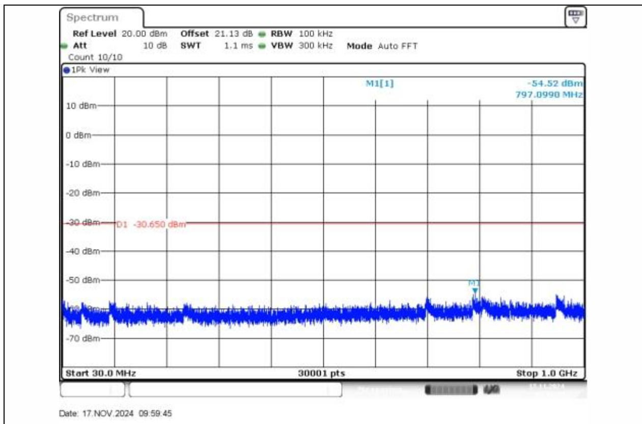
11N40SISO-Ant1-2452-30~1000-PASS
