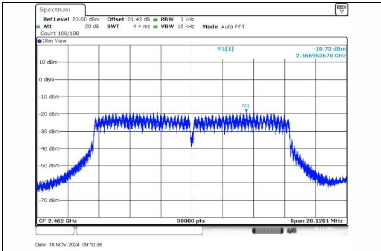
11N20SISO-Ant1-2462-PASS
