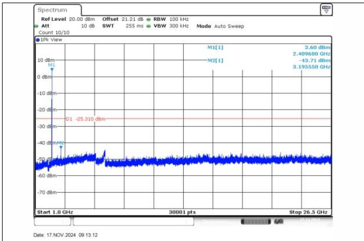
11B-Ant1-2412-1000~26500-PASS
