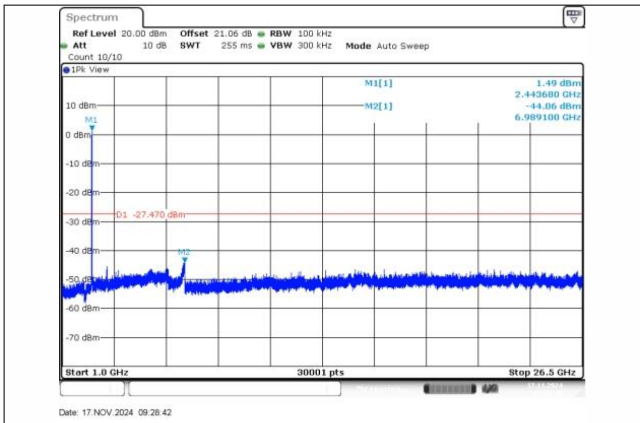
11G-Ant1-2437-1000~26500-PASS
