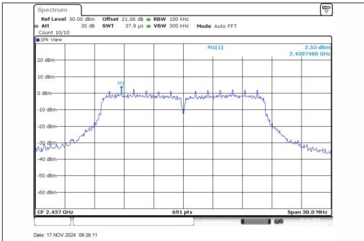
11G-Ant1-2437-0~Reference-PASS
