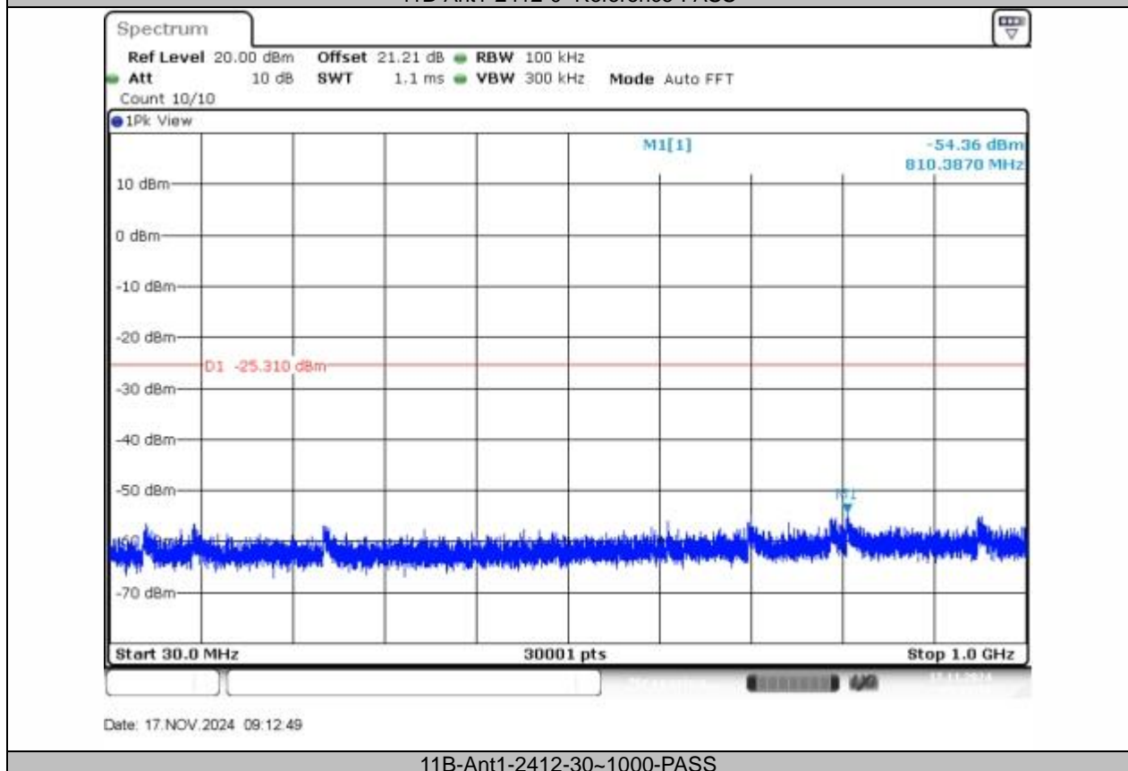
11B-Ant1-2412-30~1000-PASS
