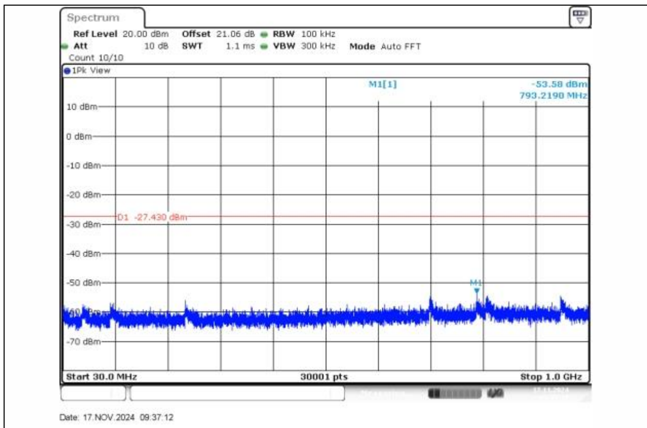
11N20SISO-Ant1-2437-30~1000-PASS
