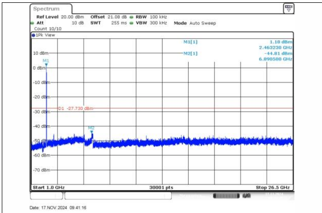
11N20SISO-Ant1-2462-1000~26500-PASS
