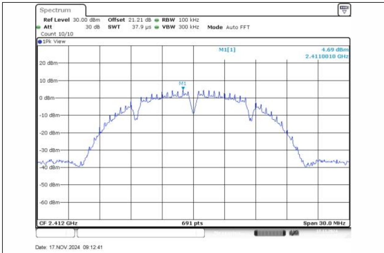
11B-Ant1-2412-0~Reference-PASS
