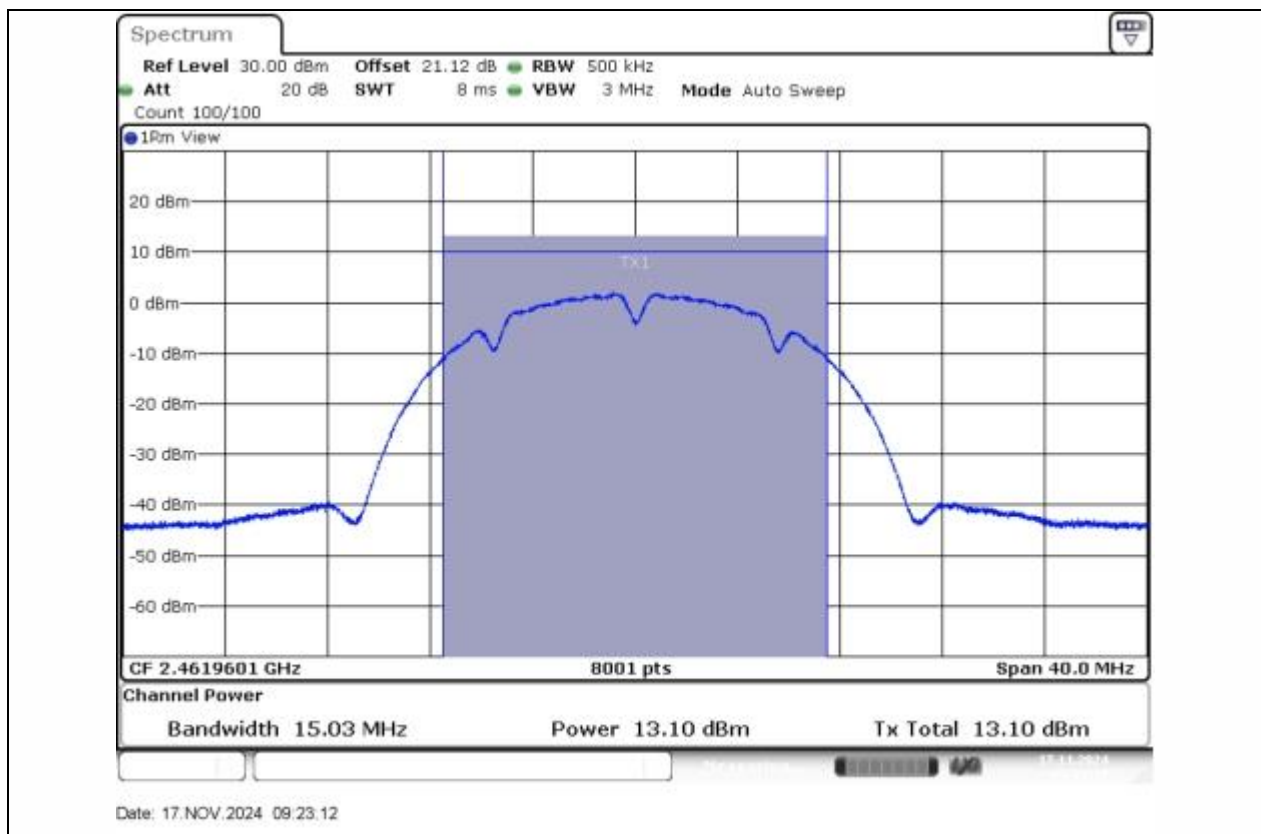
11B-Ant1-2462-PASS
