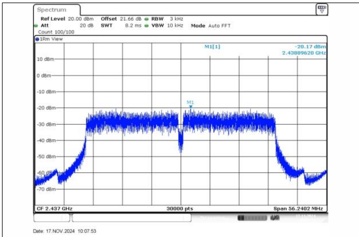
11N40SISO-Ant1-2437-PASS
