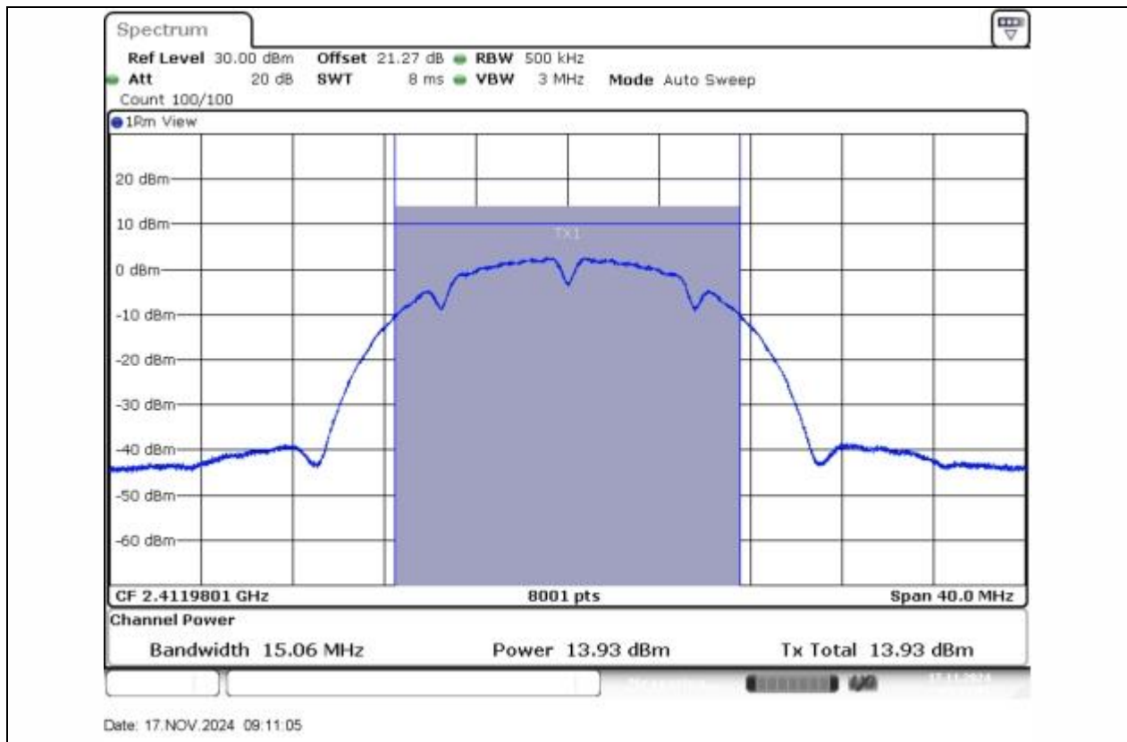
11B-Ant1-2412-PASS
