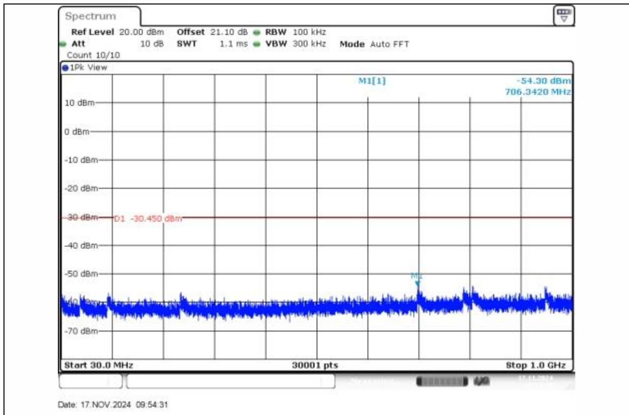
11N40SISO-Ant1-2422-30~1000-PASS
