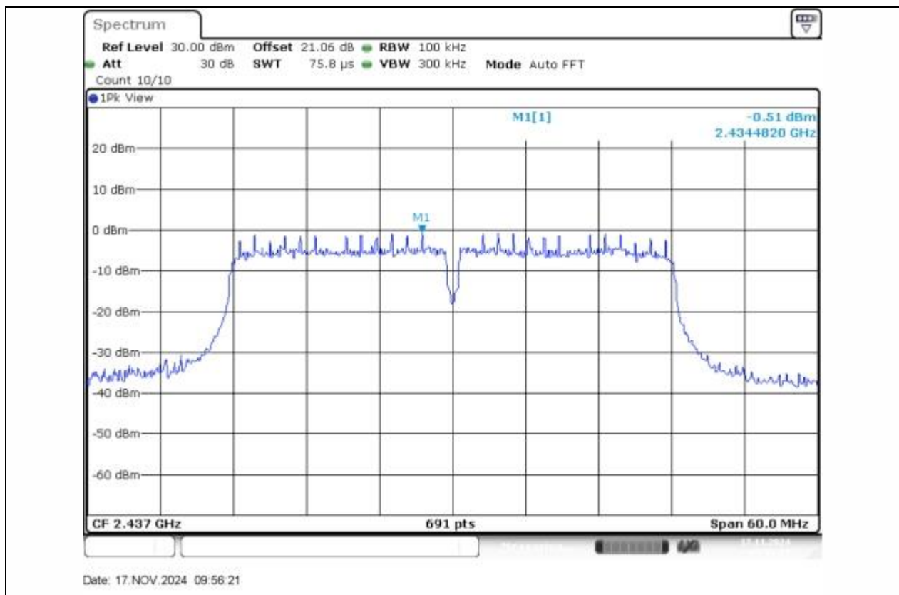
11N40SISO-Ant1-2437-0~Reference-PASS
