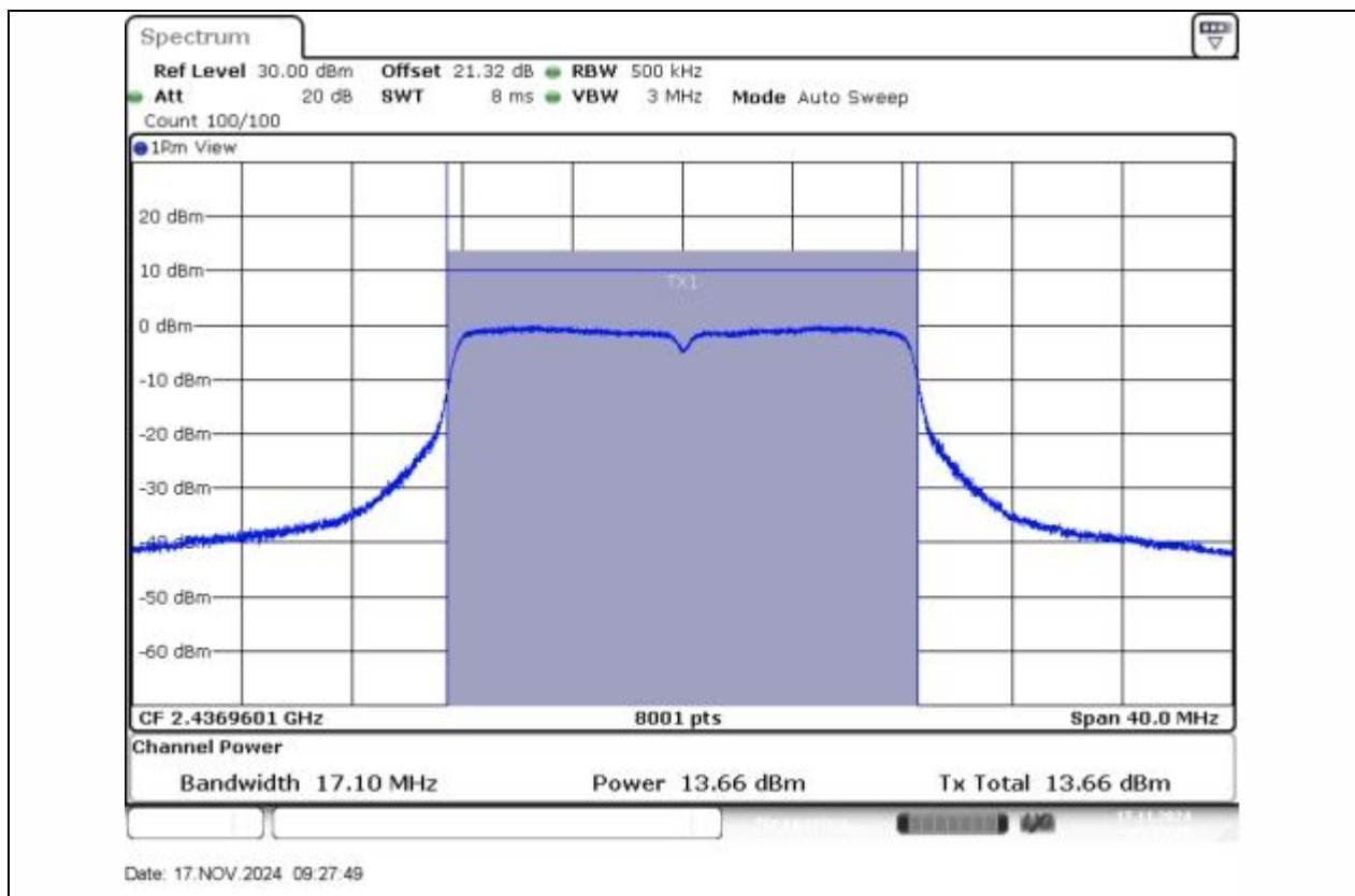
11G-Ant1-2437-PASS
