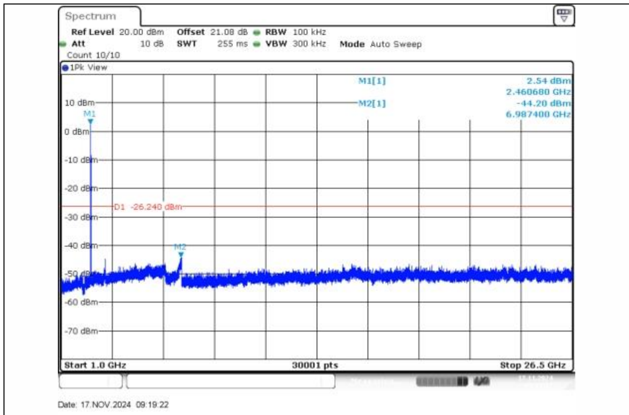
11B-Ant1-2462-1000~26500-PASS
