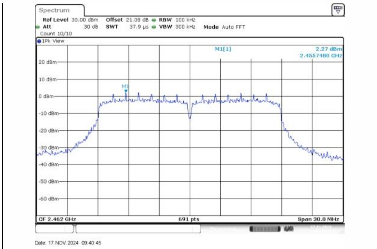
11N20SISO-Ant1-2462-0~Reference-PASS
