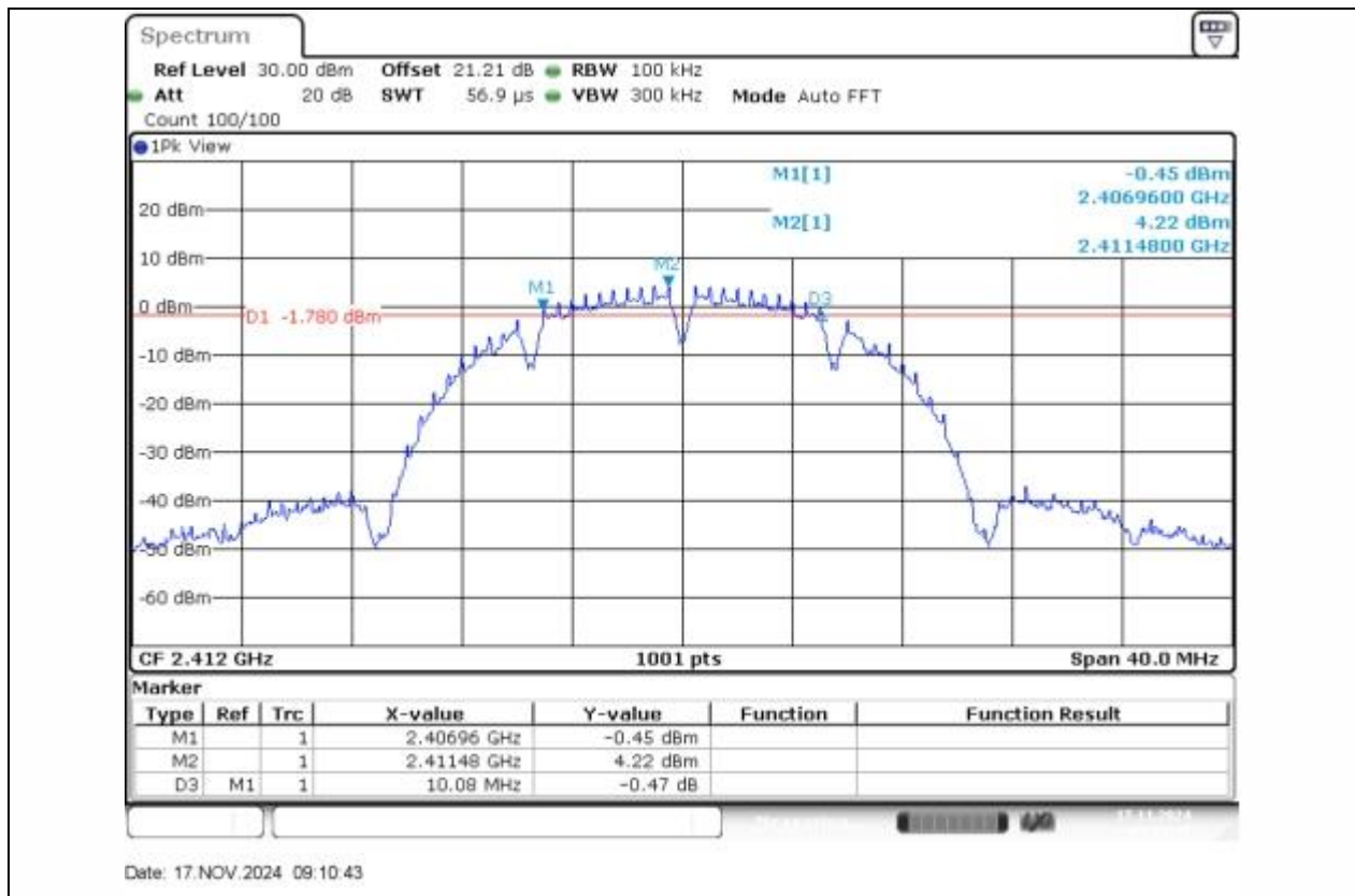
11B-Ant1-2412-PASS
