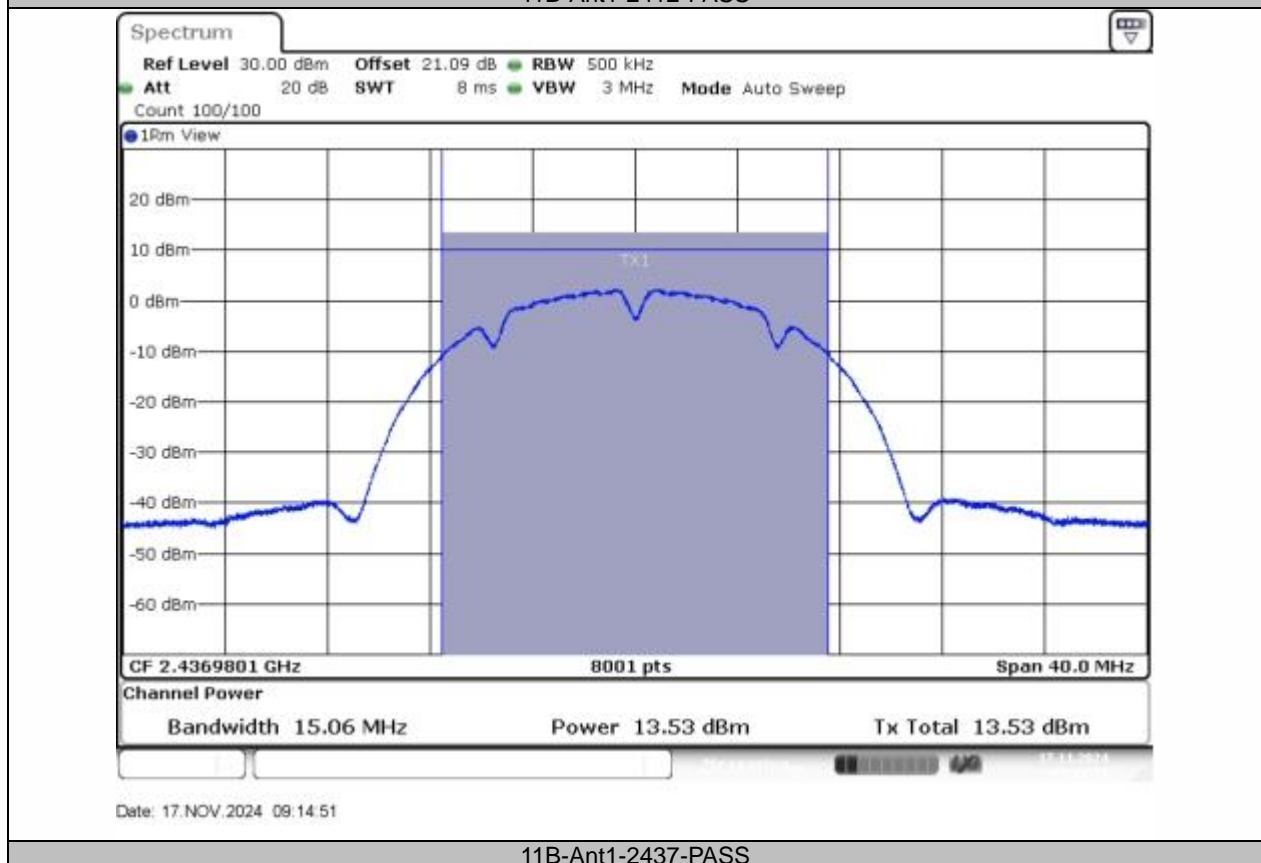
11B-Ant1-2437-PASS
