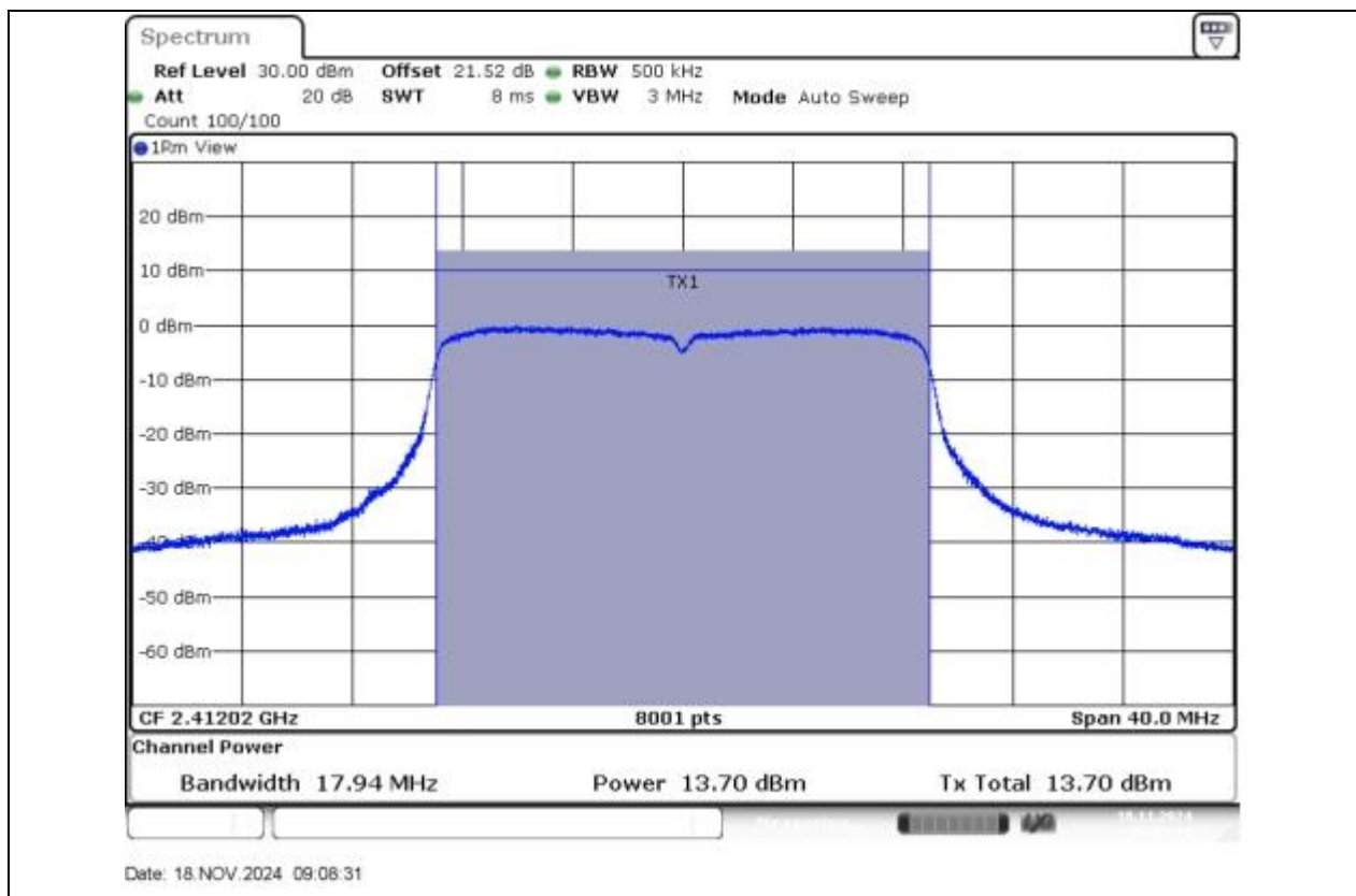
11N20SISO-Ant1-2412-PASS
