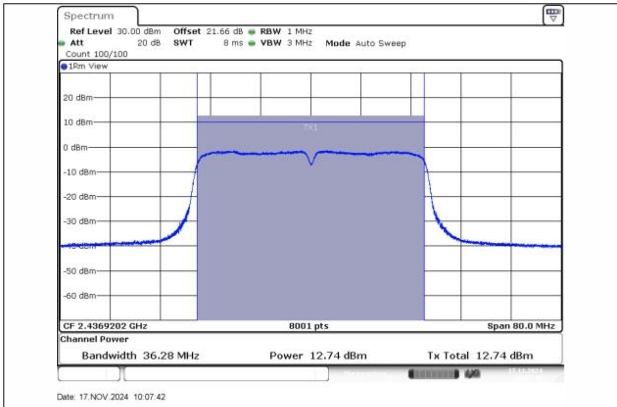
11N40SISO-Ant1-2437-PASS
