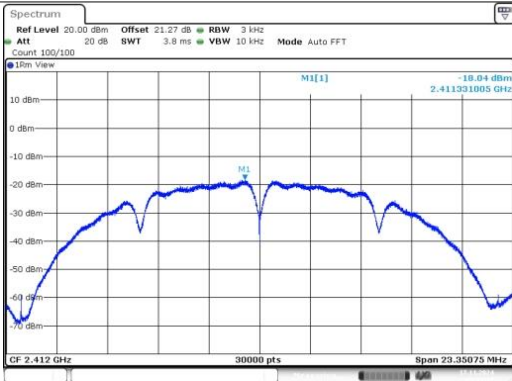
11B-Ant1-2412-PASS
