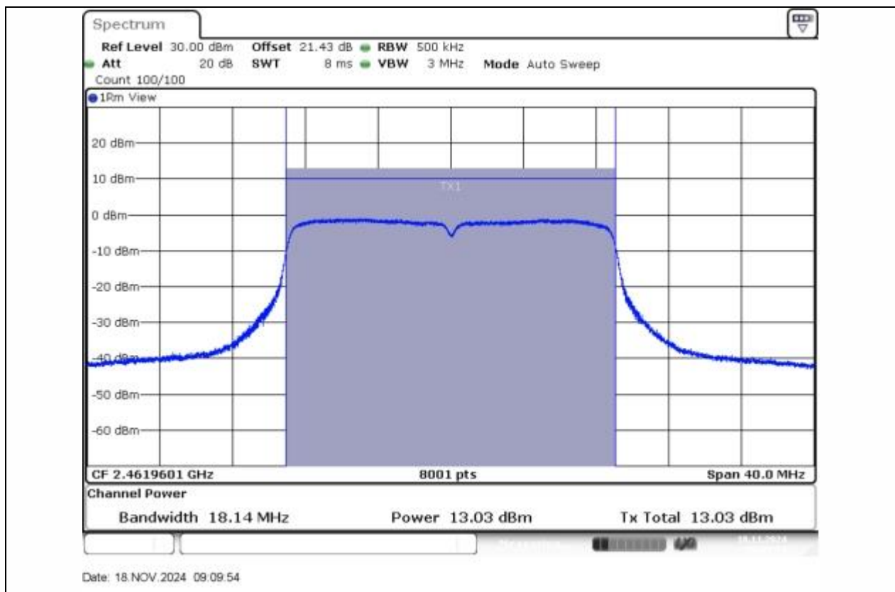
11N20SISO-Ant1-2462-PASS
