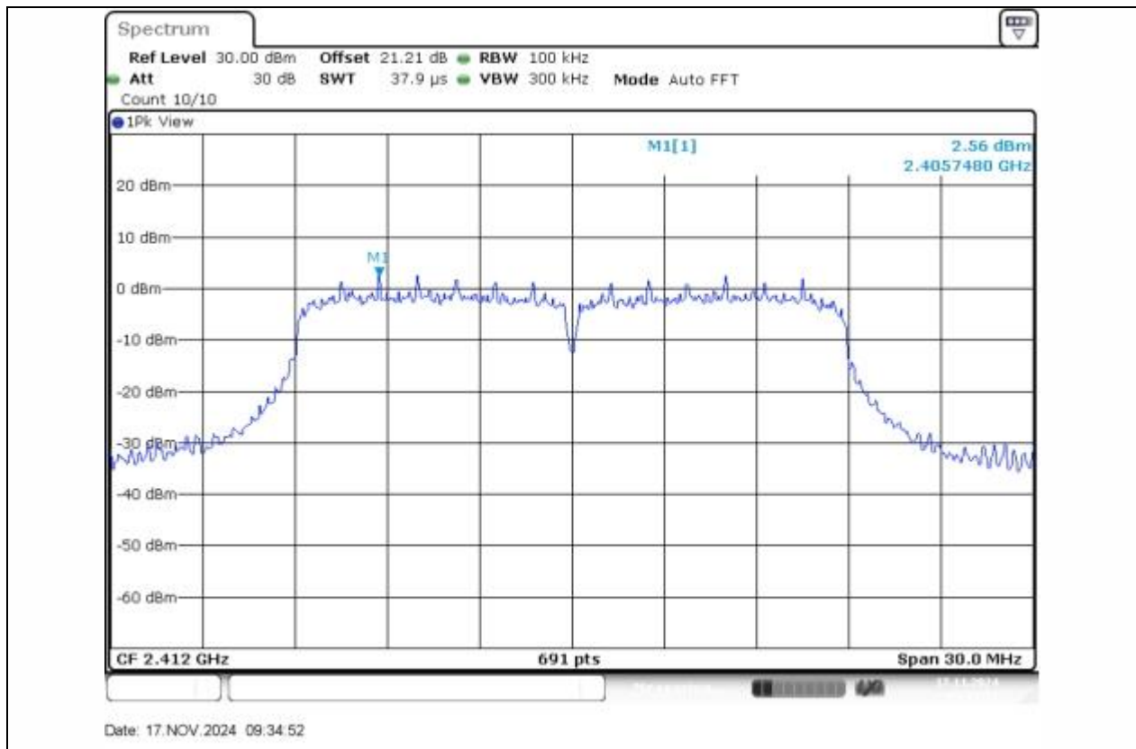
11N20SISO-Ant1-2412-0~Reference-PASS
