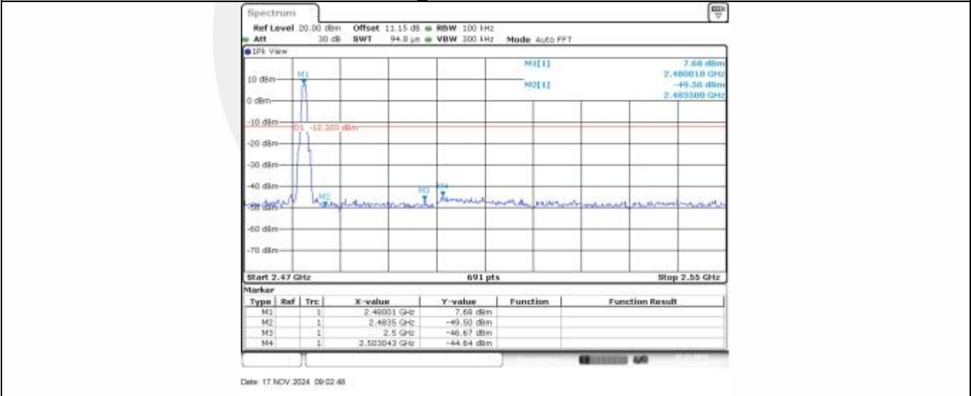
BLE_1M-Ant1-2480-PASS
