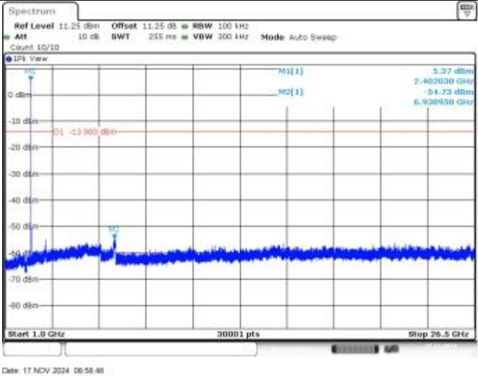
BLE_1M-Ant1-2402-1000-26500-PASS
