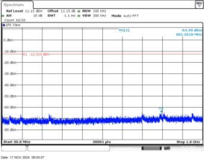
BLE_1M-Ant1-2480-30~1000-PASS
