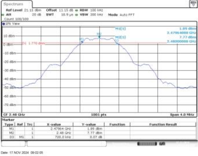
BLE_1M-Ant1-2480-PASS
