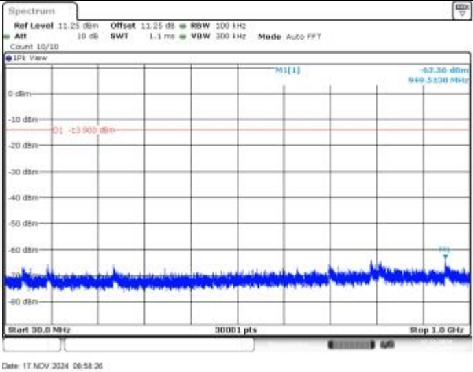
BLE_1M-Ant1-2402-30-1000-PASS
