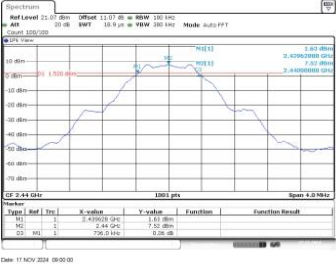
BLE_1M-Ant1-2440-PASS
