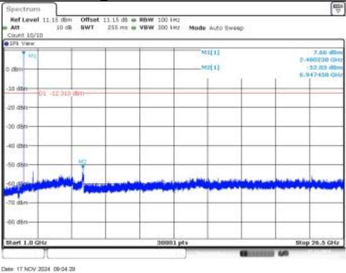
BLE_1M-Ant1-2480-1000~26500-PASS
