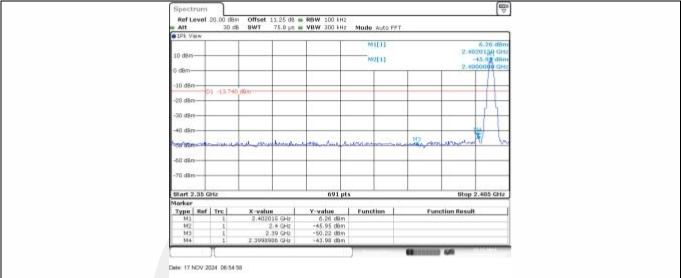
BLE_1M-Ant1-2402-PASS
