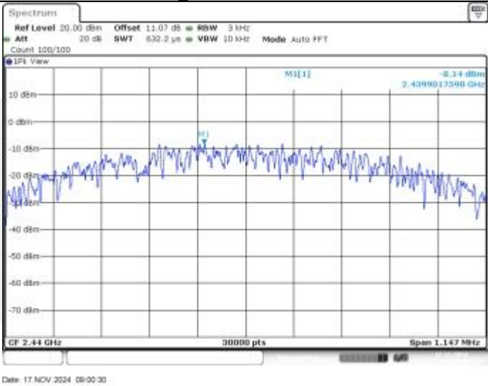
BLE_1M-Ant1-2440-PASS
