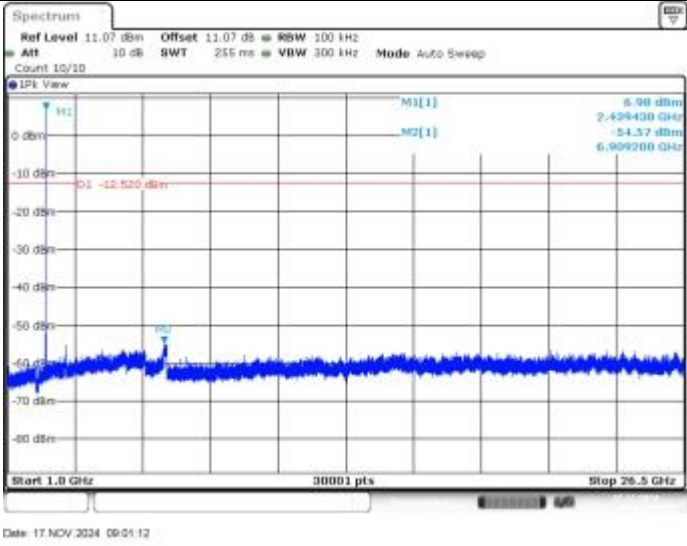
BLE_1M-Ant1-2440-1000~26500-PASS
