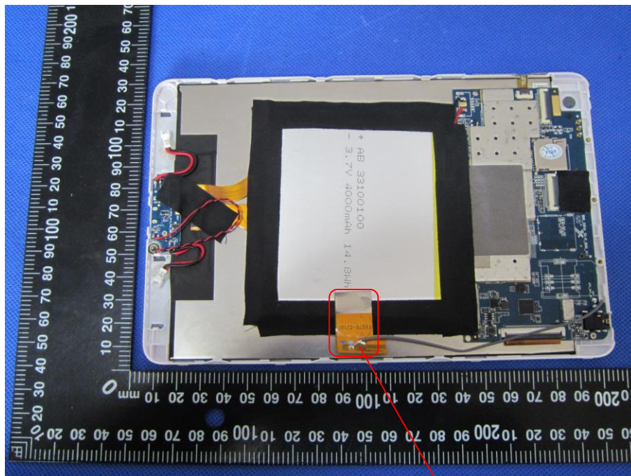
Wi-Fi/BT/GPS Ant.
