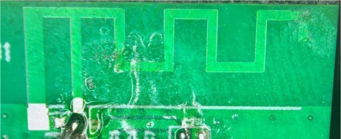
Antenna physical object and physical dimensions
