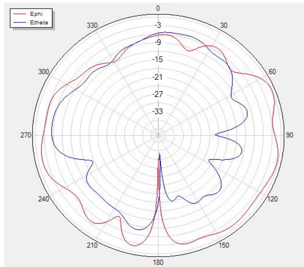
Phi=90 freq=2440MHz
