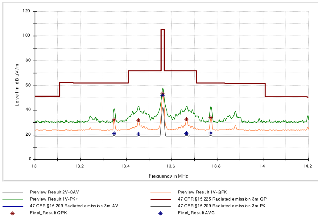
Figure 12: Chart of emission within the band 13.110 MHz to 14.010 MHz, with tag, position 2, antenna in line at 3m distance
