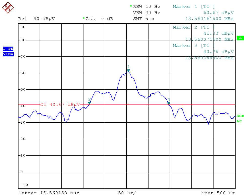
Figure 10: Chart of 20 dB bandwidth tests
