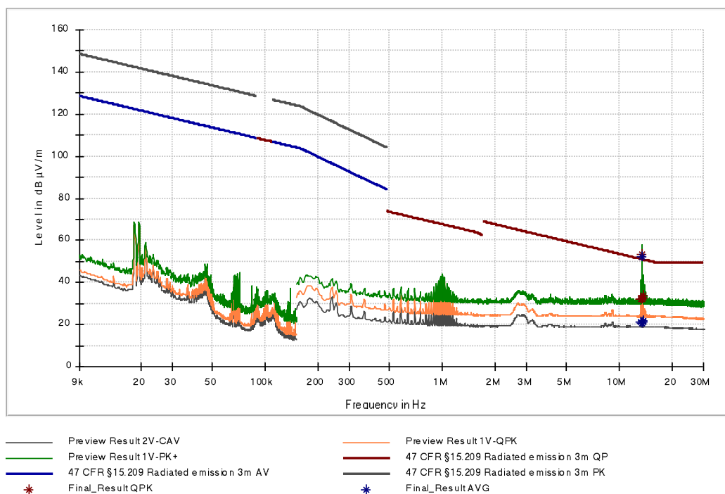
Figure 13: Chart of emissions test below 30 MHz with tag in position 2, antenna in line at 3 m
