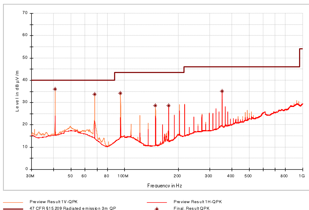
Figure 14: Chart of emissions test from 30 MHz to 1 GHz with tag in position 3 at 3 m
