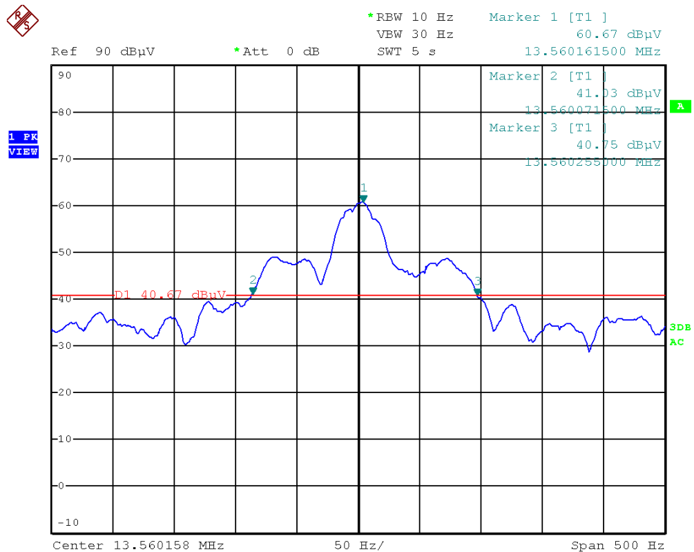
Figure 10: Chart of 20 dB bandwidth tests
