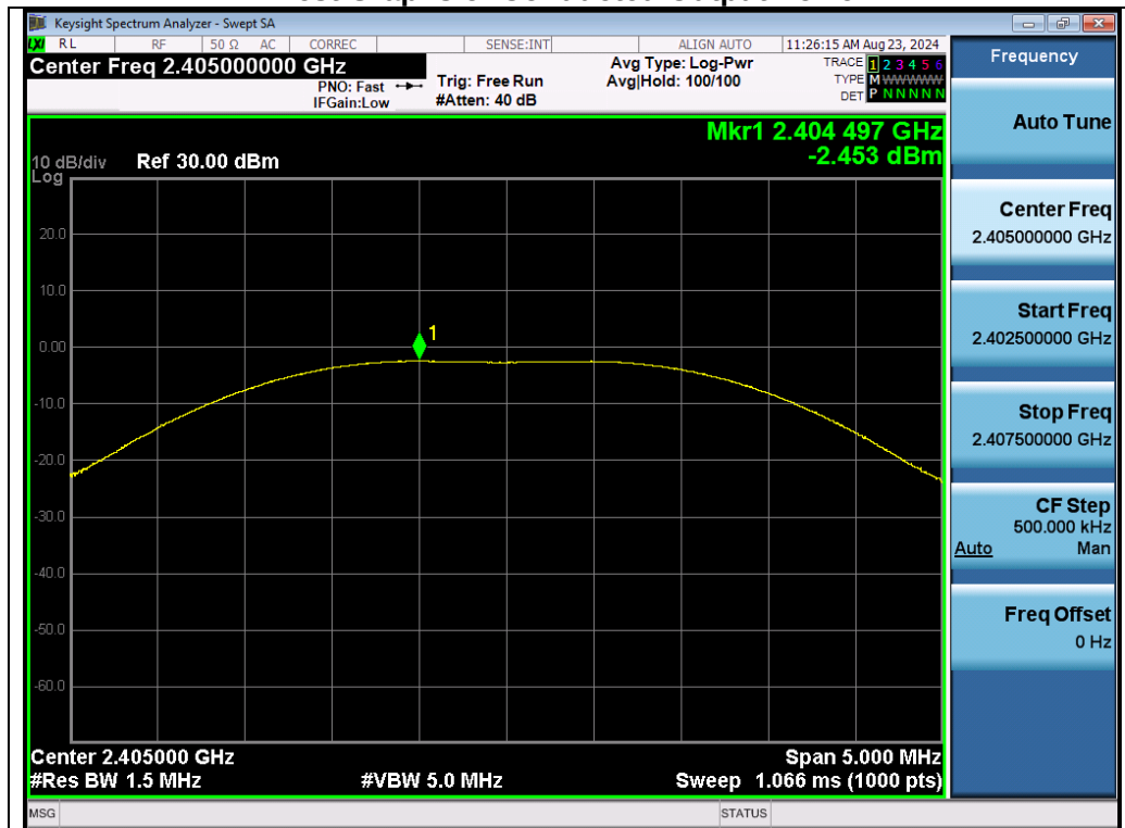
Test_Graph_2.4G_ANT1_2405_Peak Power
