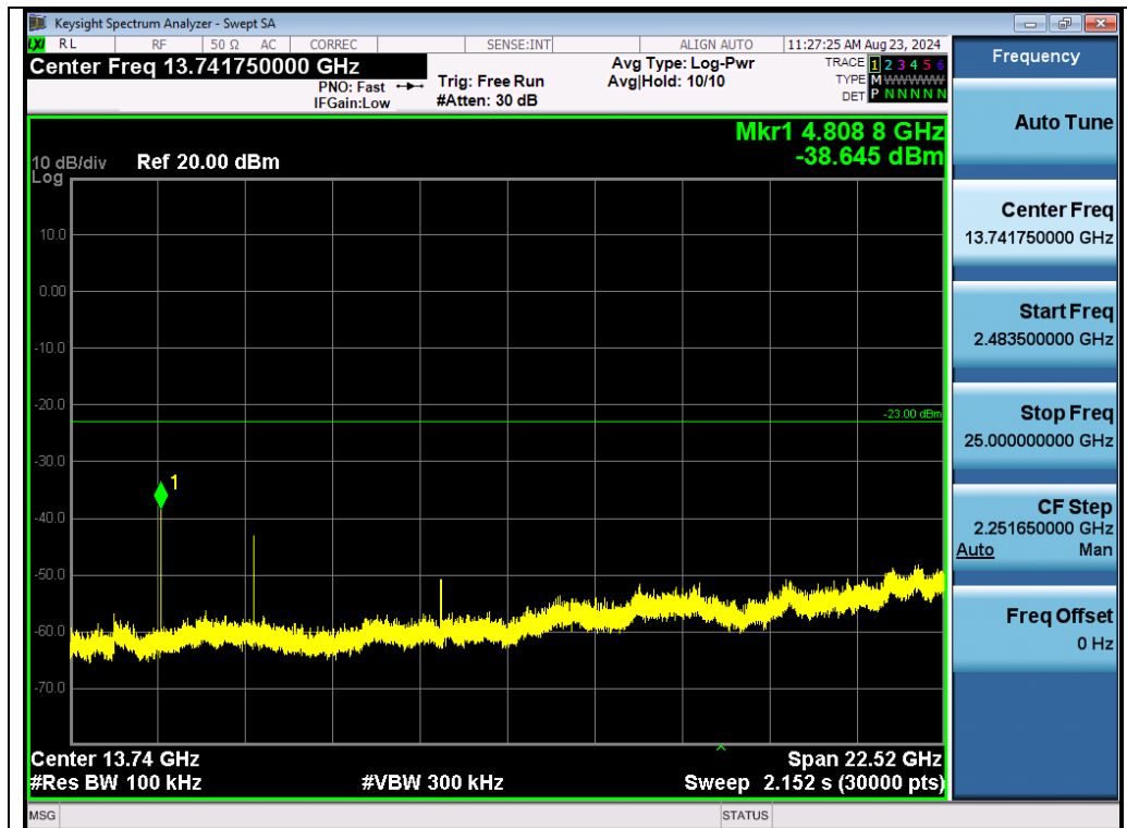
Test_Graph_2.4G_ANT1_2405_Higher Band Emissions
