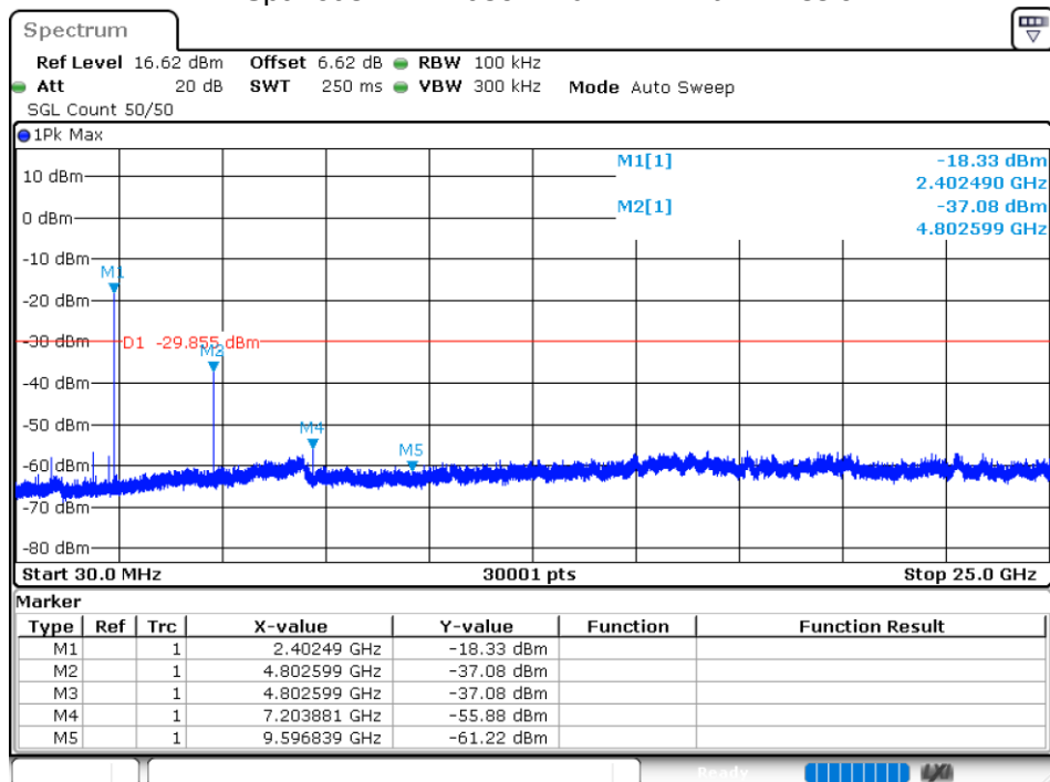
Tx. Spurious NVNT user 2402MHz Ant1 Emission
