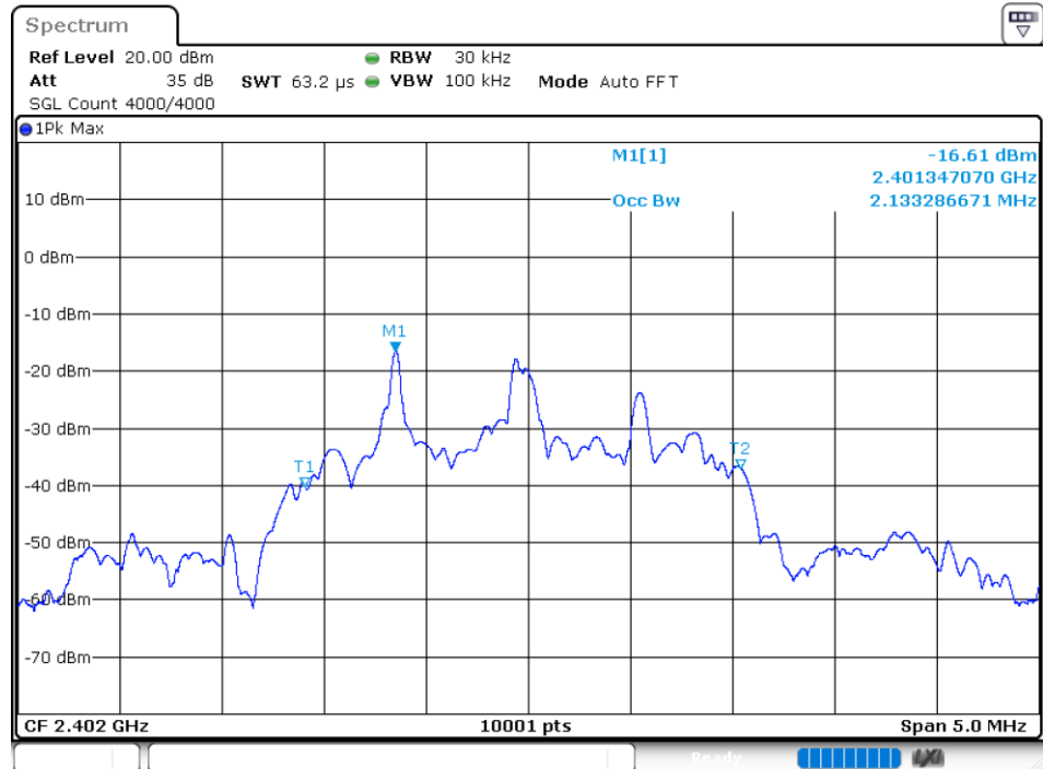
OBW NVNT user 2402MHz Ant1
