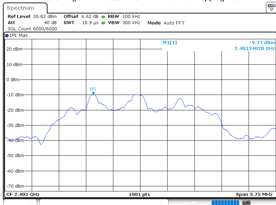
Band Edge NVNT user 2402MHz Ant1 No-Hopping Ref
