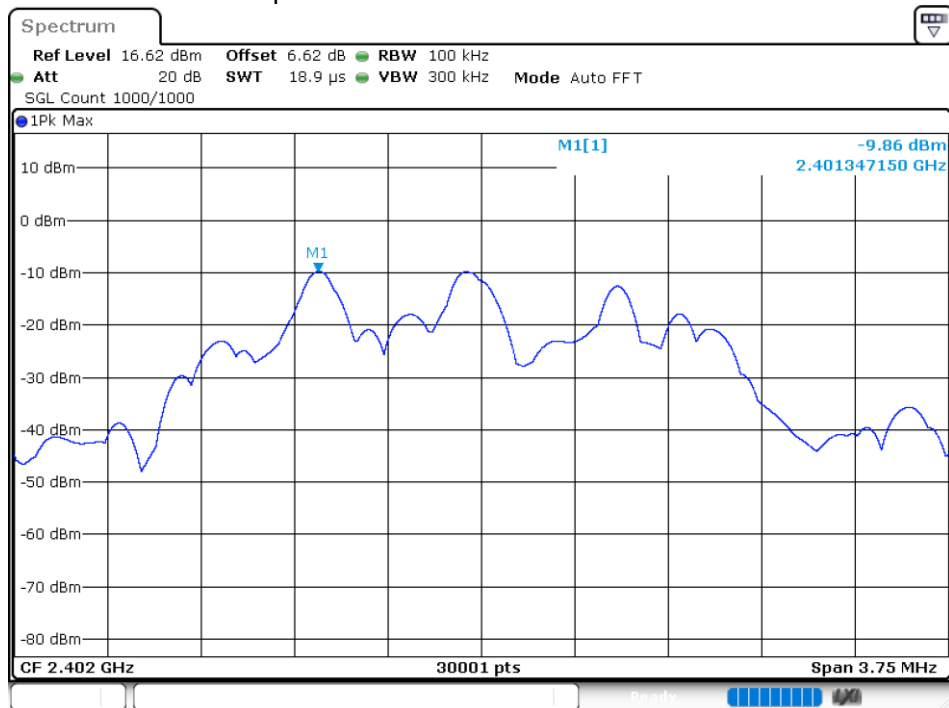
Tx. Spurious NVNT user 2402MHz Ant1 Ref
