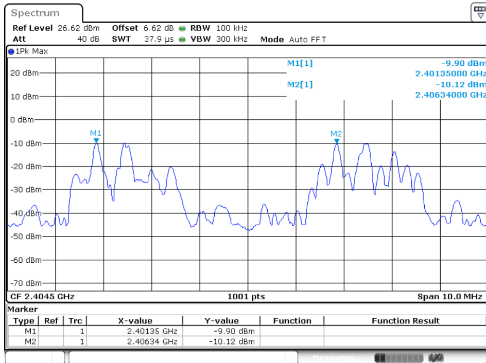
CFS NVNT user 2402MHz
