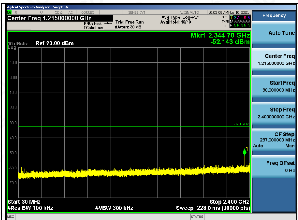
Test_Graph_ANT1_2441.85_Lower Band Emissions
