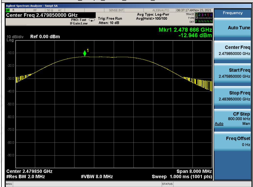
Test_Graph_ANT1_2479.85_Peak Power
