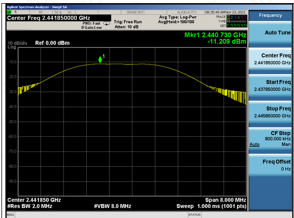
Test_Graph_ANT1_2441.85_Peak Power
