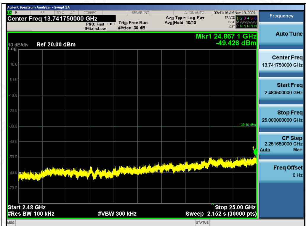
Test_Graph_ANT1_2403.85_Higher Band Emissions
