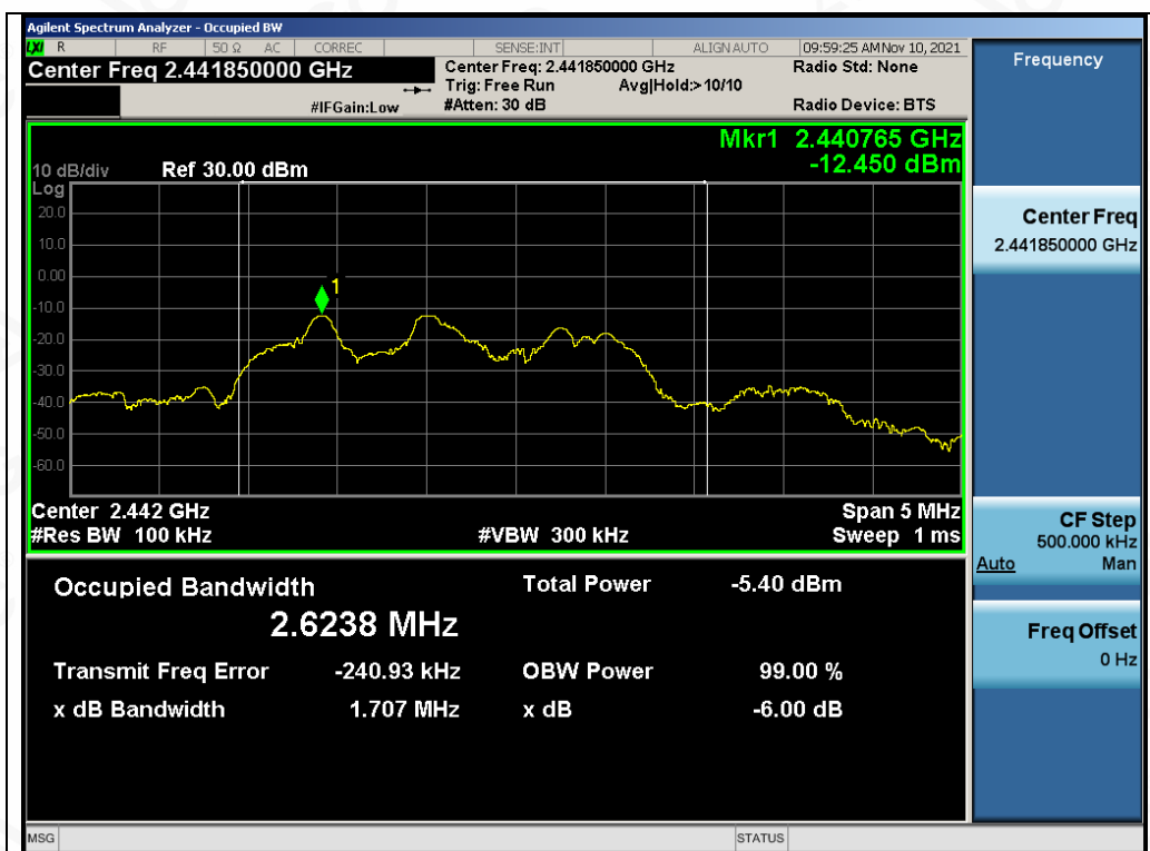
Test_Graph_ANT1_2441.85_DTSBW
