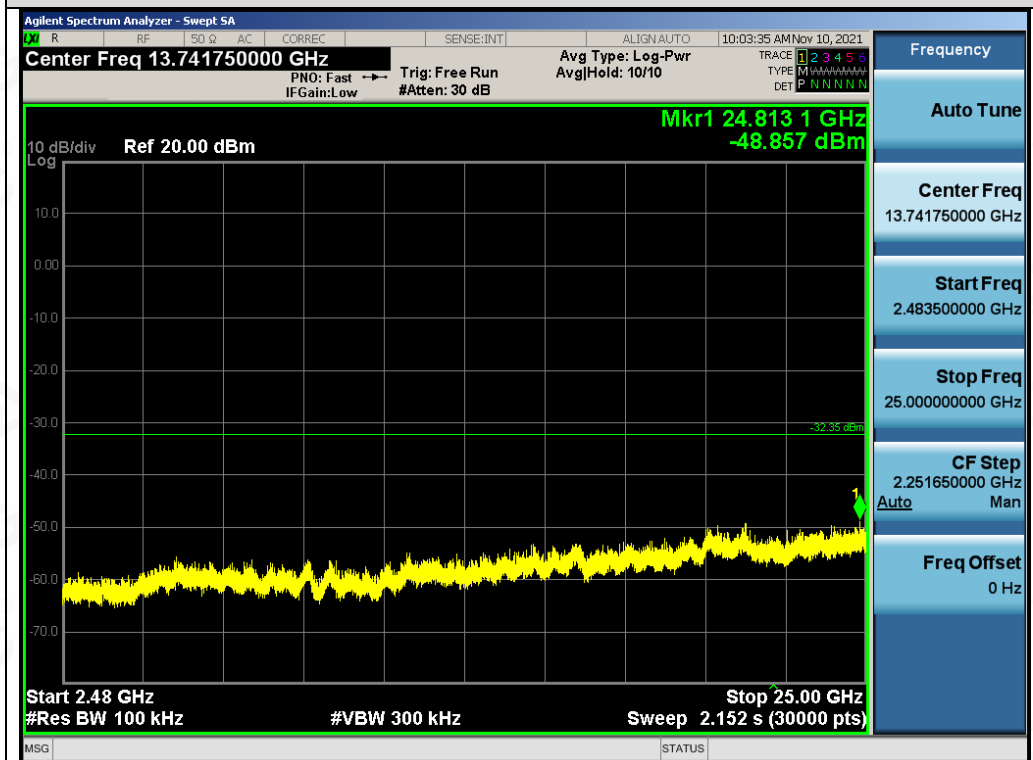
Test_Graph_ANT1_2441.85_Higher Band Emissions
