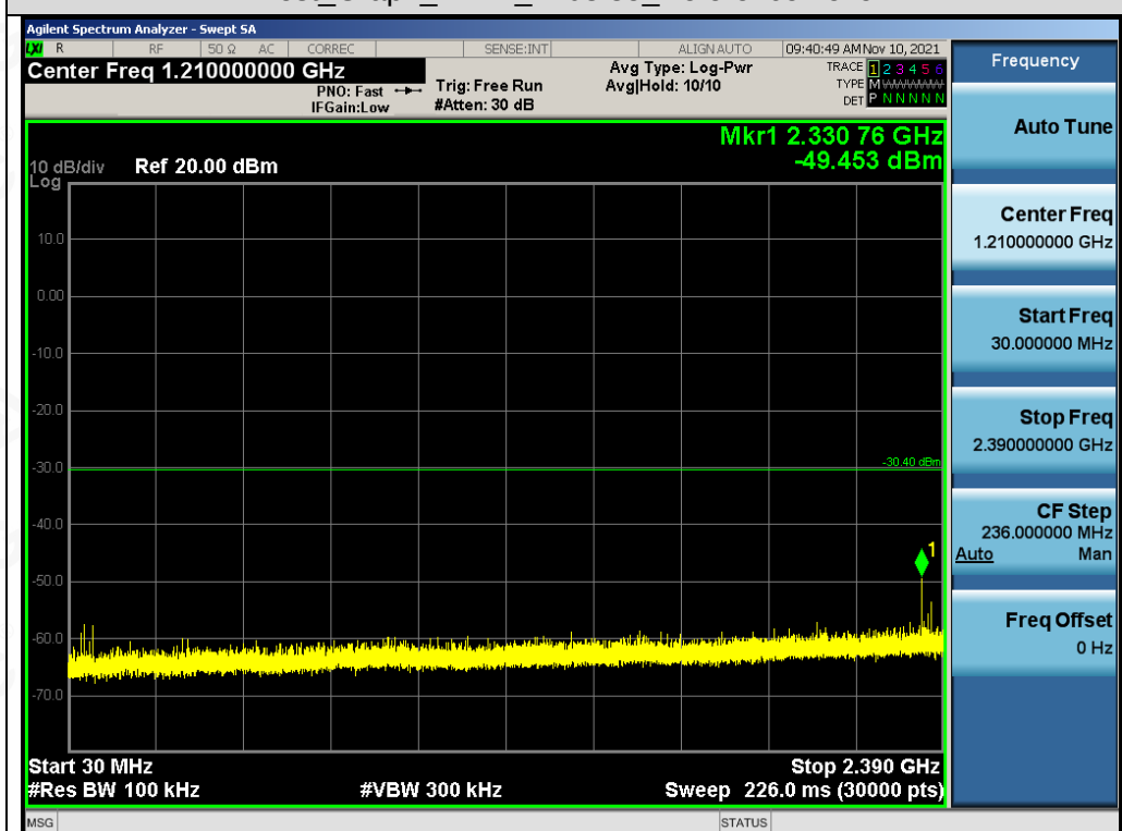
Test_Graph_ANT1_2403.85_Lower Band Emissions
