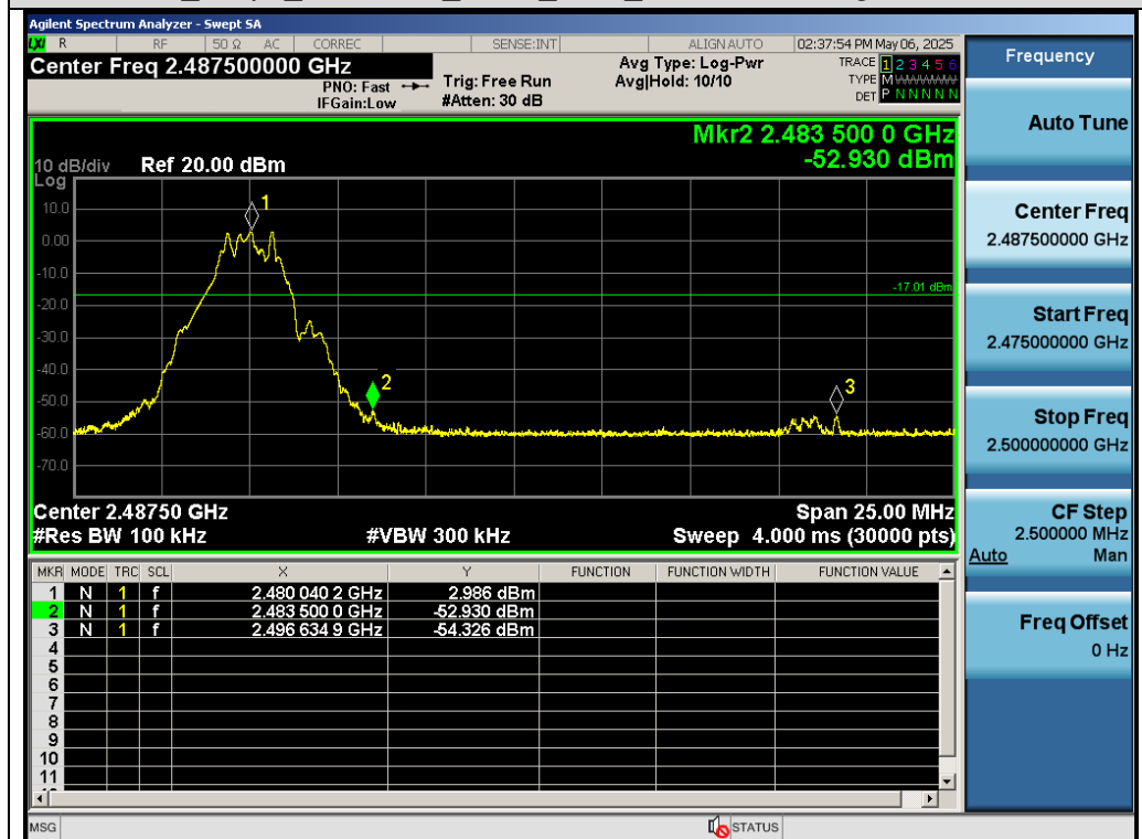
Test_Graph_SRD 2.4G_ANT1_2480_Higher Band Edge Emissions
