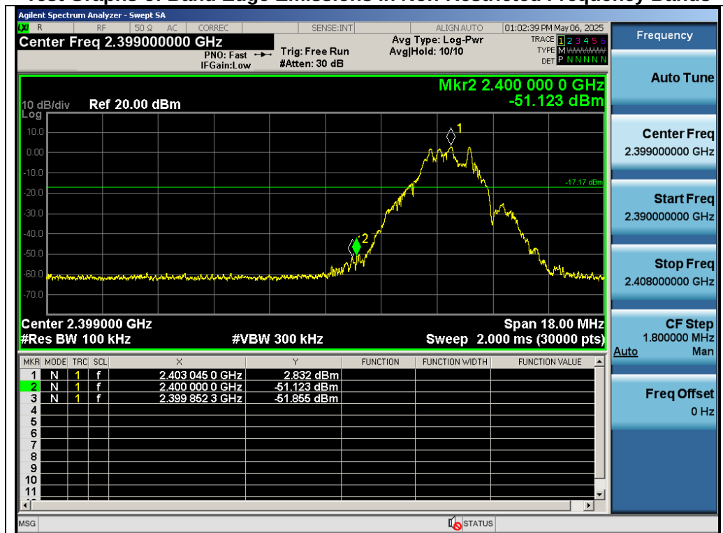
Test_Graph_SRD 2.4G_ANT1_2403_Lower Band Edge Emissions
