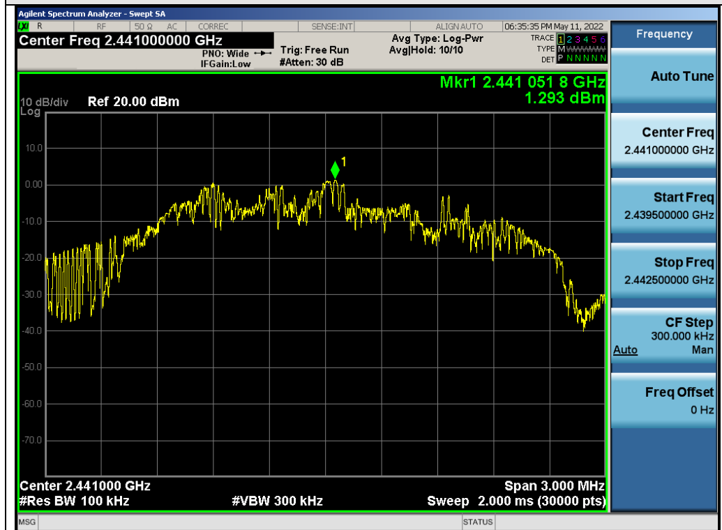
Test_Graph_2.4G_ANT1_2441_Reference Level
