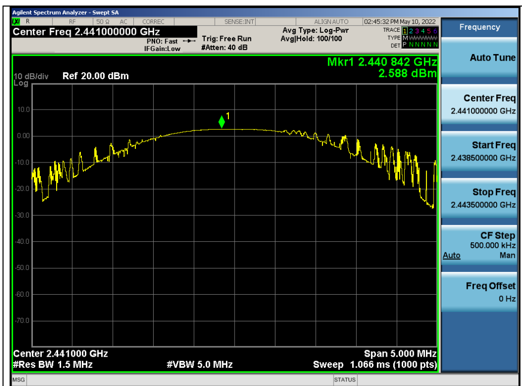
Test_Graph_2.4G_ANT1_2441_Peak Power
