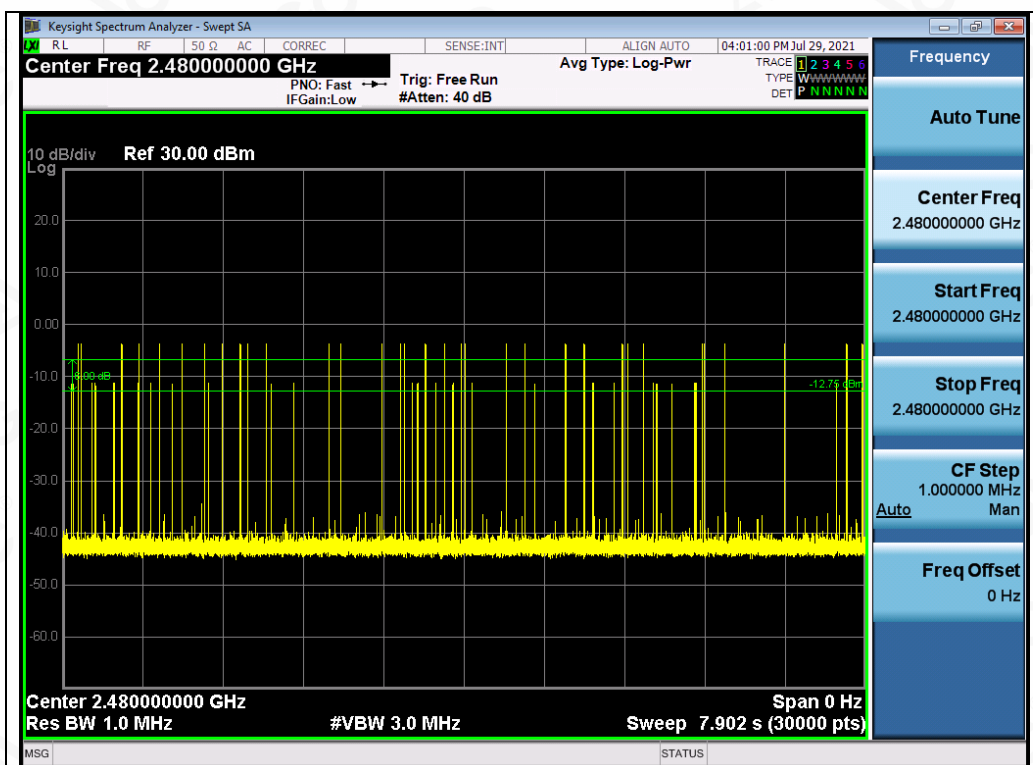
Test Graph BR HOP ANT1 NA 1Mbps 2480 Number of Burst
