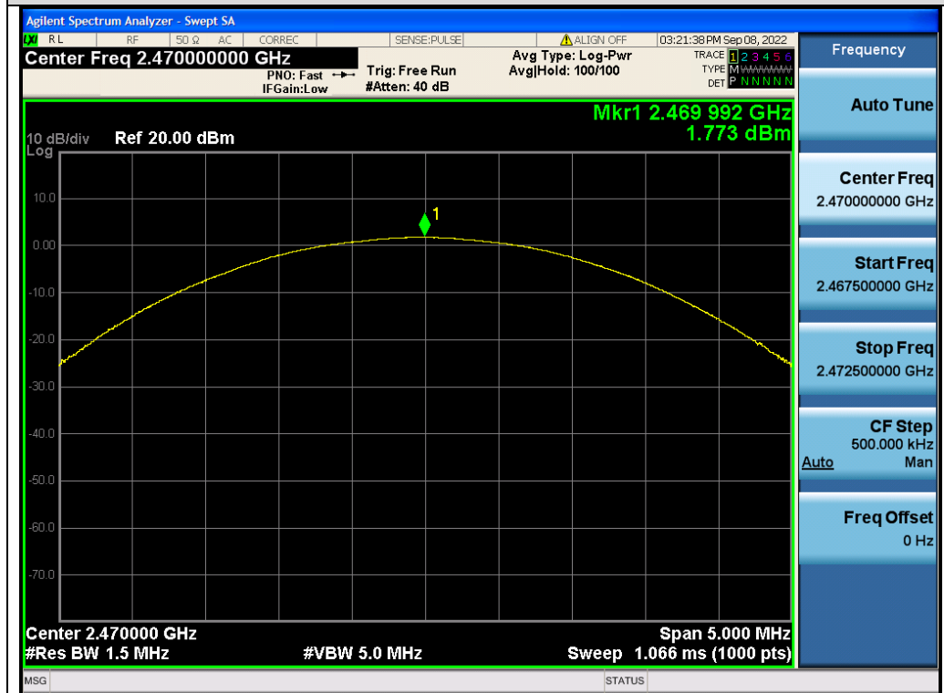
Test_Graph_GFSK_ANT1_2470_Peak Power
