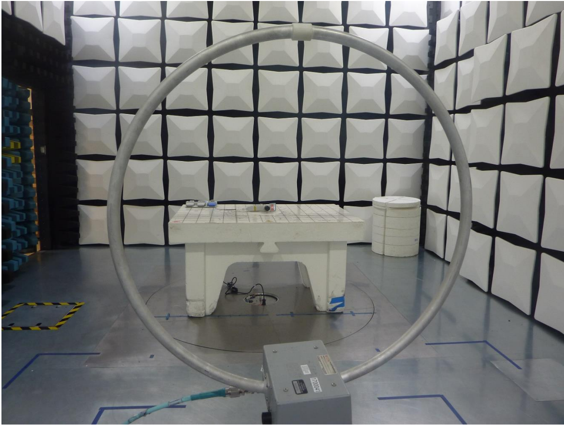
Figure 3: 9KHz-30MHz Radiated Emission Test Setup at 0 degree -Front View
