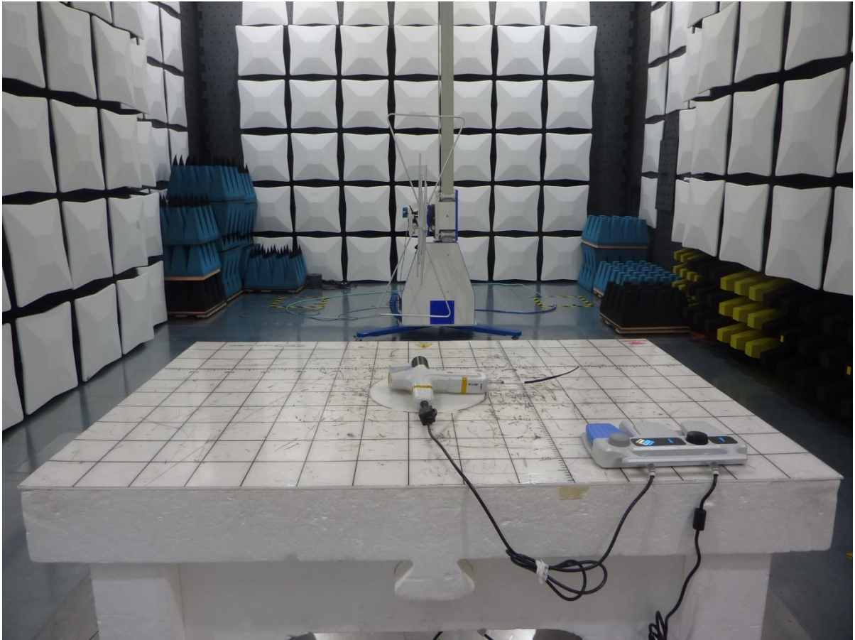
Figure 8: Test Setup for Radiated Emissions 30MHz to 1000MHz - Rear View
