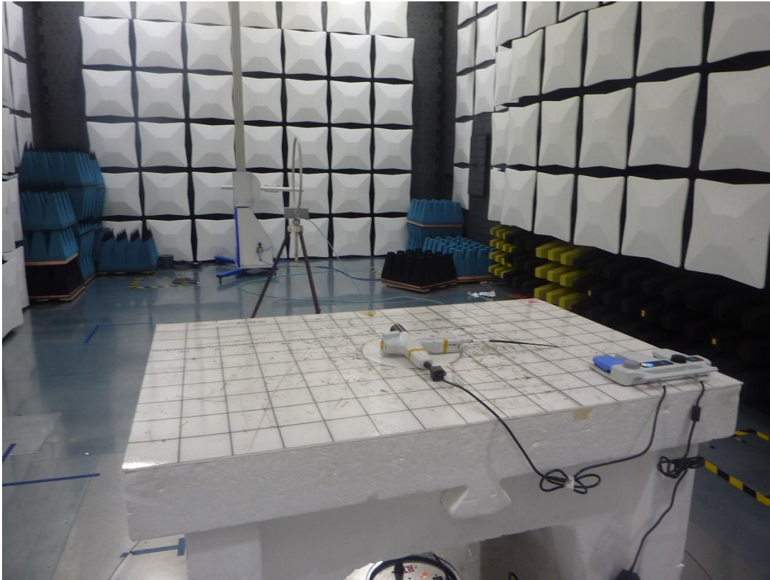
Figure 6: 9KHz-30MHz Radiated Emission Test Setup at 90 degree - Rear View
