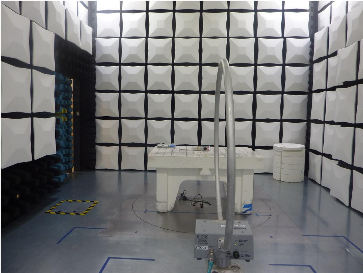
Figure 52: 9KHz-30MHz Radiated Emission Test Setup at 90 degree -Front View
