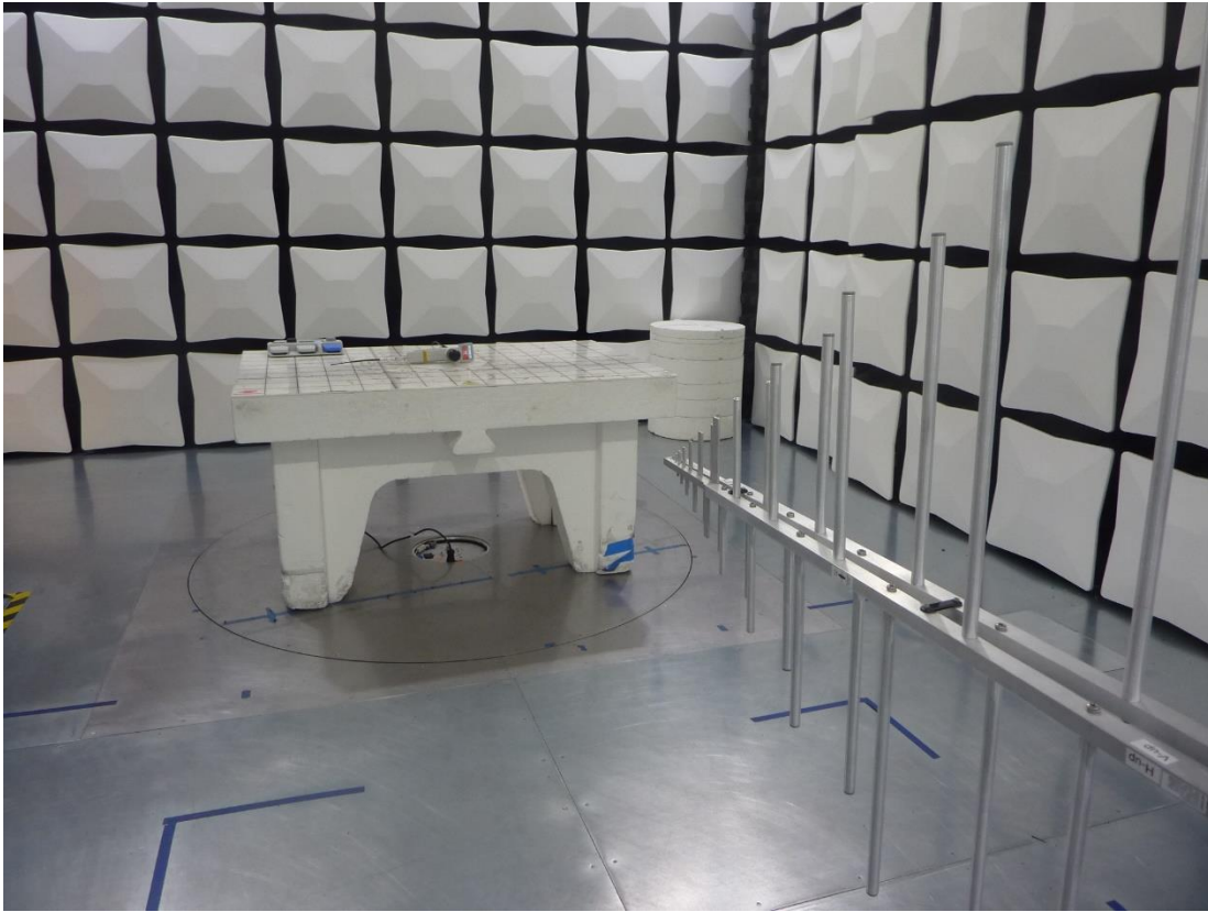
Figure 7: Test Setup for Radiated Emissions 30MHz to 1000MHz - Front View
