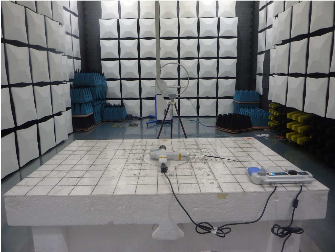
Figure 41: 9KHz-30MHz Radiated Emission Test Setup at 0 degree - Rear View
