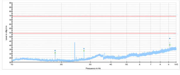
Figure 8.4-10: Radiated spurious emissions mid channel
