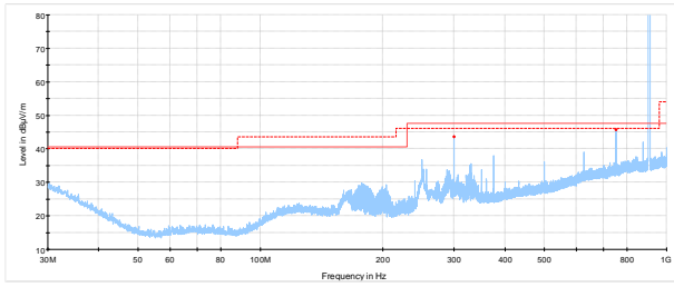
Figure 8.4-7: Radiated spurious emissions low channel
