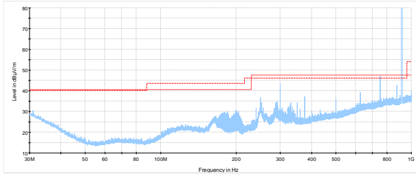
Figure 8.4-9: Radiated spurious emissions mid channel
