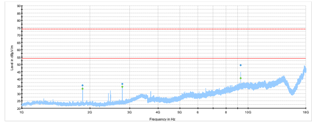
Figure 8.4-12: Radiated spurious emissions high channel
