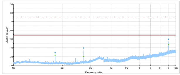
Figure 8.4-8: Radiated spurious emissions low channel
