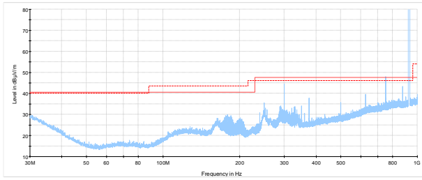
Figure 8.4-11: Radiated spurious emissions high channel
