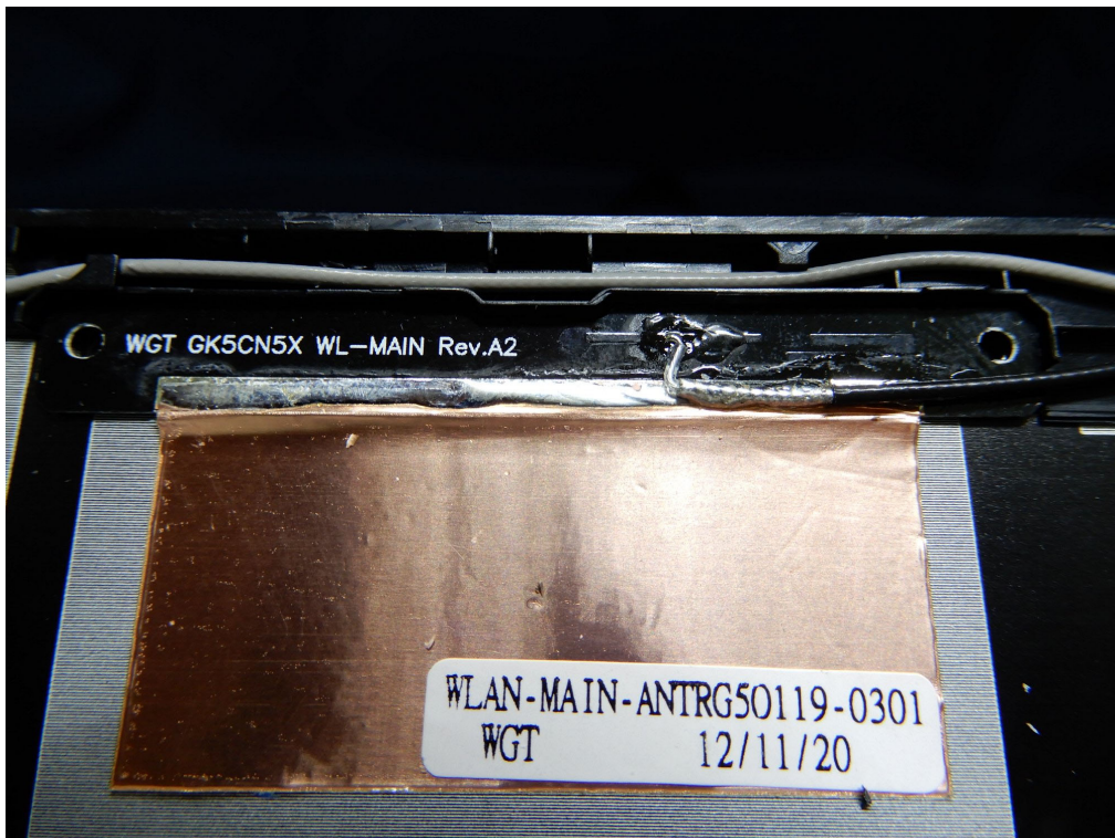
WGT Main Antenna Part No. ANTRG5W119-0301
