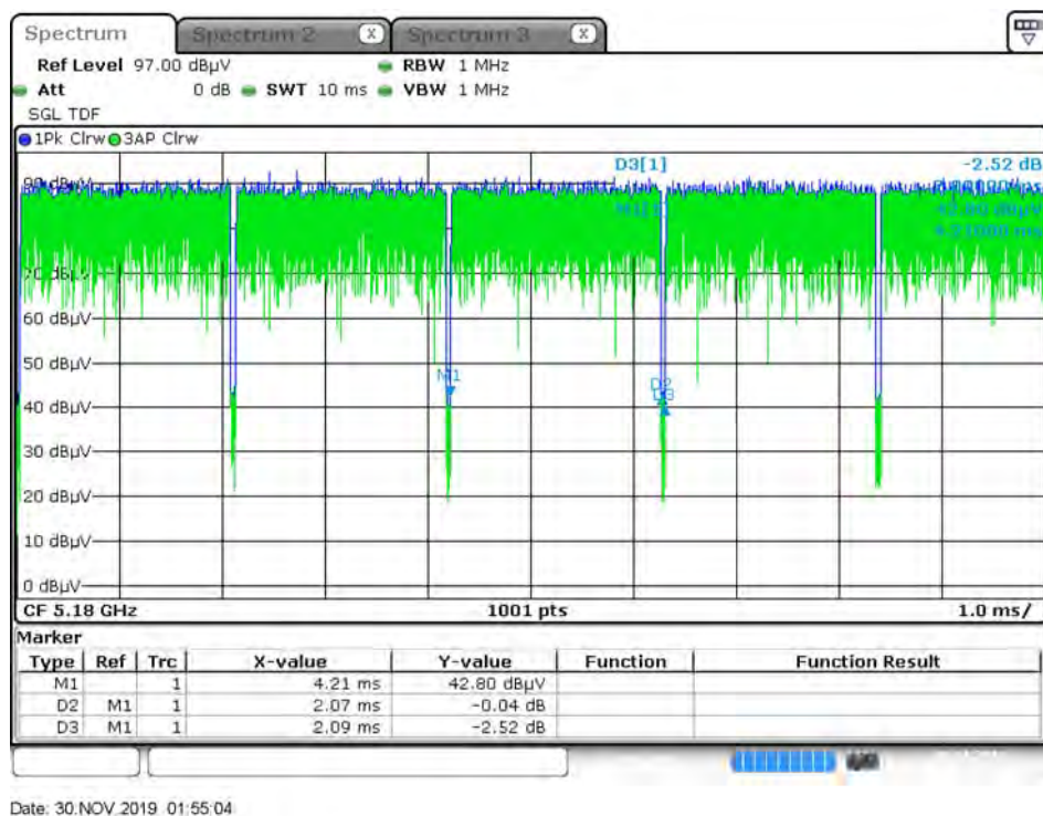
802.11a (SISO B)
