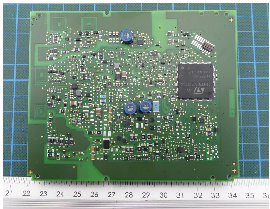
Board 1 – bottom view
