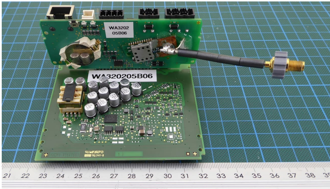
PCBs – front view
