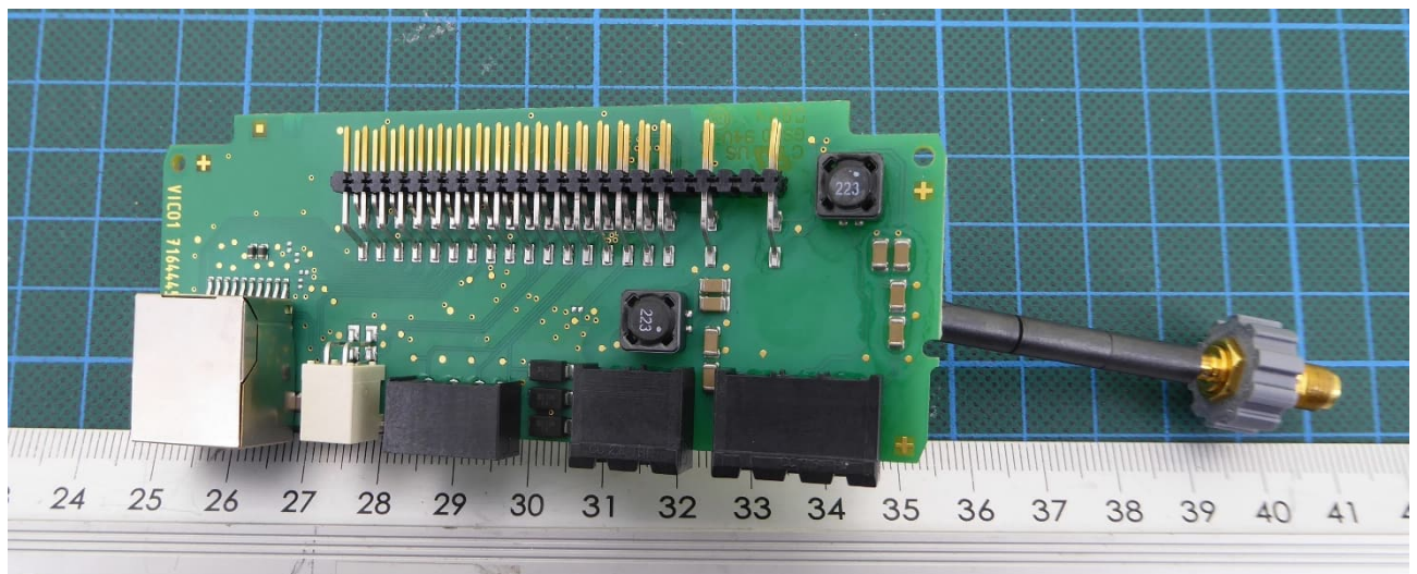
Board 2 – back view
