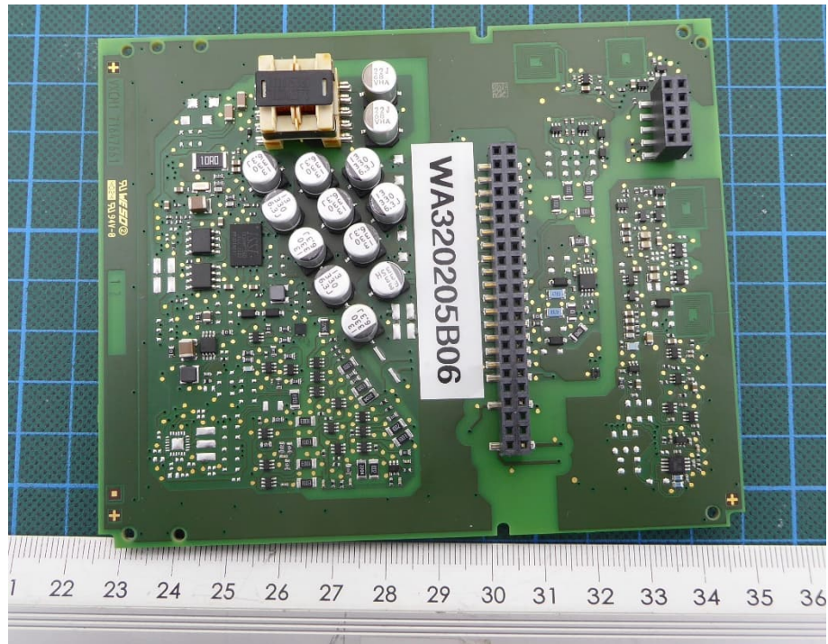
Board 1 – top view
