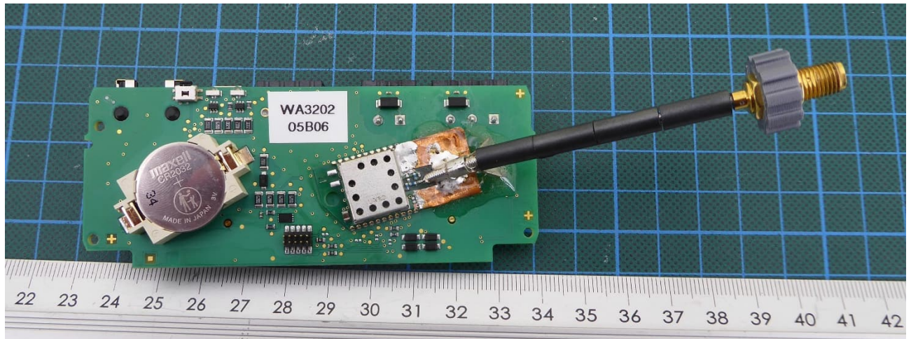
Board 2 – front view
