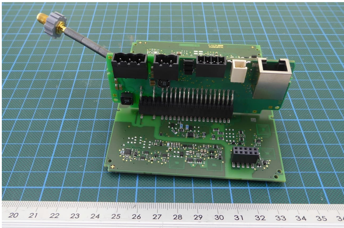
PCBs – back view
