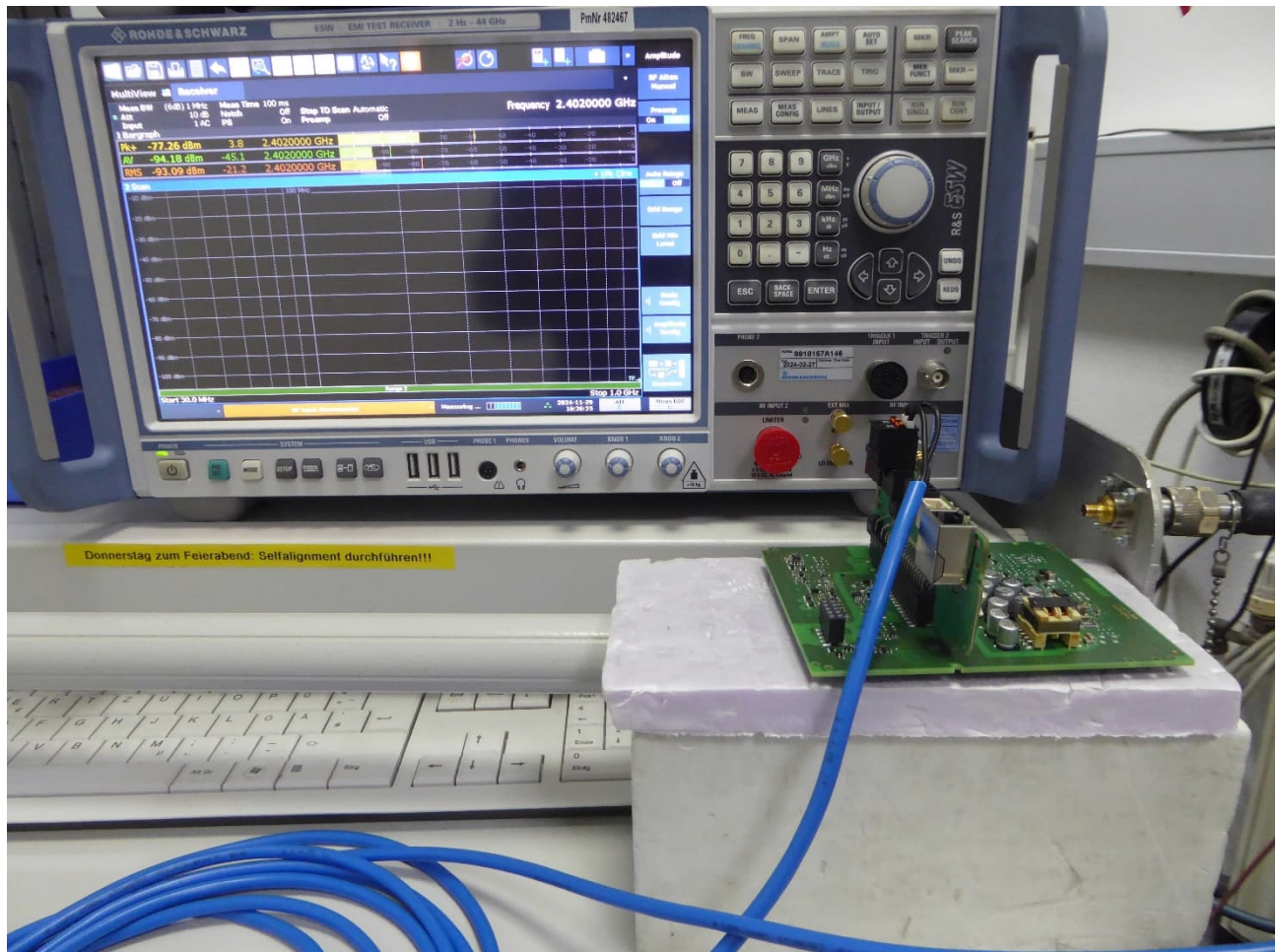
Setup antenna port conducted
