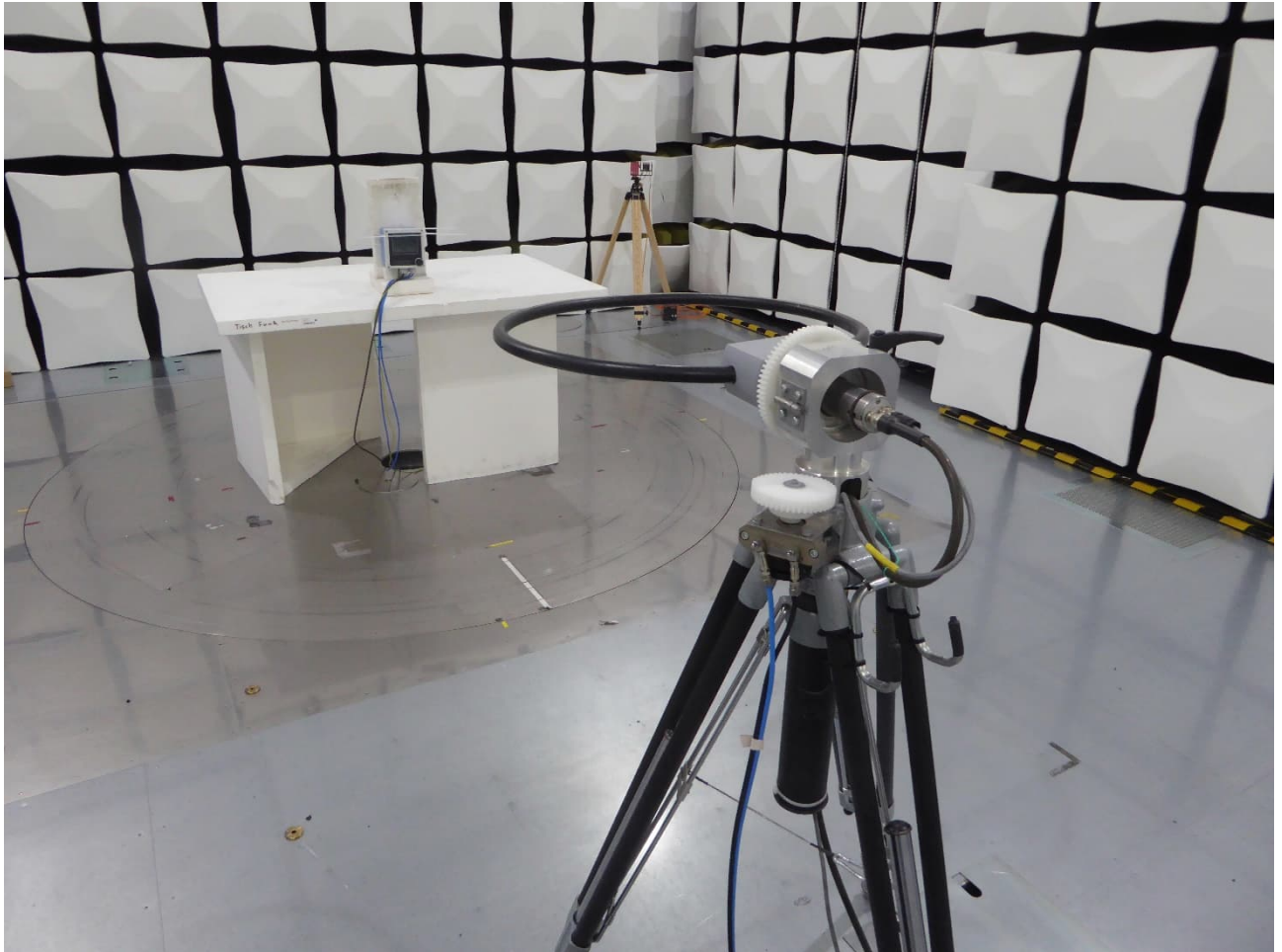
Antenna position 3, EUT position 1
