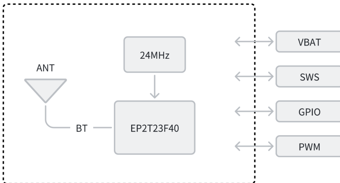
Fig 3-1 EWN-EP2T23F1CA System Block Diagram
