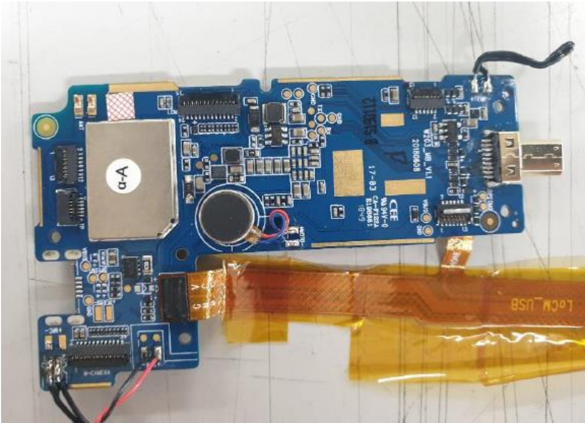
Display Board 1 (Front Side)
