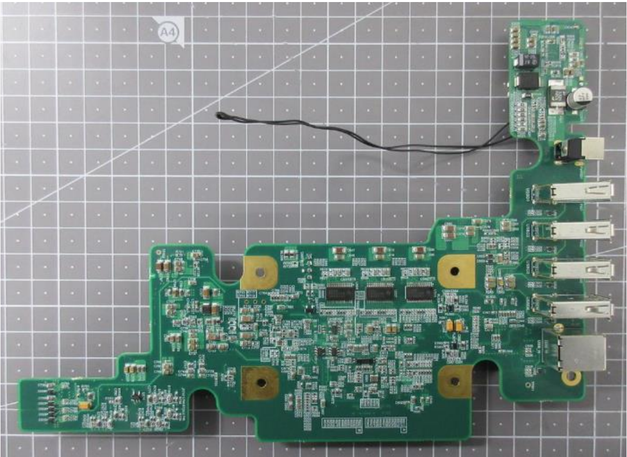
Main Board (Rear Side)
