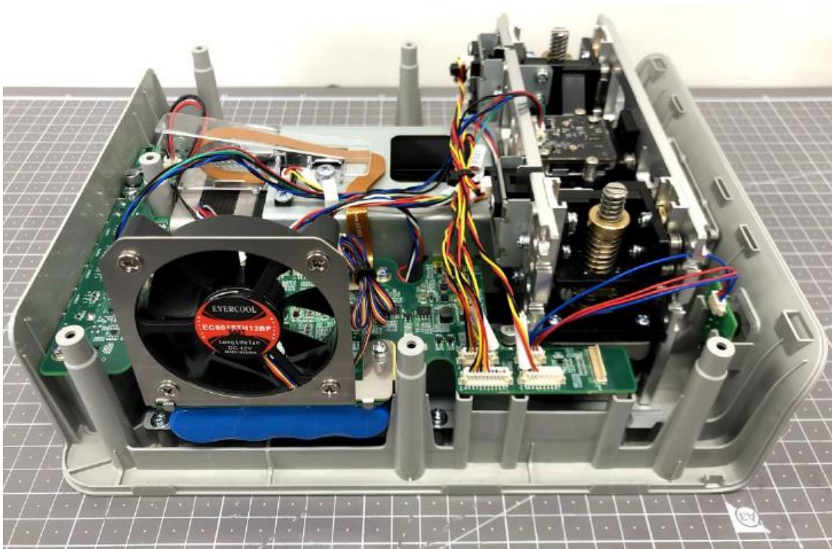
Side View
