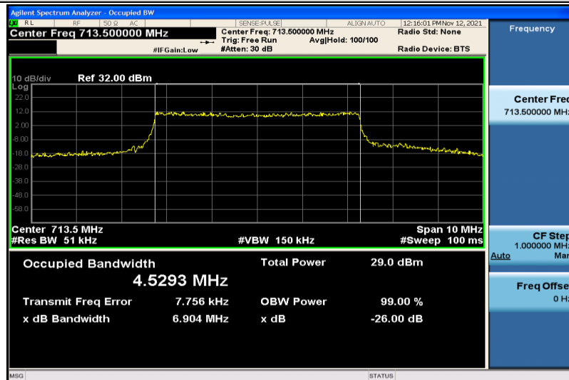
Band17-5MHz-QPSK-23825-25RB#0-4.5293
