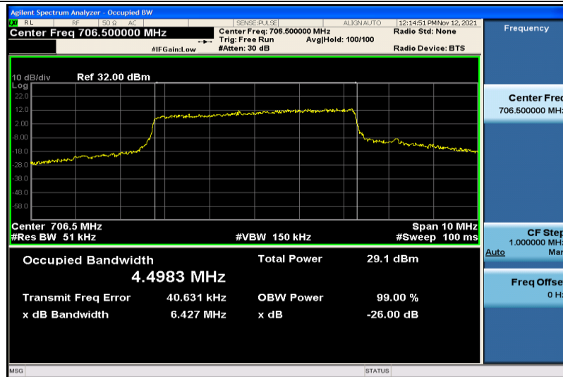
Band17-5MHz-QPSK-23755-25RB#0-4.4983
