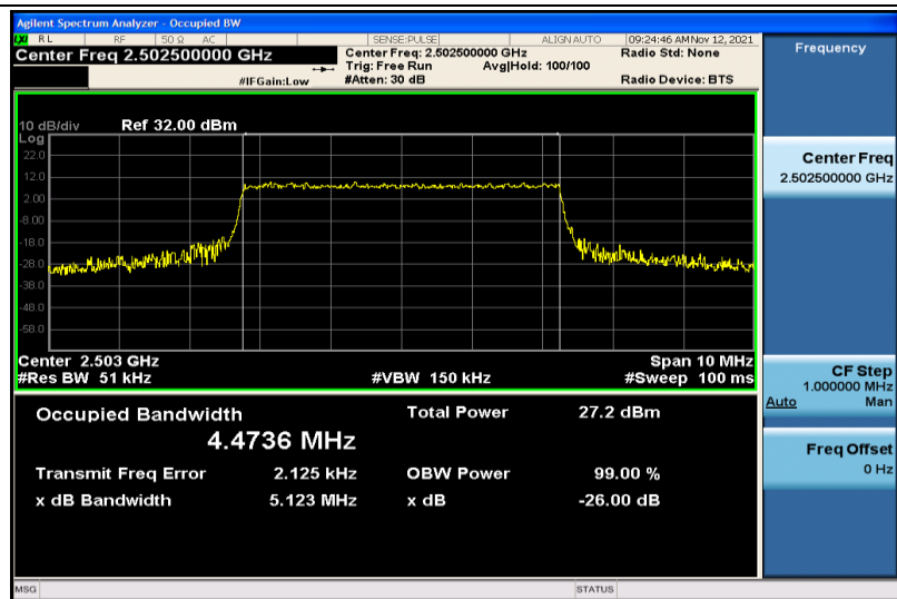
Band7-5MHz-16QAM-20775-25RB#0-4.4736
