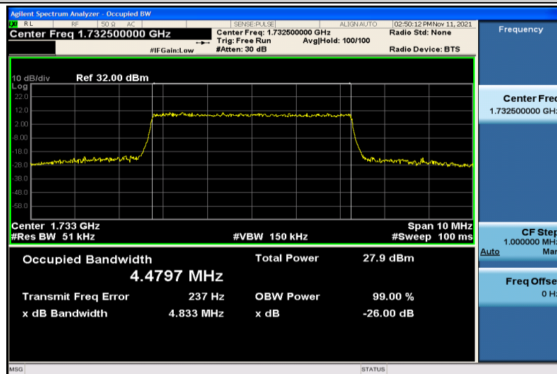
Band4-5MHz-16QAM-20175-25RB#0-4.4797
