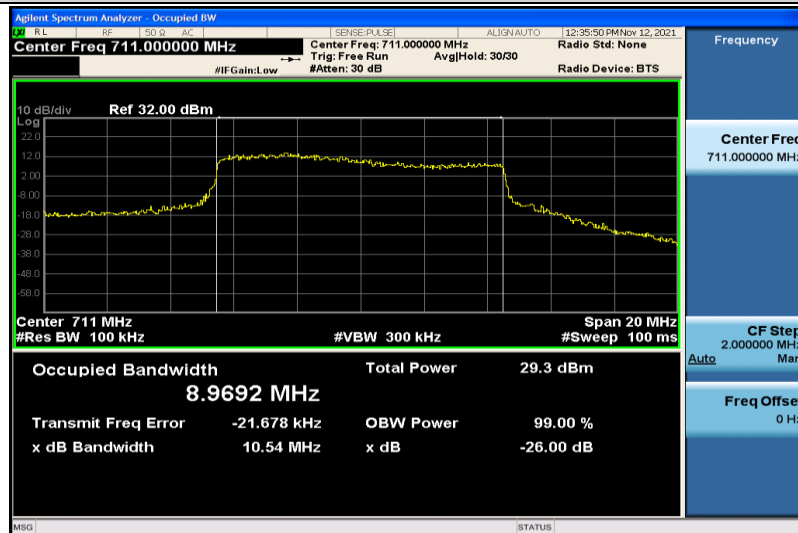
Band17-10MHz-QPSK-23800-50RB#0-8.9692
