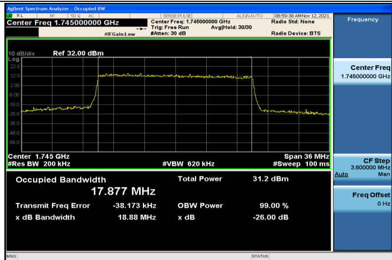
Band4-20MHz-QPSK-20300-100RB#0-17.877
