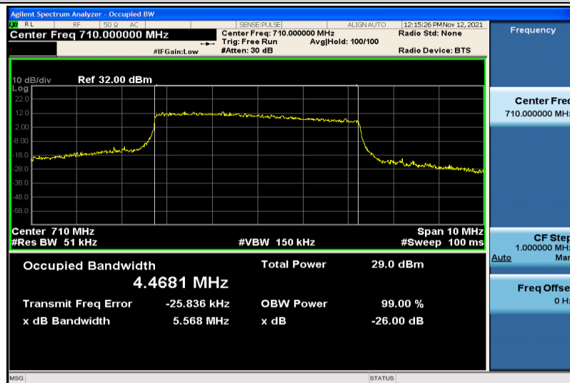
Band17-5MHz-QPSK-23790-25RB#0-4.4681
