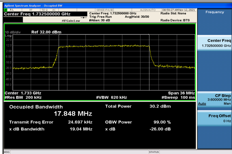
Band4-20MHz-16QAM-20175-100RB#0-17.848
