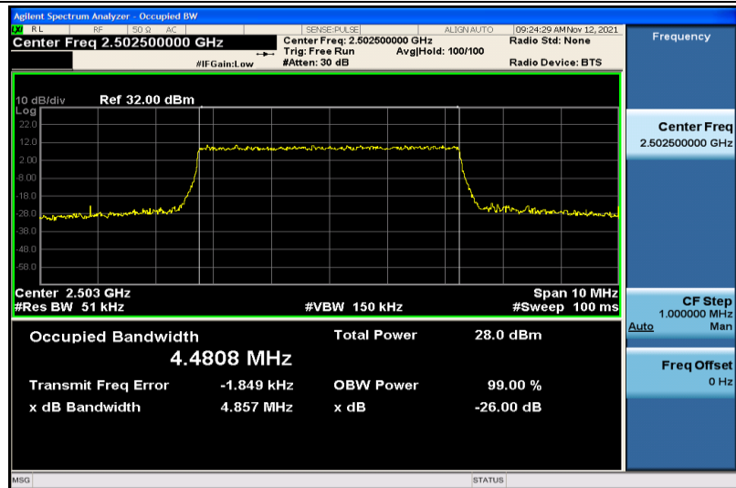
Band7-5MHz-QPSK-20775-25RB#0-4.4808
