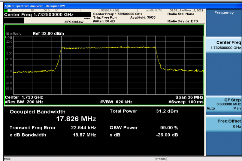
Band4-20MHz-QPSK-20175-100RB#0-17.826
