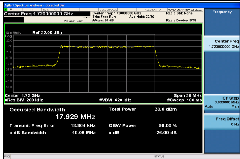
Band4-20MHz-16QAM-20050-100RB#0-17.929
