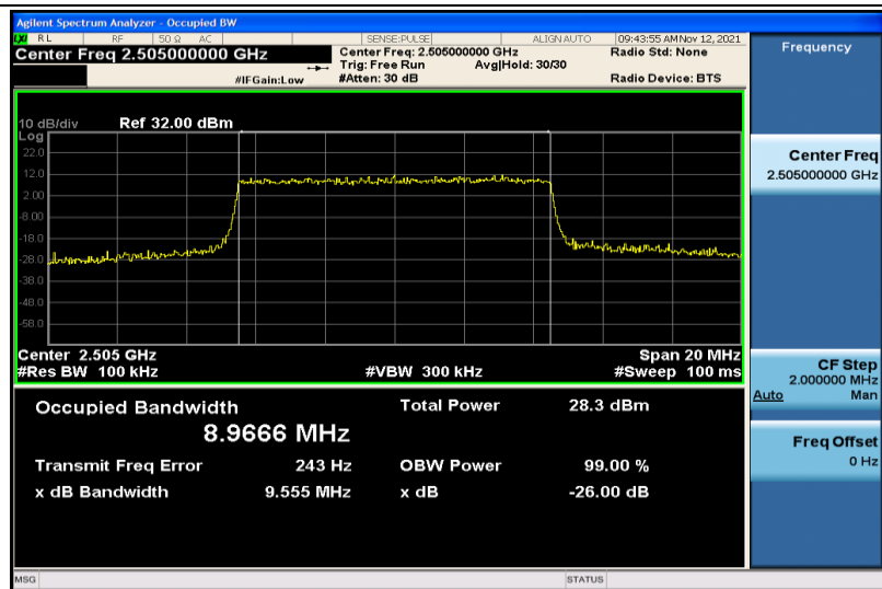
Band7-10MHz-QPSK-20800-50RB#0-8.9666
