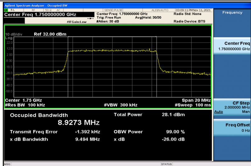
Band4-10MHz-16QAM-20350-50RB#0-8.9273
