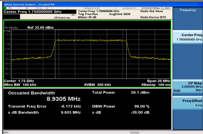
Band4-10MHz-QPSK-20350-50RB#0-8.9305
