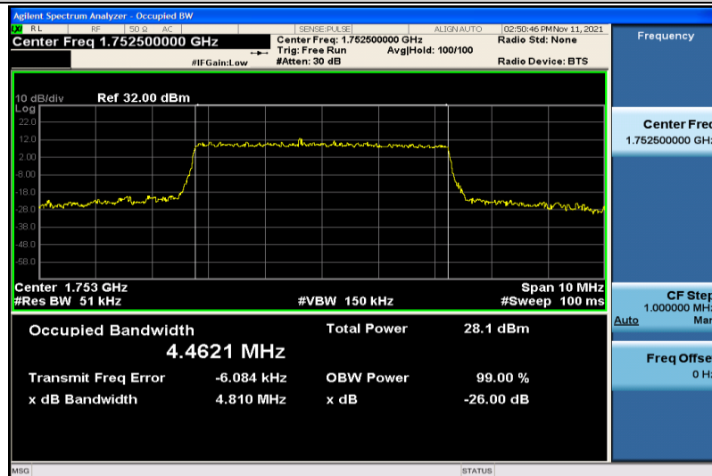
Band4-5MHz-16QAM-20375-25RB#0-4.4621
