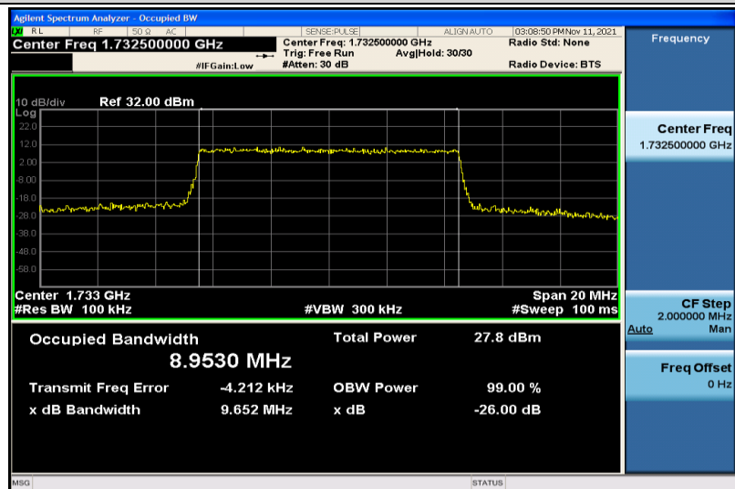
Band4-10MHz-16QAM-20175-50RB#0-8.9530
