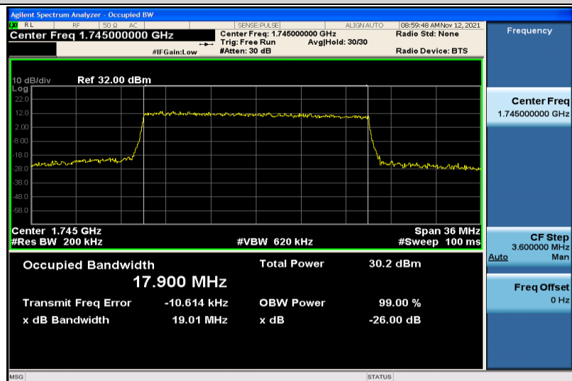
Band4-20MHz-16QAM-20300-100RB#0-17.900
