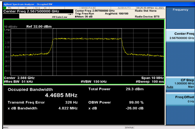
Band7-5MHz-QPSK-21425-25RB#0-4.4685
