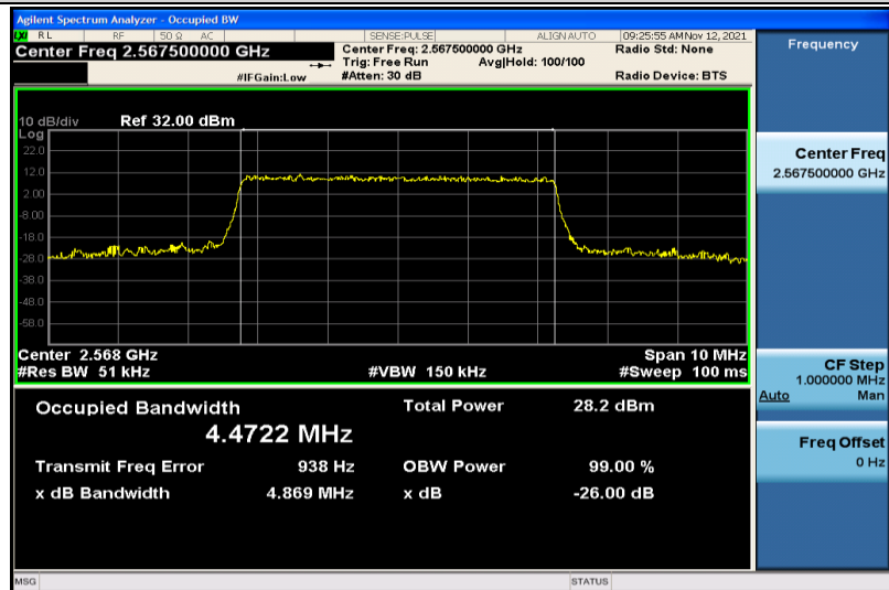
Band7-5MHz-16QAM-21425-25RB#0-4.4722
