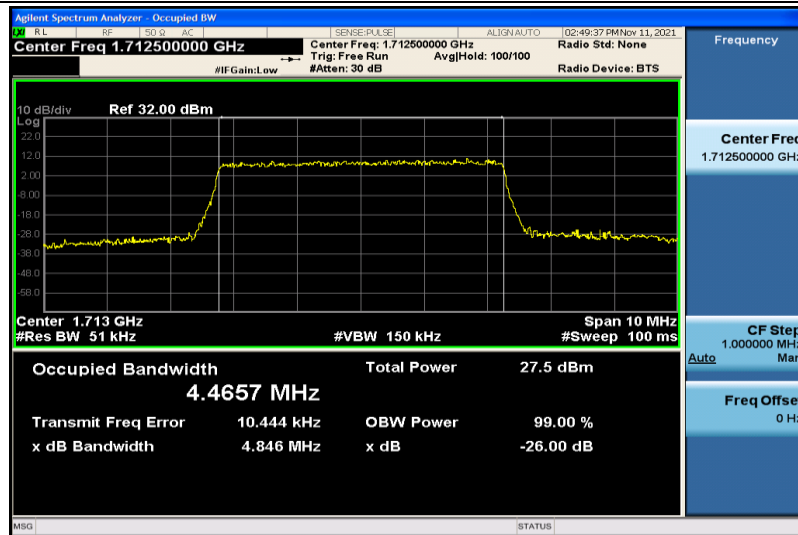
Band4-5MHz-16QAM-19975-25RB#0-4.4657
