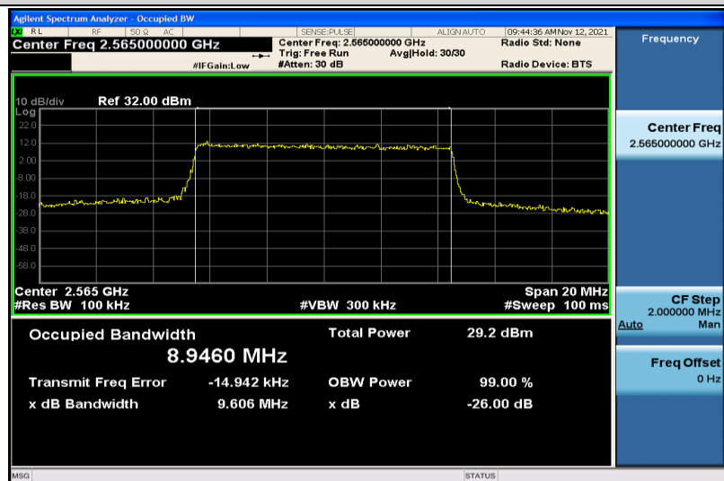
Band7-10MHz-QPSK-21400-50RB#0-8.9460
