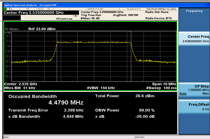
Band7-5MHz-QPSK-21100-25RB#0-4.4790
