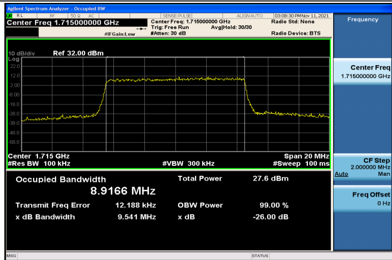
Band4-10MHz-16QAM-20000-50RB#0-8.9166
