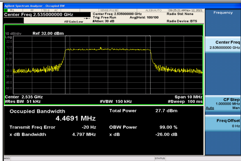
Band7-5MHz-16QAM-21100-25RB#0-4.4691
