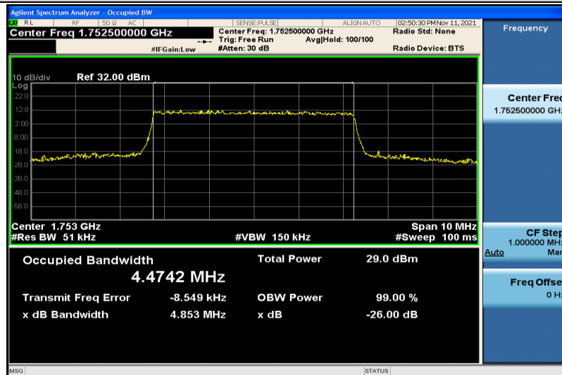
Band4-5MHz-QPSK-20375-25RB#0-4.4742
