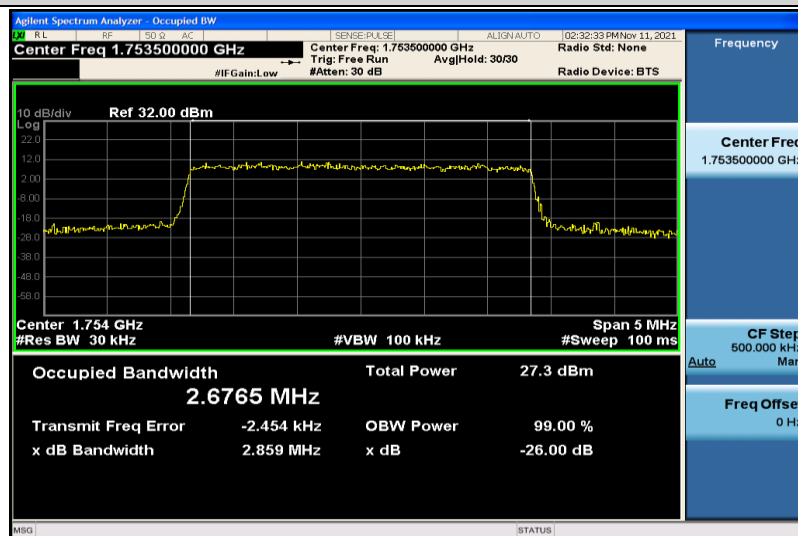
Band4-3MHz-16QAM-20385-15RB#0-2.6765
