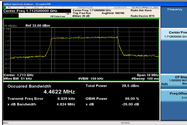
Band4-5MHz-QPSK-19975-25RB#0-4.4622
