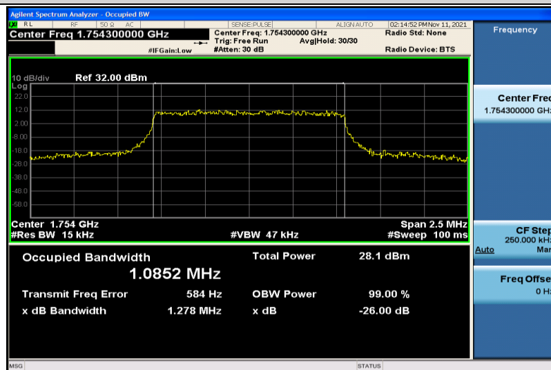
Band4-1.4MHz-QPSK-20393-6RB#0-1.0852
