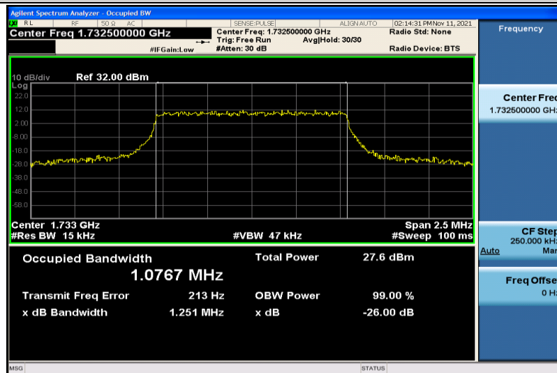
Band4-1.4MHz-QPSK-20175-6RB#0-1.0767
