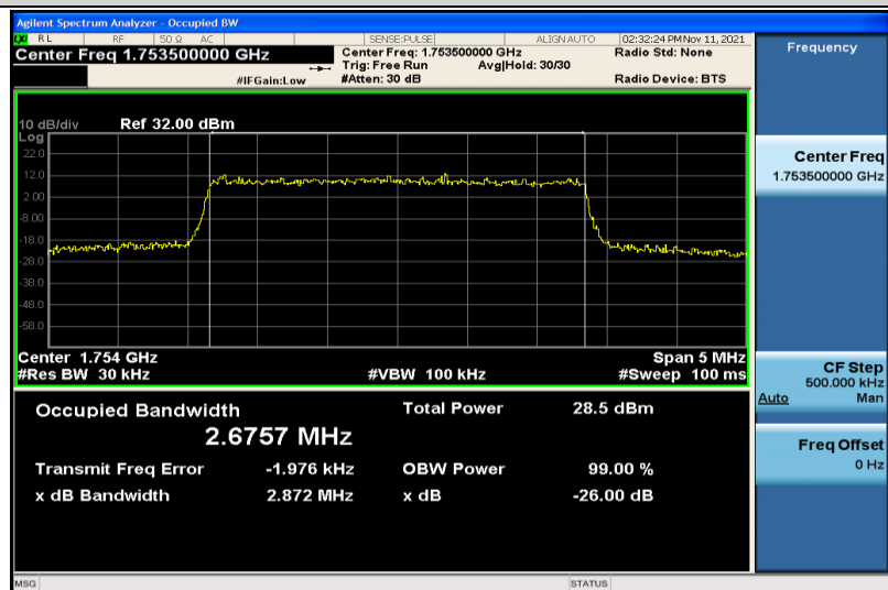
Band4-3MHz-QPSK-20385-15RB#0-2.6757
