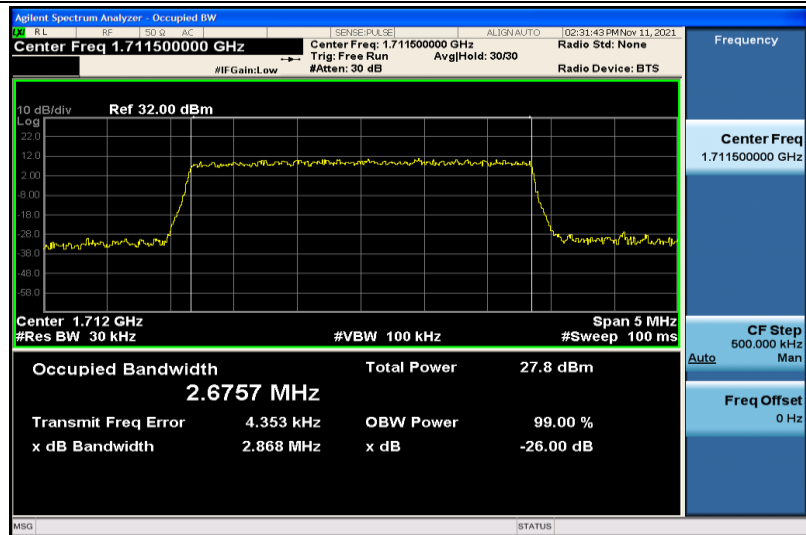
Band4-3MHz-QPSK-19965-15RB#0-2.6757
