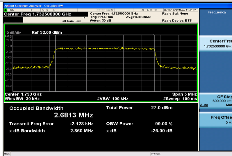
Band4-3MHz-16QAM-20175-15RB#0-2.6813
