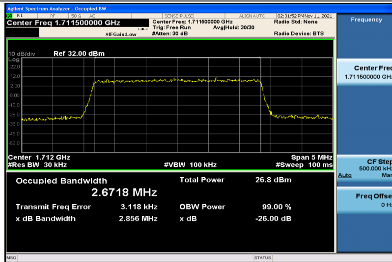
Band4-3MHz-16QAM-19965-15RB#0-2.6718
