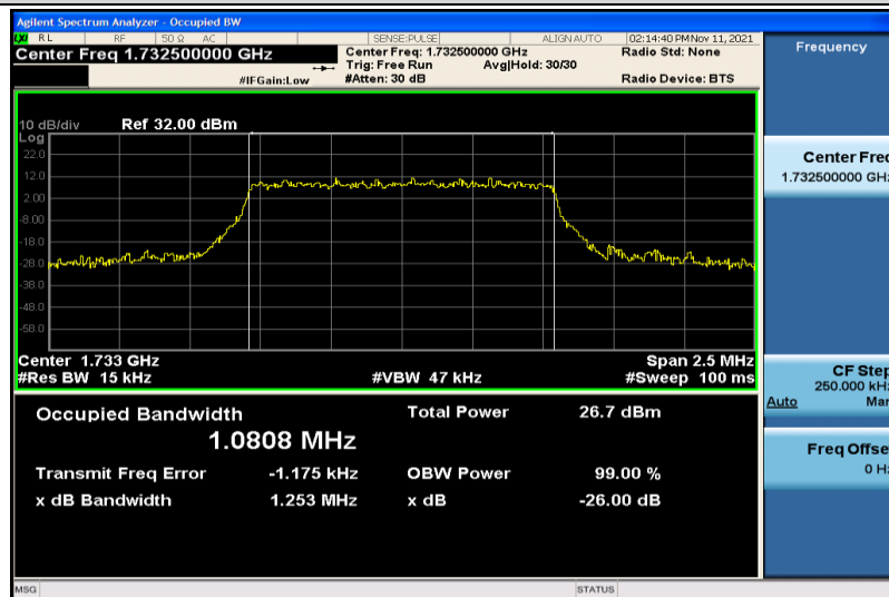
Band4-1.4MHz-16QAM-20175-6RB#0-1.0808
