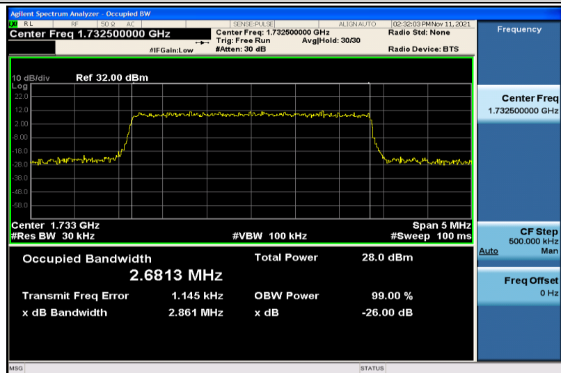
Band4-3MHz-QPSK-20175-15RB#0-2.6813
