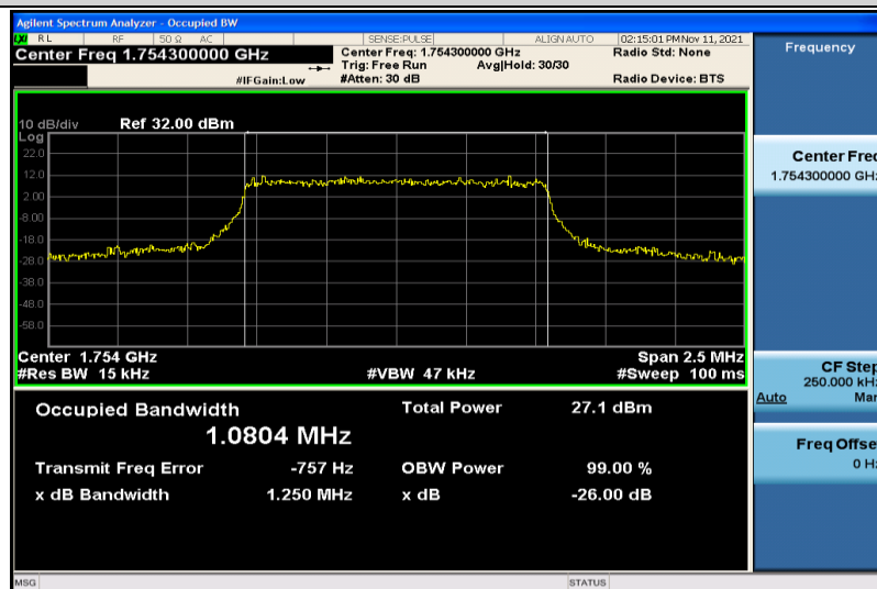
Band4-1.4MHz-16QAM-20393-6RB#0-1.0804
