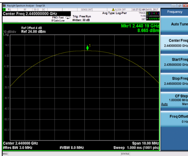
Output Power: 2440MHz
