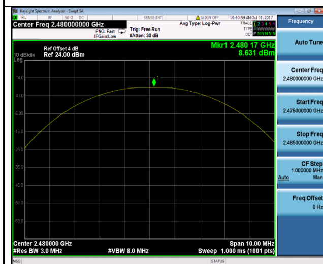
Output Power: 2480MHz
